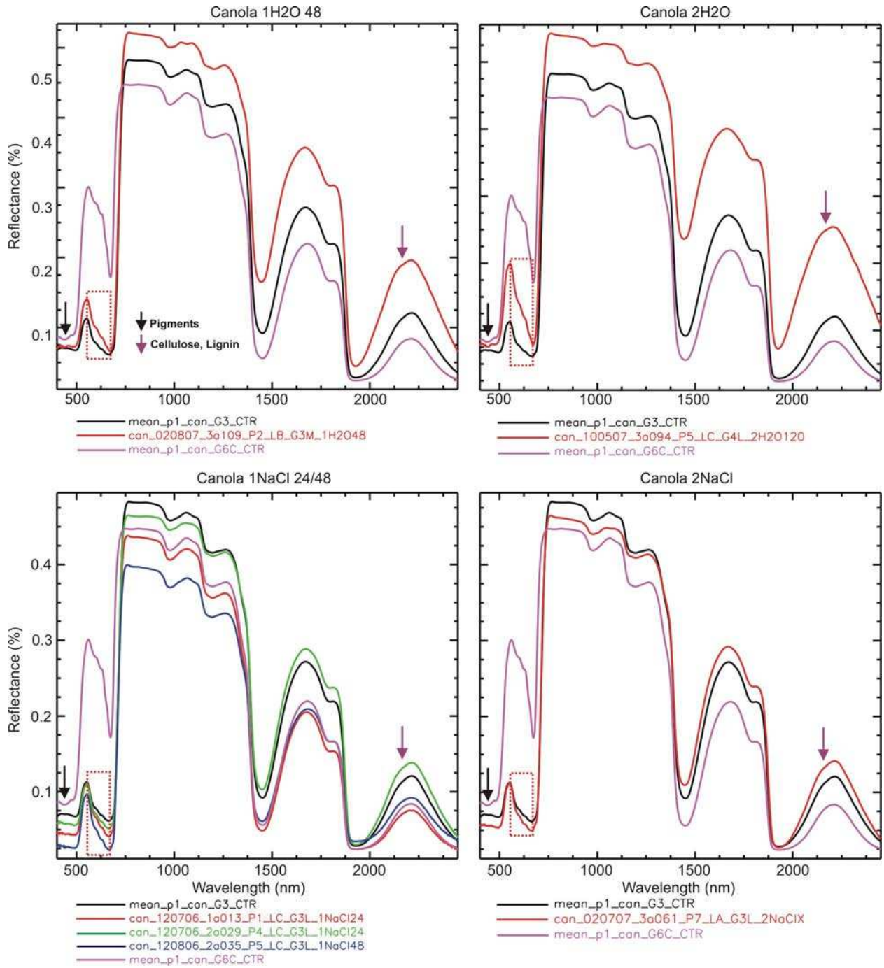
Figure 18. Endmember spectra for canola experiments H 2 O, NaCl, HCN, and NH 3 . Mean spectra of control G3 (black line, mature healthy) and G6C (pink line, high senescence) are included for reference. Arrows denote key absorption features observed in endmember spectra compared with G3. Red dotted box denotes an increased ratio between the green peak and chlorophyll trough.
