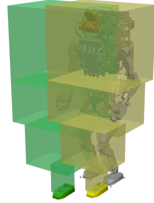
Fig. 4. Simplified bounding box model of the robot used to plan footstep locations that will be collision-free for the entire robot.
