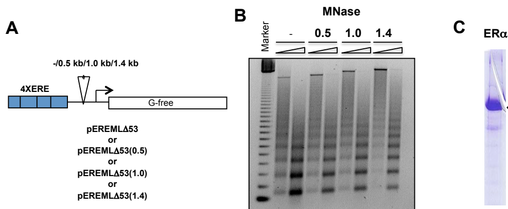
Fig. 1. Materials for ER \alpha -dependent activation from distal sites. (A) Schematic of templates: parent vector pEREMLA53 and its derivatives in which ERE is 0.5, 1.0, or 1.4 kb away from core promoter. (B) MNase analysis of chromatinized templates. (C) Preparation of ER \alpha following purification from baculovirus-infected Sf9 cells.
