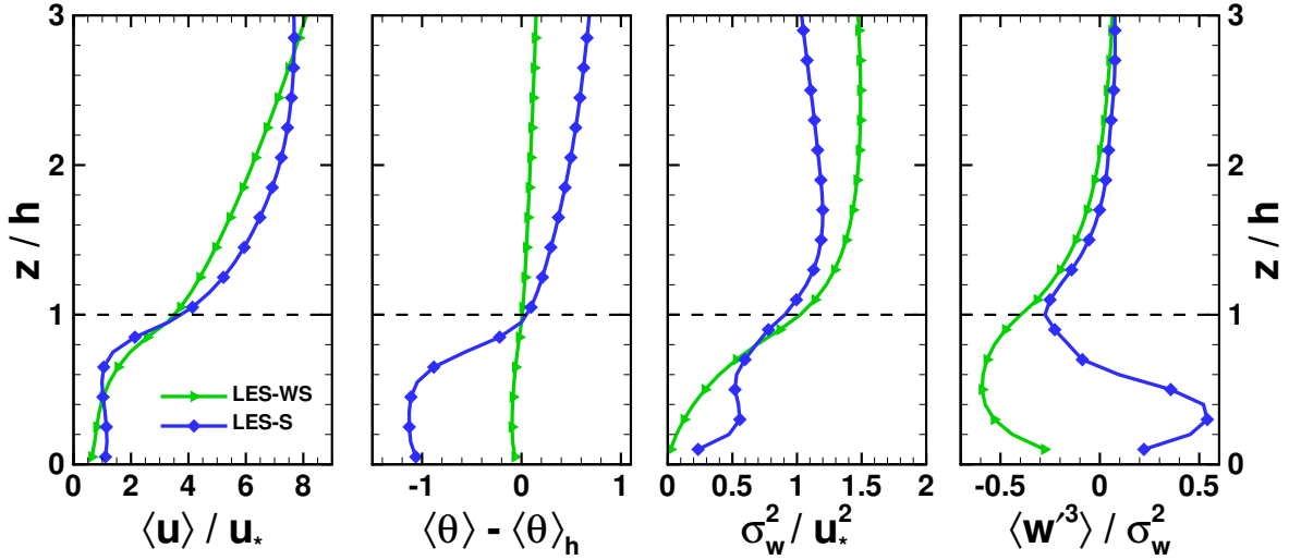
Figure 3: Horizontal- and time-averaged vertical profiles of the mean wind normalized by the friction velocity at canopy top \langle u \rangle / u_* (left), potential temperature minus the canopy-top potential temperature in Kelvin (middle-left), vertical velocity variance normalized by u_*^2 (middle-right), and vertical velocity skewness (right) from the coupled-canopy turbulence-resolving large eddy simulations mimicking the periods during CHATS when the dispersion experiments took place. The profiles are calculated from two nearly identical simulations that only vary in the geostrophic wind driving the flow; U_g = (8, 4) \text{ ms}^{-1} for cases (LES-WS, LES-S), respectively, where these geostrophic wind variations result in two different stability conditions: weakly stable (LES-WS) and stable (LES-S). Note that the axis-ranges differ slightly between Figures 2 and 3.
