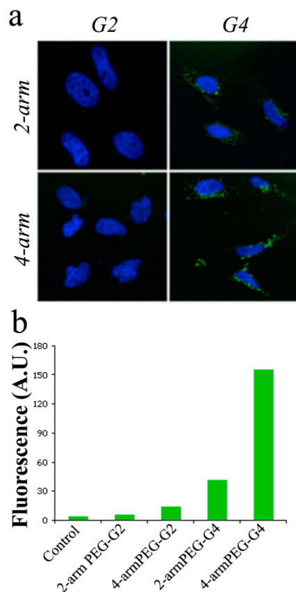
Figure 3. Cell binding and internalization. (a) Confocal imaging of HeLa cells treated with AF488-labeled dendrimers at 100 nM concentration (nuclei were visualized with Hoechst (blue)) and (b) membrane binding quantification of HeLa cells treated for 30 min with PEG-dendrimer hybrids.
