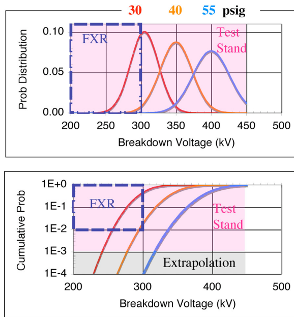
Figure 6. Hypothetical calculations show the effect of reducing gas pressure on pre-fire rates.
