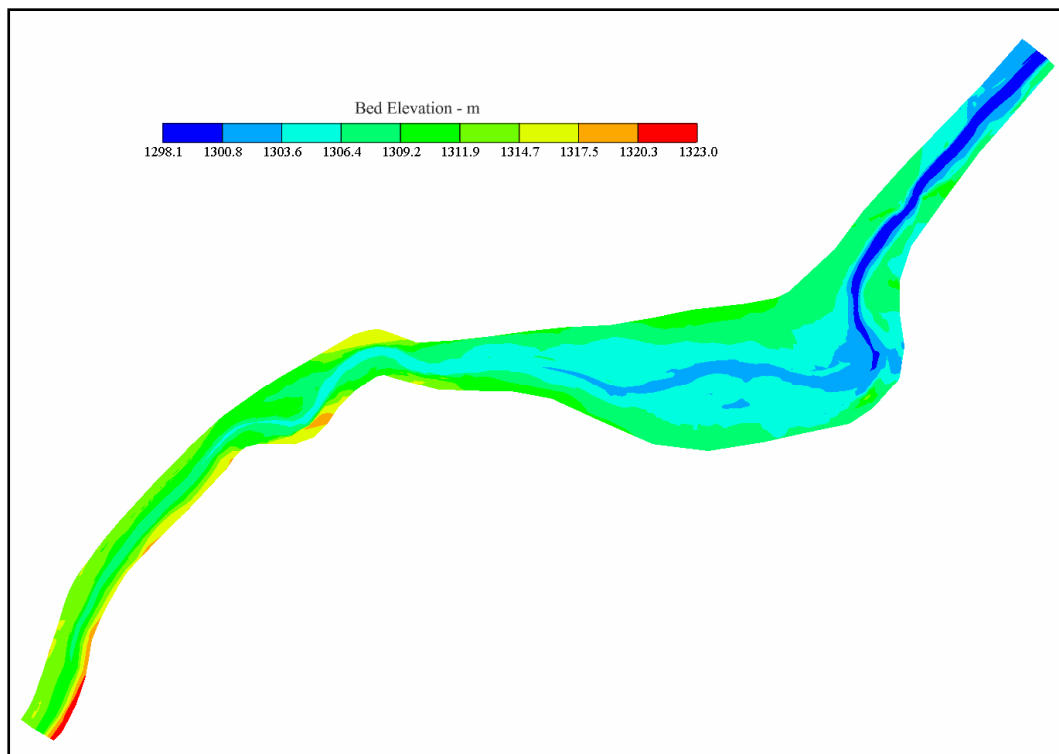
Figure 3. Model bathymetry
