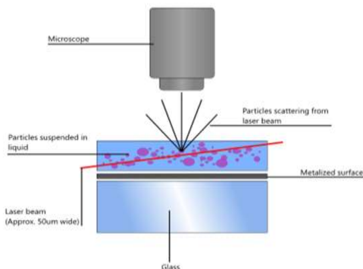
Figure 4: NANOSIGHT (Nanoparticle Tracking Analysis)
