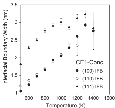
Fig. 5. The low-index, \gamma - \gamma' interfacial 10–90 widths, based on the composition profiles, as a function of temperature. The results are based on an overall cell composition of Ni-15Al (at.%) and CE1.
