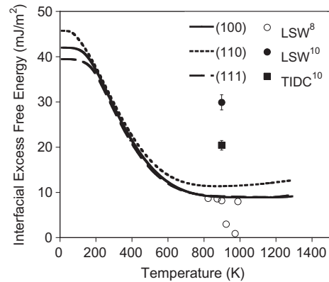
Fig. 11. The IEFE as a function of temperature for the (100), (110) and (111) \gamma\text{--}\gamma' boundaries calculated using CE2. The IEFE is derived by numerically integrating Eq. (1) using the piecewise continuous polynomial fit to the IEFE. The solid and dashed lines are the predicted IEFEs, and are in good agreement with IEFEs derived from earlier coarsening experiments of Ardell. Open and filled circles are from coarsening data fit to LSW theory [8] and the filled square is from fits using trans-interface-diffusion-controlled theory [10].
