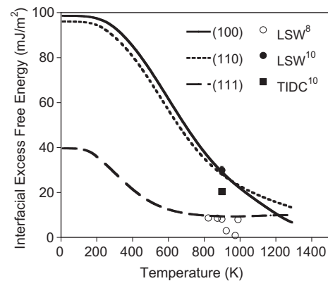
Fig. 8. The IEF E as a function of temperature for the (100), (110) and (111) \gamma - \gamma' boundaries calculated using CE1. The IEF E is derived by numerically integrating Eq. (1) using the piecewise continuous polynomial fit to the interfacial excess energy. The solid and dashed lines are the predicted IEF Es which are in good agreement with energies derived from earlier coarsening experiments of Ardell. Open and filled circles are from coarsening data fit to LSW theory [8] and the filled square is from fits using trans-interface-diffusion-controlled theory [10].
