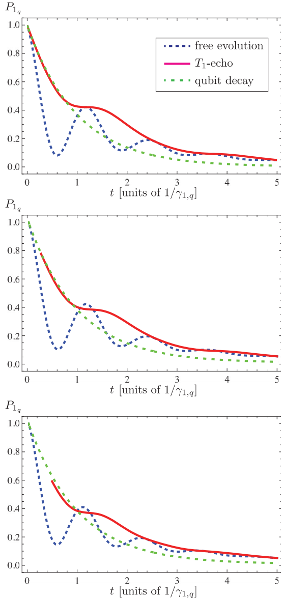
FIG. 6. (Color online) Time evolution of the qubit's excited-state population P_{1,q} as a function of time with (solid red) and without (dashed blue) application of the T_1 -echo sequence and for three different detunings between qubit and memory. The pulses are realized in this case using a detuned Hamiltonian evolution; see the text. The green dotted line shows again simple exponential decay with the rate \gamma_{1,q} . The red line does not start at the origin due to the finite pulse time 2t_\pi needed for application of the sequence. Parameters are (in units of \gamma_{1,q} ) \gamma_{\varphi,q} = 0.5 , \gamma_{1,m} = \gamma_{\varphi,m} = 0 , v_\perp = 5 , \delta\omega = 0 (top), 1 (middle), 2 (bottom).
