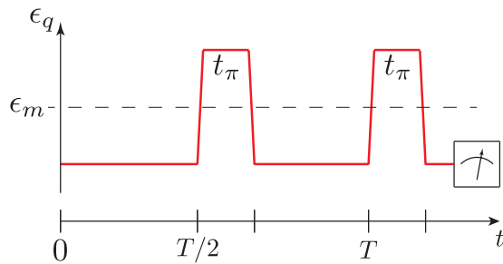
FIG. 4. (Color online) Illustration of the T_1 -echo sequence using only detuned Hamiltonian evolution. Both pulses \hat{U}_\perp and \hat{U}_R can be replaced by a period of detuned free evolution at detuning \delta\omega_1 = -v_\perp^2/\delta\omega for the time t_\pi . The red line depicts the qubit's level splitting at different times. The resonance condition with the memory, \epsilon_q = \epsilon_m , is indicated by the dashed line in the middle. The situation depicted corresponds to the case of initially \delta\omega = v_\perp where \delta\omega_1 = -\delta\omega .
