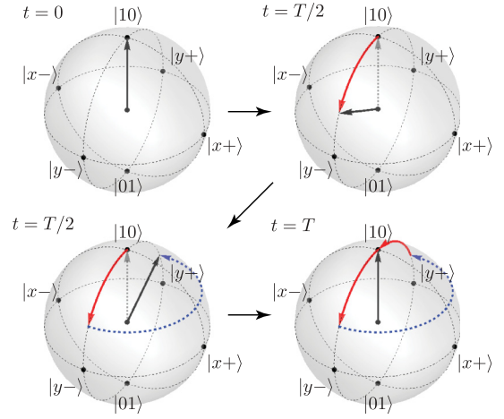
FIG. 2. (Color online) Step-by-step illustration of the T_1 -echo sequence on the effective one-excitation Bloch sphere for the resonance case \delta\omega = 0 , with a starting state |1_q, 0_m\rangle ; for details see the text. Red arrows show the path of the state vector during the two time spans of free evolution; the blue dashed arrow represents the path during the echo pulse \hat{U}_\perp . The recovery pulse is not shown, since for \delta\omega = 0 we have |\Psi_T\rangle = -i|\Psi_0\rangle . The illustration depicts a free-evolution time of T = 2\pi/(3\omega_0) . In this illustration we assume infinitely sharp pulses, i.e., no time is needed for the application of U_\perp .
