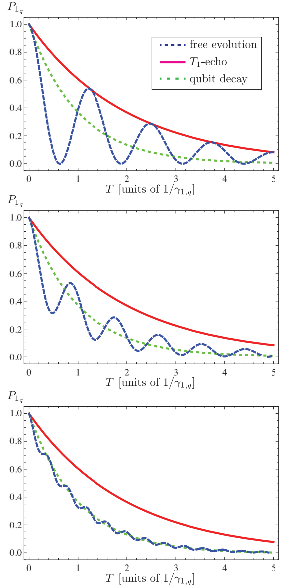
FIG. 5. (Color online) Time evolution of the qubit's excited-state population P_{1,q} as a function of free-evolution time T with (red solid) and without (blue dashed) application of the T_1 -echo sequence and for three different detunings between qubit and memory. The dotted green line shows the decay of the qubit itself without any interactions with other quantum systems. The pulses are assumed to be infinitely sharp in time, and there is relaxation acting on only the qubit, not the memory. Parameters are (in units of \gamma_{1,q} ) \gamma_{1,m} = \gamma_{\varphi,q} = \gamma_{\varphi,m} = 0 , v_\perp = 5 , \delta\omega = 0 (top), 5 (middle), 15 (bottom).
