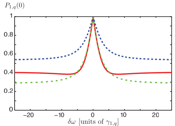
FIG. 7. (Color online) Initial decay of the qubit state vector due to the finite pulse length t_\pi obtained from numerical calculations. The red solid curve shows the probability of finding the qubit in its excited state as a function of detuning \delta\omega , after only the pulses have been applied to the system via the detuned Hamiltonian evolution. The total time that has passed is thus 2t_\pi , while no free evolution has taken place, so the free-evolution time T is zero. The green dotted curve for comparison shows the value of e^{-\gamma_{1,q}2t_\pi} , meaning the value of qubit excitation probability after application of the pulses without any influence of the TLS. The blue dashed line finally shows decay with the composite rate \gamma_+ . One can see that for small initial detuning, the pulses lead to decay dominated by the qubit rate, while for stronger initial detuning it crosses over to decay of the coupled systems. Parameter values are (in units of \gamma_{1,q} ) \gamma_{\varphi,q} = 0.5 , \gamma_{1,m} = \gamma_{\varphi,m} = 0 , v_\perp = 5 .
