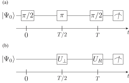
FIG. 1. Schematic representation of the pulse sequence for (a) standard spin-echo sequence and (b) the proposed T_1 -echo sequence. In both cases, the state of the qubit is read out after time T . Also in both cases, the application of echo and recovery pulses leads to a final state which is independent of T . For details, see the text.
