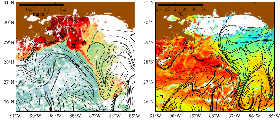
Figure 1. (left) Chlorophyll a concentration in the northern Gulf of Mexico on 12 July 2012 derived from the MODIS (Moderate Resolution Imaging Spectroradiometer) sensor aboard satellite Aqua with deployment sites in the two GLAD drifter groups considered indicated (triangles) and altimetric attracting LCS computed as 30 day backward squeezelines overlaid (black curves). (right) Sea surface temperature on 28 July 2012 derived from Advanced Very High Resolution Radiometer (AVHRR/3) sensor aboard satellite NOAA-19 with LCS overlaid.
