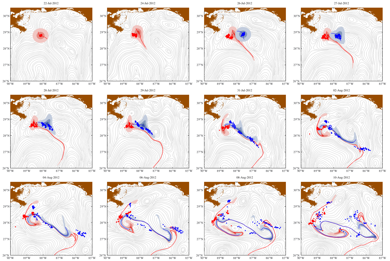
Figure 2. Sequence of selected snapshots of the evolution of fluid patches as advected by the altimetry-derived velocity field (4) (red and blue areas) and corresponding centerpieces or attracting LCS obtained as the advected images of forward stretchlines through the patches at the initial time (red and blue curves). Also indicated are S1 (red dots), S2 (blue dots) drifter positions, and instantaneous streamlines of the altimetry-derived velocity field (gray curves).
