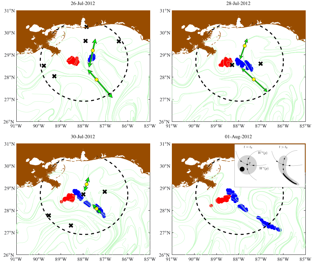
Figure 3. Altimetric LCS cores found within the circular domain delimited by the dashed line (yellow dots with green arrows attached); S1 (red dots) and S2 (blue dots) drifter positions; altimetric LCS computed as backward squeeze-lines (light green curves); and instantaneous saddle points of the altimetry-derived velocity field (black crosses). The inset in the lower right panel illustrates the effect of a saddle point on a material patch in steady flow. The saddle point, denoted p , is the counterpart of LCS core and the stable [respectively., unstable] manifold, denoted W^s(p) [respectively, W^u(p) ], is the counterpart of repelling [respectively, attracting] LCS.
