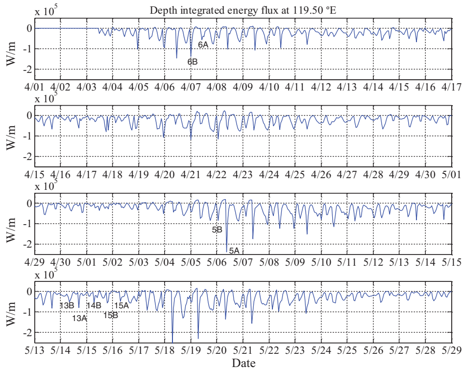
Figure 5. Same as in Figure 3 except for the depth-integrated energy flux over the entire water column.
