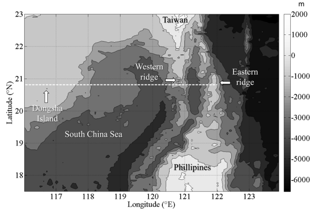
Figure 1. Map of the northern South China Sea showing the locations of the Dongsha Island and two ridges in the Luzon Strait. The latitude 20.81^{\circ}\text{N} is along the dashed line. The depth contour is in meters with a contour interval of 1000 m.
