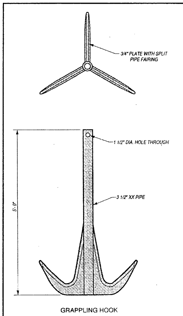
Figure 4. Grappling hook (To convert inches to centimeters, multiply by 2.54)
