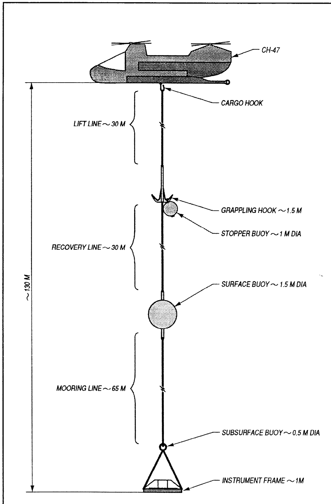
Figure 1. System suspended while in flight
