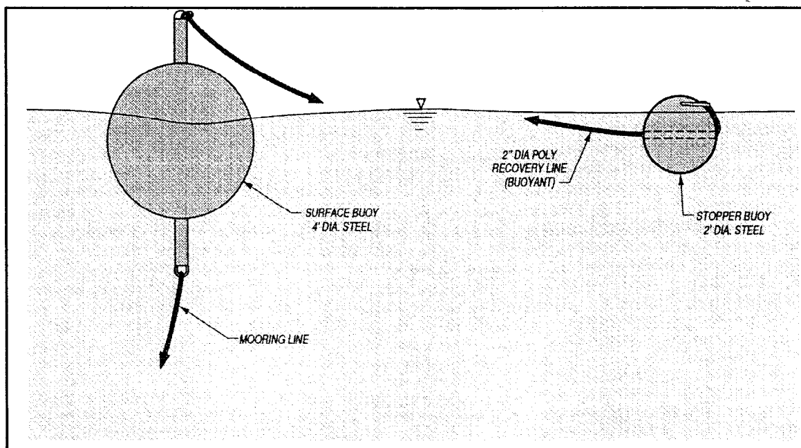
Figure 3. Surface buoy and stopper buoy (To convert inches to centimeters, multiply by 2.54)
