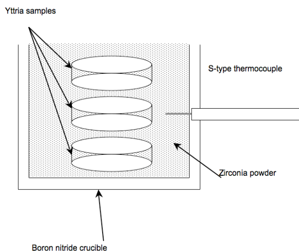
Figure 3. Small open casket used for sintering 6 mm diameter compacts
