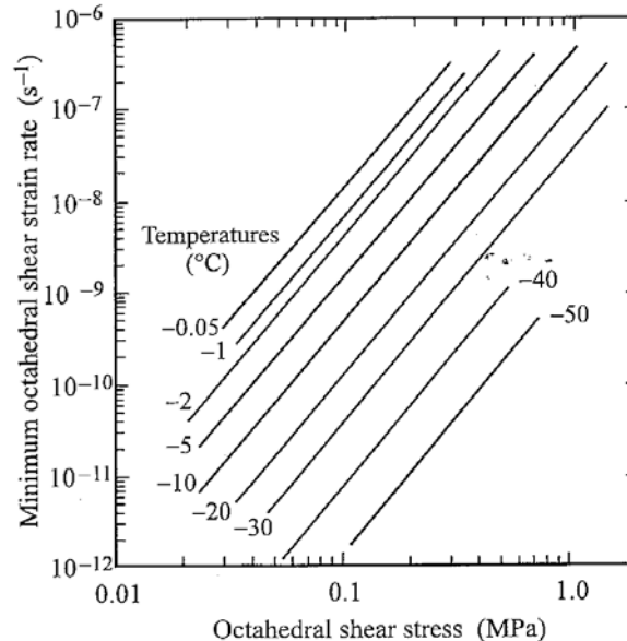
Figure 23. Minimum strain rate of polycrystalline ice in uniaxial creep. The variation in ice response as a function of ice temperature is illustrated by the family of curves (Budd and Jacka 1989).
