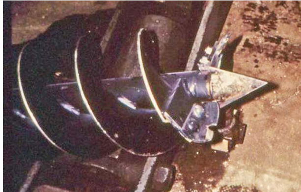
Figure 20. A modified auger bit used for cutting in ice (Haehnel 1998). The auger shown has a 30 cm (12 in.) diameter.
