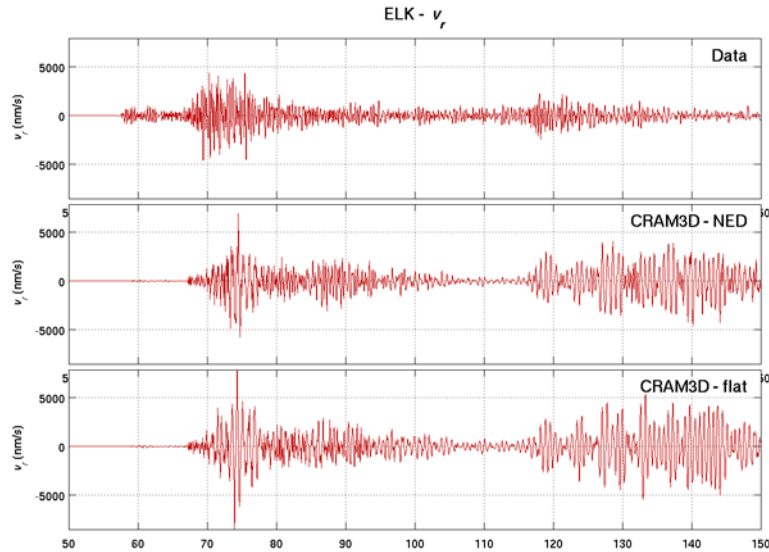
Figure 11. Calculated and observed waveforms from the NPE at station ELK at a distance of 400 km. Top: Observed; Middle: calculated with topography; Bottom: calculated with flat topography.
