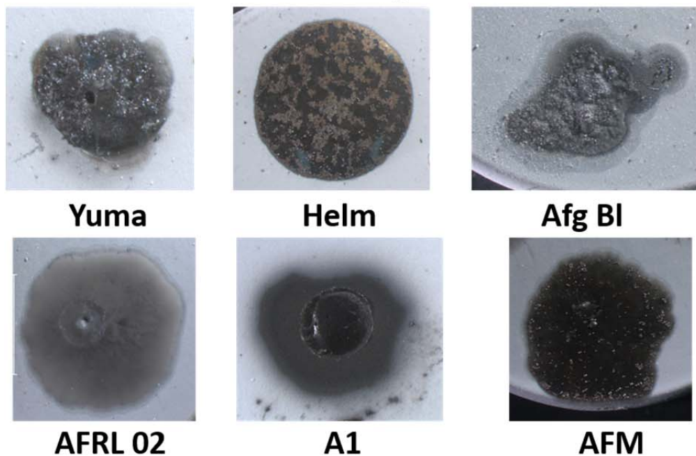
Figure 34: Wetting behavior of Phase 3 heated on TBCs at 1300 °C.
