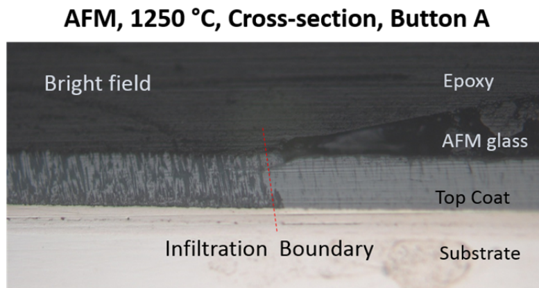
Figure 39: Optical cross-section image of Yuma and AFM heated to 1250 °C. Dashed curve indicates the edge of Yuma sample infiltrated into the top coat. Top Yuma image is presented in bright field microscopy while inset Yuma image is presented in dark field microscopy. AFM sample, imaged in bright field, indicates infiltration boundary by separating with a dashed line.
