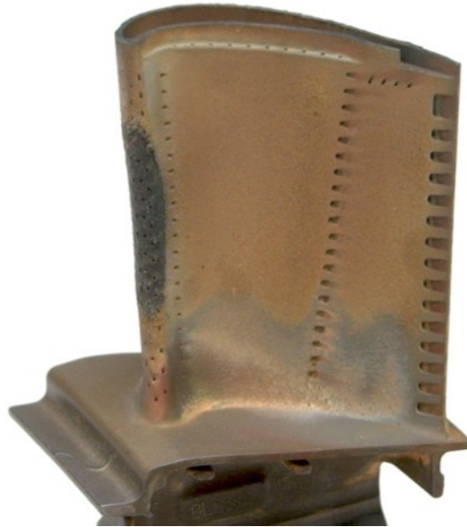
Figure 17: Turbine engine blade coated with CMAS
