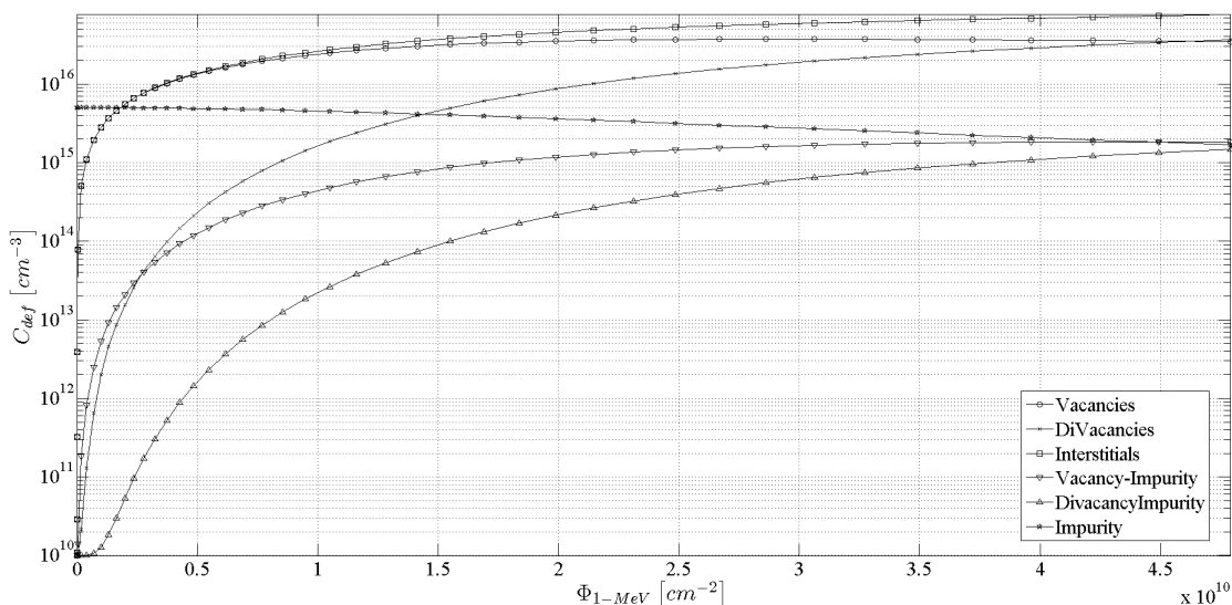
Figure 21. The first simulation using the model with six defect species and a time-averaged 1-MeV equivalent neutron flux of 5 \times 10^{10} n/cm -2 /s and an initial impurity concentration of 5 \times 10^{15} at/cm 3 .
