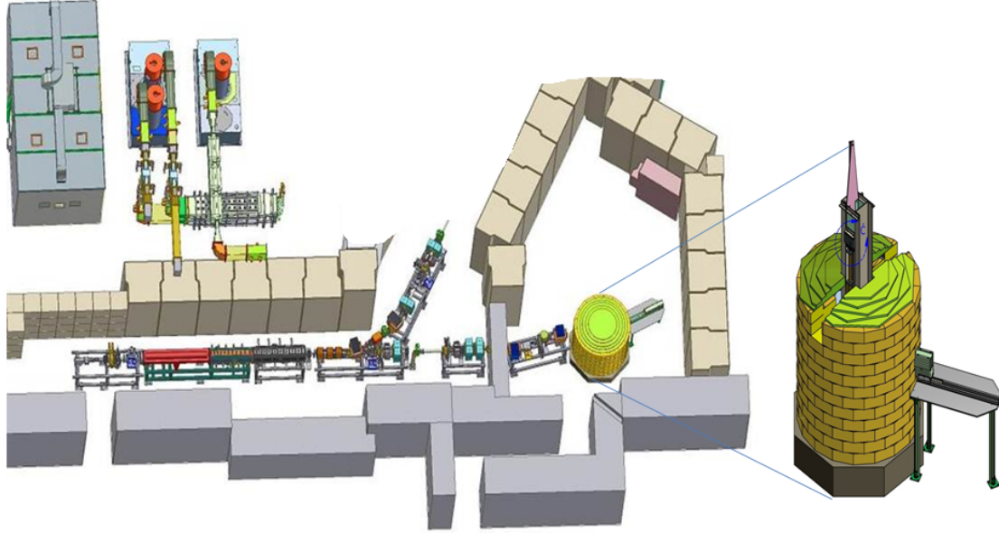
Figure 14. A schematic of the IU NREF beamline at the LENS.
