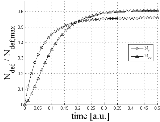
Figure 16. For this arbitrary selection of parameters, the vacancy population rises quickly, but reaches a secular equilibrium at a lower level than the di-vacancies during irradiation.
