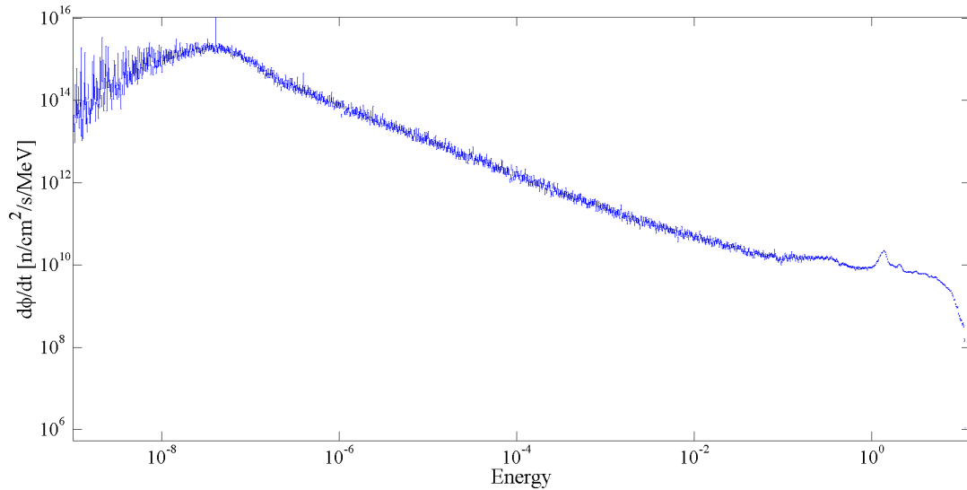
Figure 31. When operating the proton source at a current of 20 mA, the resultant neutron spectrum is scaled to a 1-MeV equivalent (Si) neutron flux of > 6 \times 10^{10} n/cm 2 /s.
