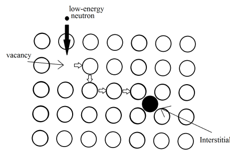
Figure 8. Schematic of the creation of a Frenkel pair (in this case using low-energy neutron bombardment of the crystal lattice). [10]
