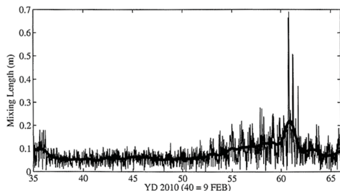
Fig. 10. Depth averaged mixing length ( \ell_m ) with the 40-h low-passed value indicated by the heavy line
