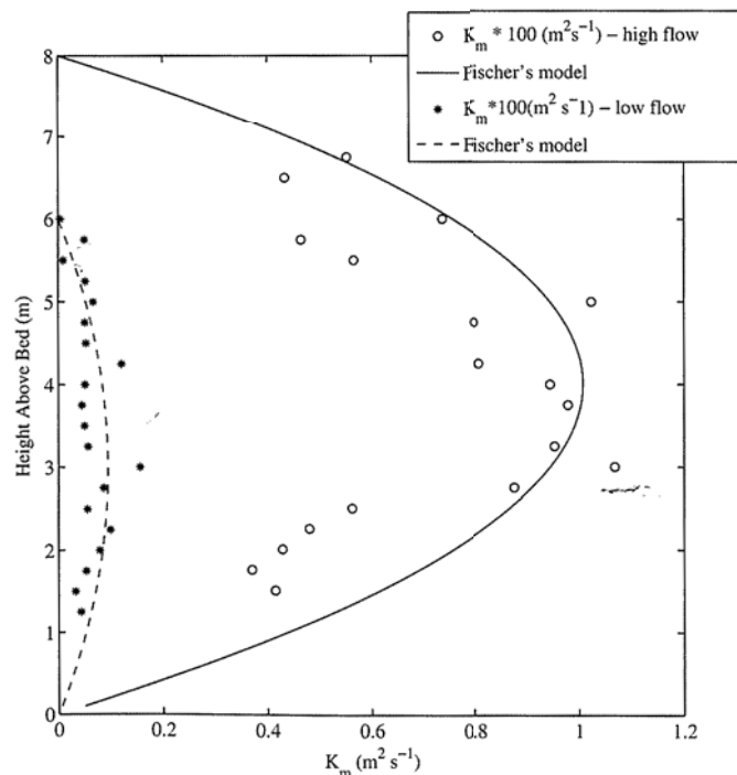
Fig. 11. Vertical profiles of K_m from Figs. 7 and 8 plotted with Fischer's model for the vertical structure of K_m
