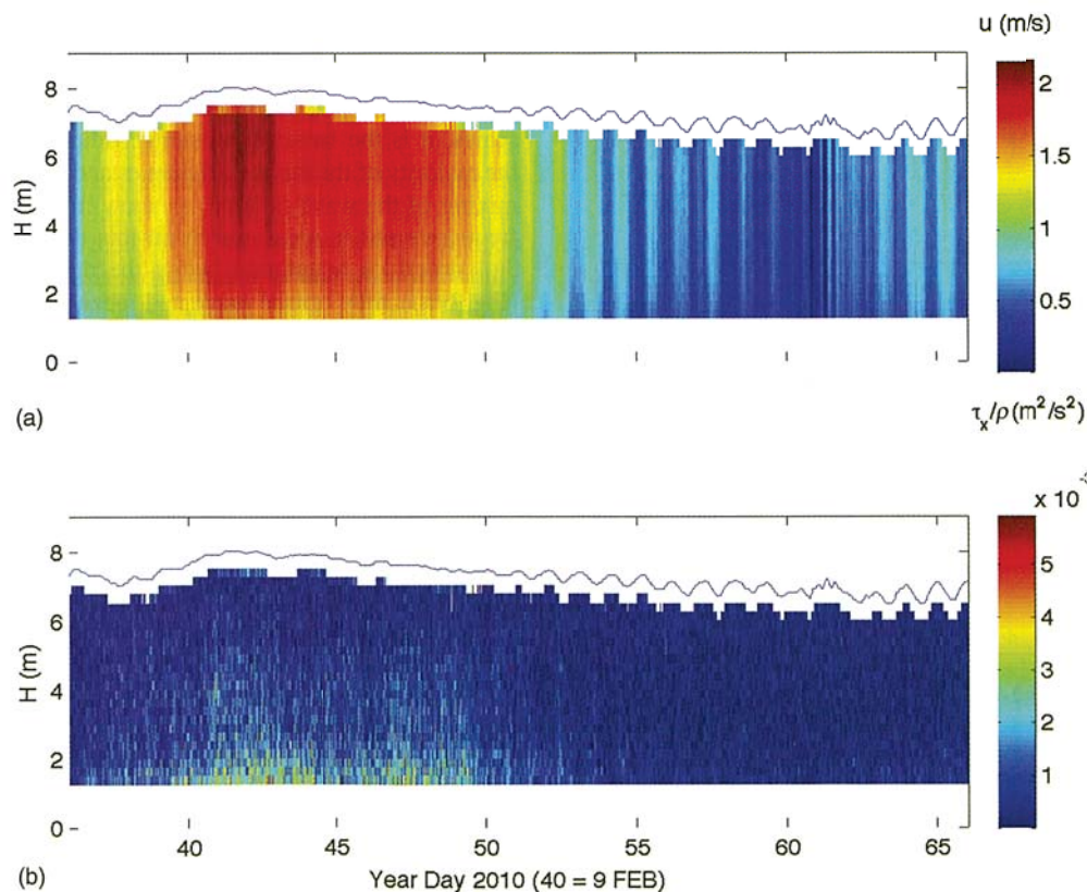
Fig. 5. (Color) Profiles through the experiment of (a) the along channel velocity, u ; (b) the turbulent stresses, -u'w'
