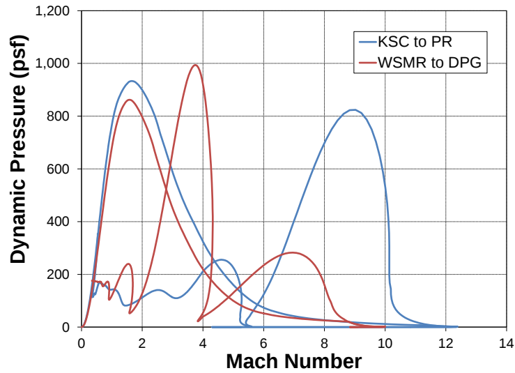
Figure 12. Initial Trajectories Plotted as Dynamic Pressure vs. Mach Number.
