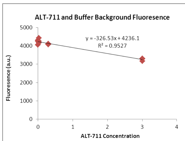
Figure 2. Fluorescence from the ALT treatment solutions at 7 days.
