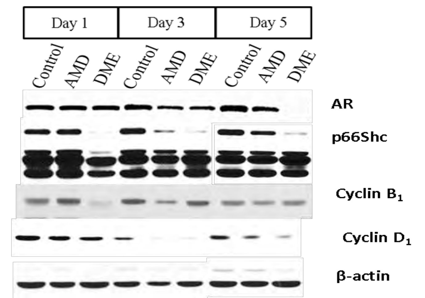
Fig. 4. The effects of AMD and DME on AR, p66Shc and cell cycle protein expression. \beta -Actin was detected as a loading control. The data shown is a representative from three sets of independent experiments.
