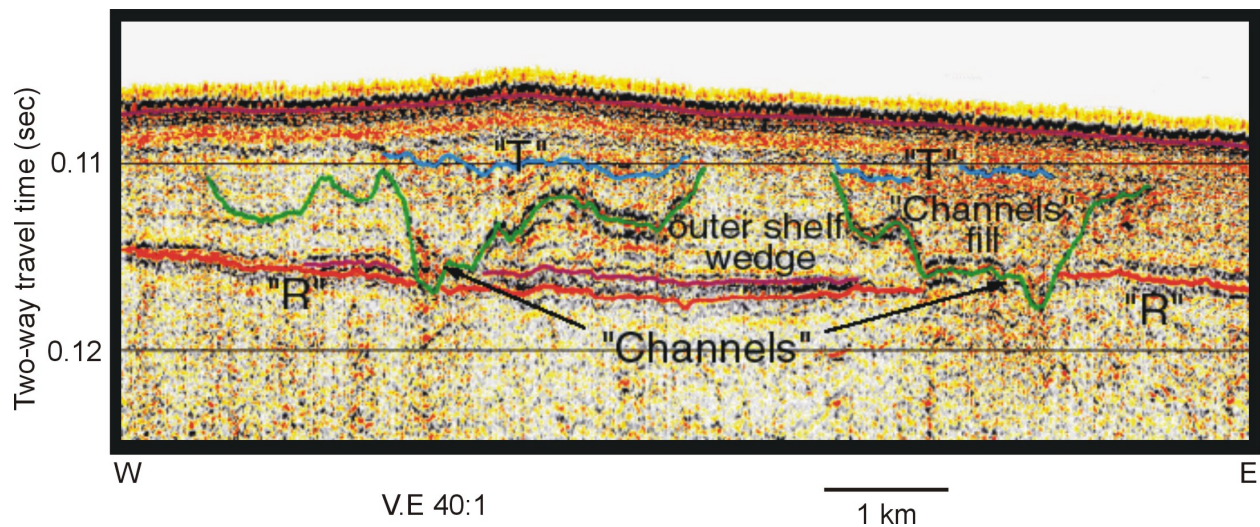
Figure 1. Huntec seismic profile on the New Jersey middle shelf, in ~80 m of water. Horizon interpretations are from Duncan et al., 2000.
