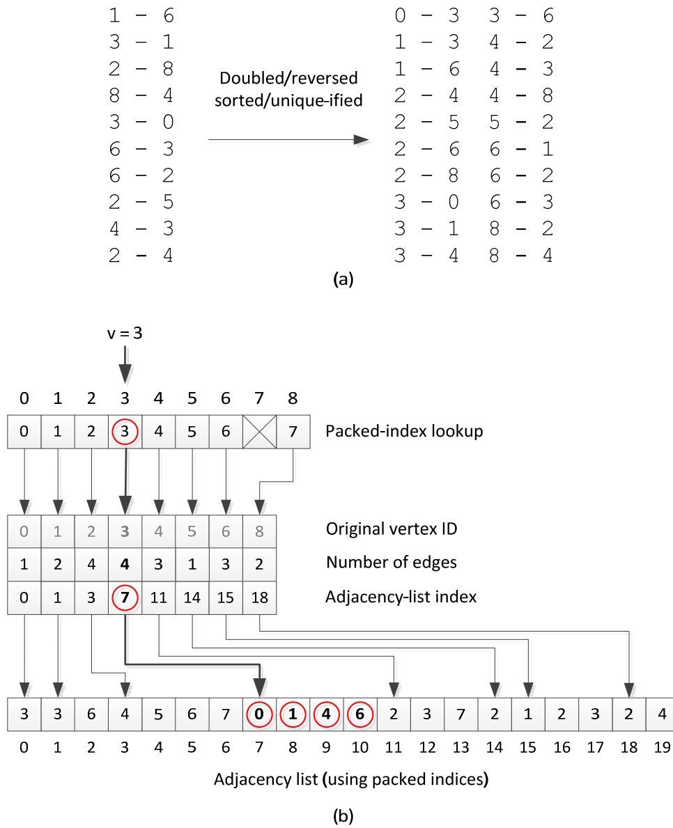
Figure 6: Data Structures for Sequential CSR Algorithm
