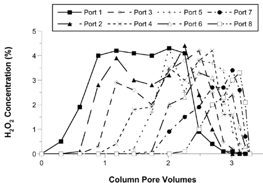
Figure 1-13. Concentration of 5% H 2 O 2 stabilized by 25 mM phytate at eight ports in a column of iron-coated sand
