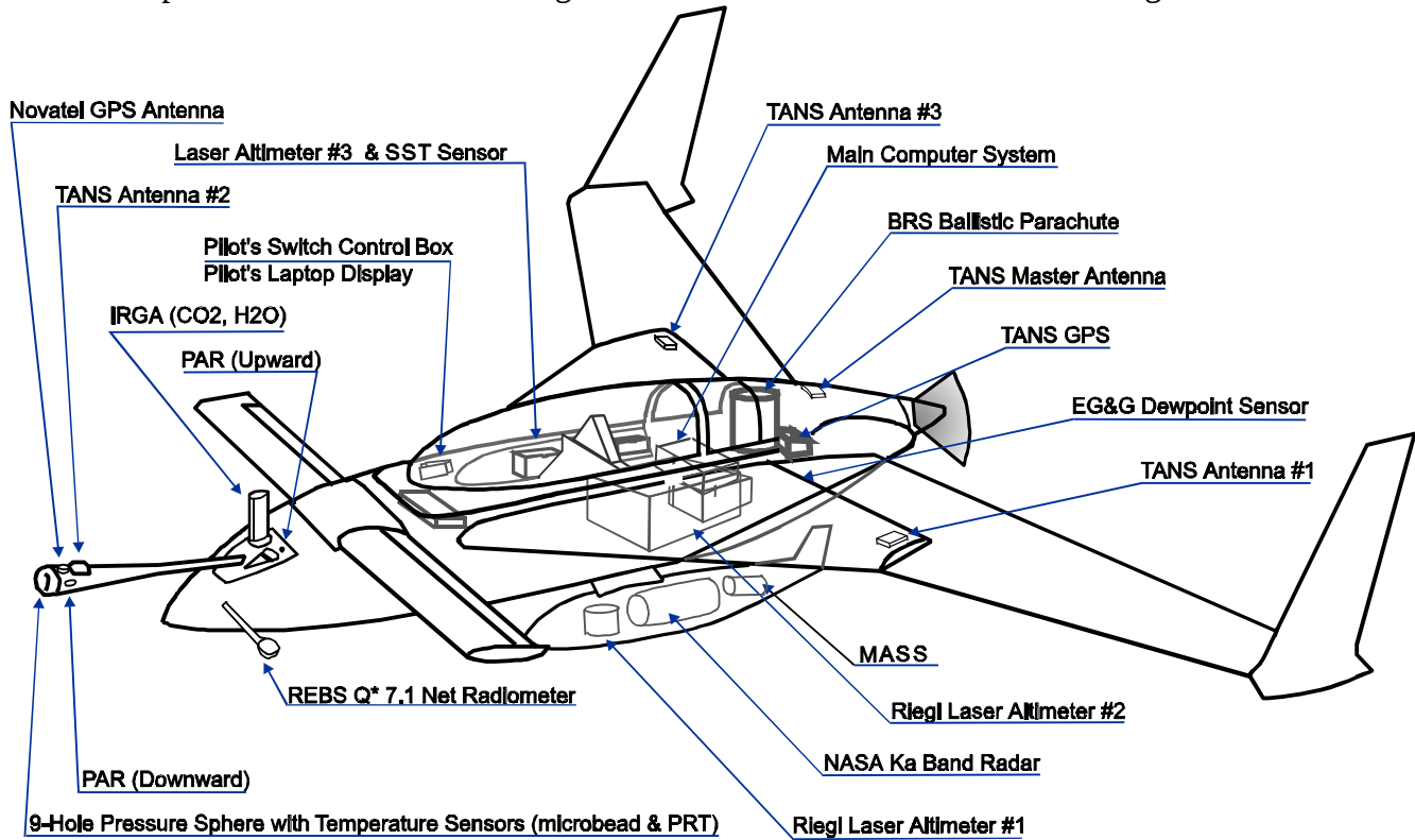
Fig. 2. Configuration of the various instrument systems on LongEZ N3R used for SHOWEX.
