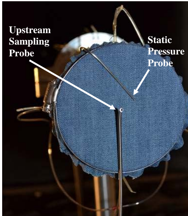
Figure A-11: Front of Wind Tunnel Sleeve Fixture with Upstream Sampling Probe and Static Pressure Probe
