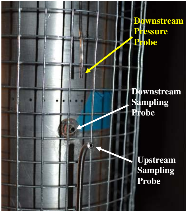
Figure A-8: Front of Wind Tunnel Swatch Holder with Upstream Sampling Probe and Static Pressure Probe
