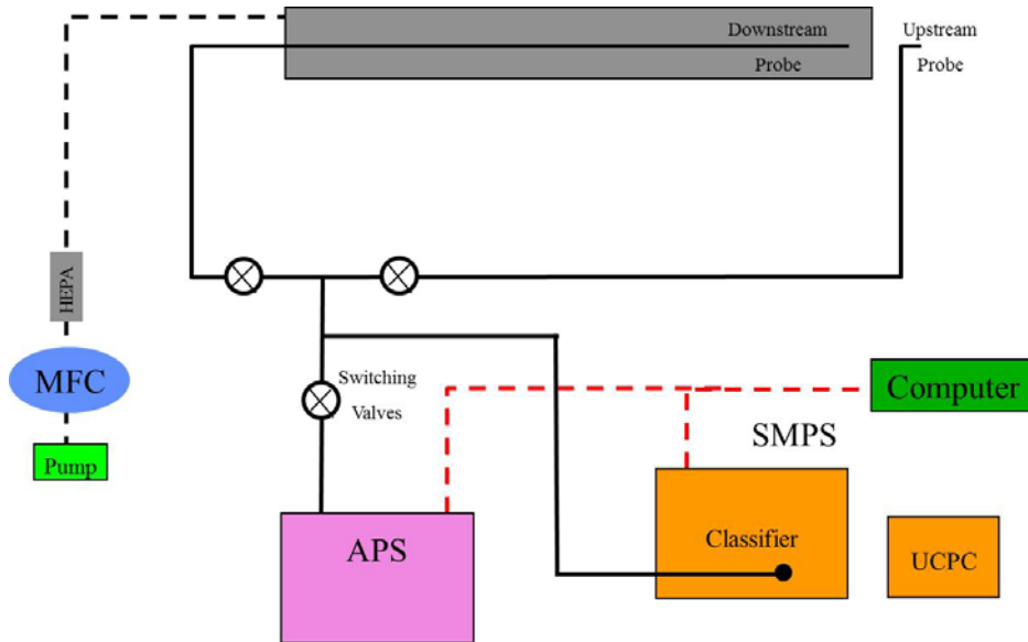
Figure A-16: Schematic of Wind Tunnel Switch Holder DOS Challenge, High Wind Tunnel Speed
