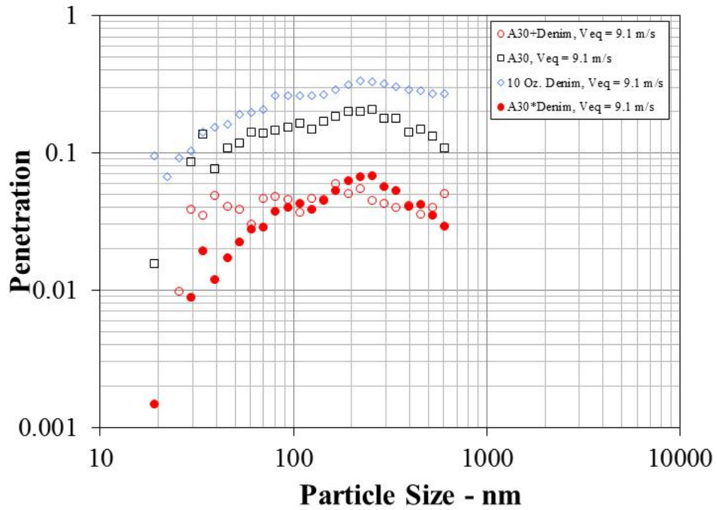
Figure A-62: Additive Effect of Fabric Penetration, Bench Top Swatch Test, Aerosil Challenge: V_{eq} = 9.1 \text{ m/s}
