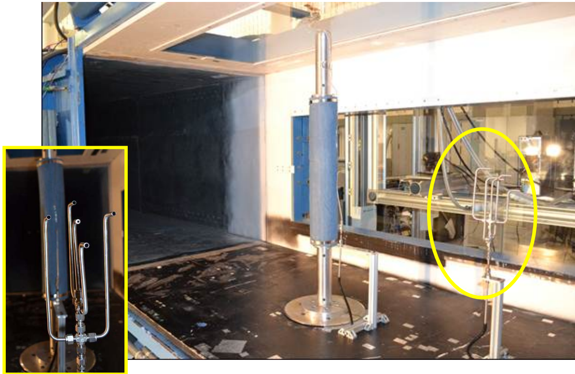
Figure A-5: Wind Tunnel Ejectors, Inset: Front View
