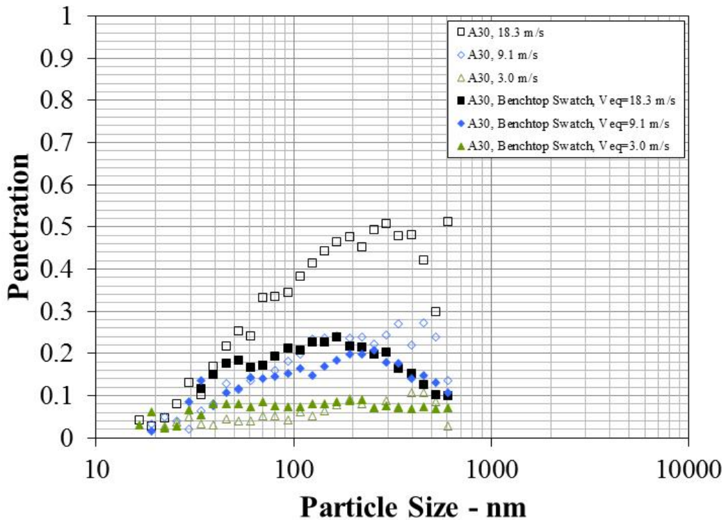
Figure A-48: Fabric Penetration Comparison between Wind Tunnel Component and Bench Top Swatch, Aerosil Challenge: A30
