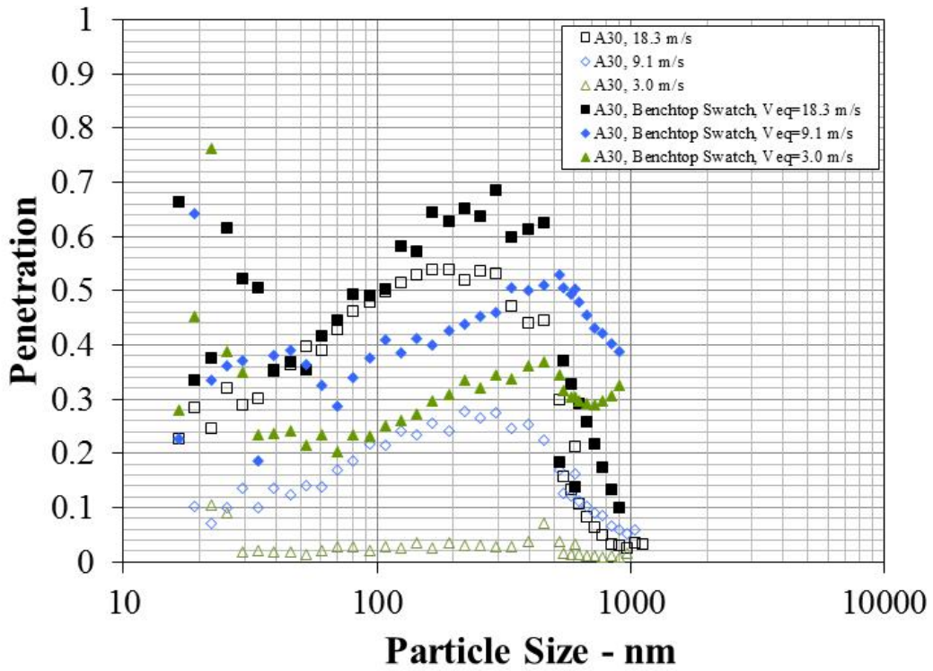
Figure A-44: Fabric Penetration Comparison between Wind Tunnel Component and Bench Top Swatch, DOS Challenge: A30
