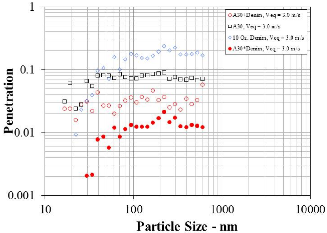
Figure A-63: Additive Effect of Fabric Penetration, Bench Top Swatch Test, Aerosil Challenge: V_{eq} = 3.0 \text{ m/s}
