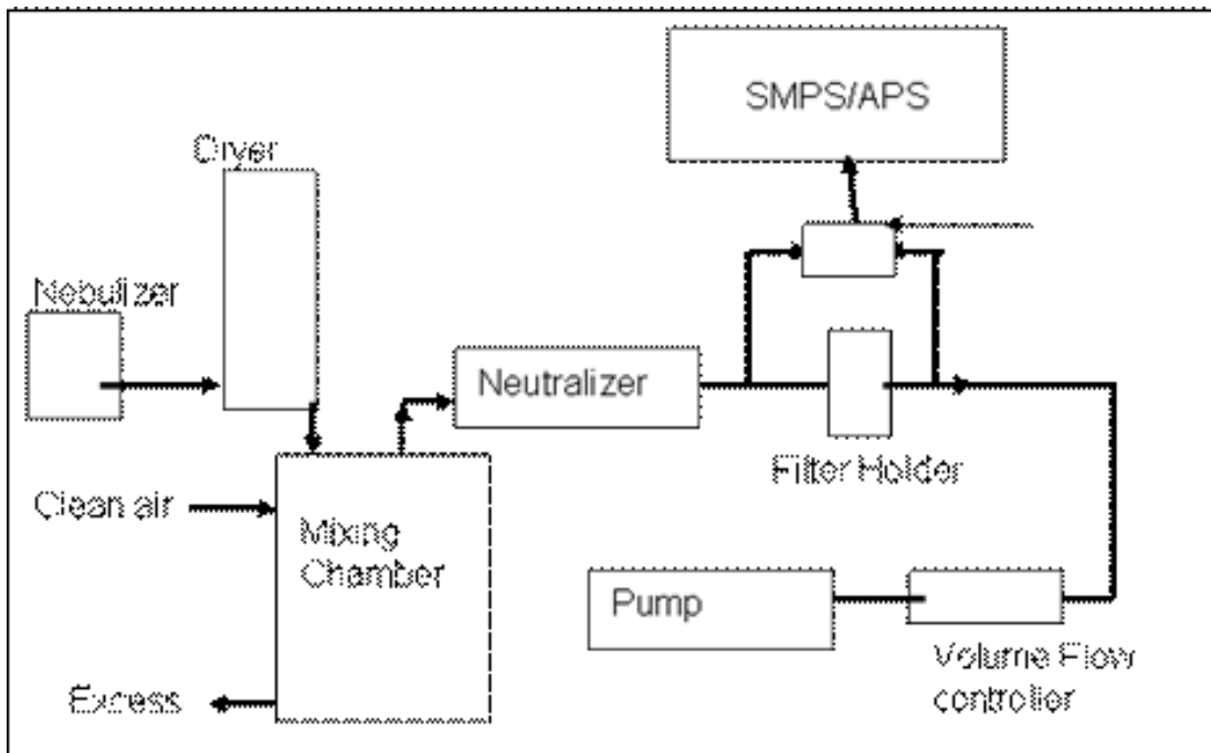
Figure A-20: Schematic of Bench Top Setup at Clarkson University, reference 6
