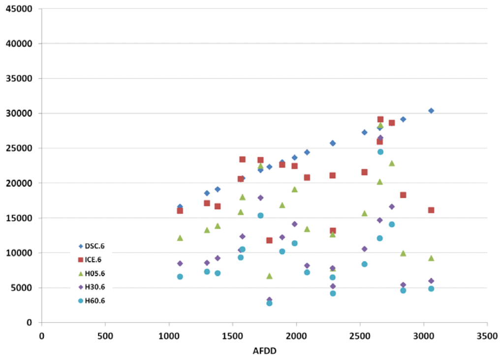
Figure 39. The aqueduct with 6 in. of outside insulation: the total maximum ice volume by AFDD (ft 3 ) formed over each winter season.
