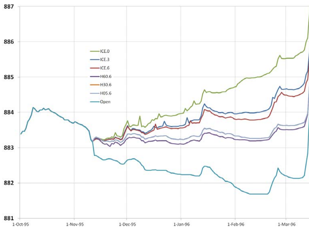
Figure 30. Upstream water levels for water year 1996 for different scenarios and for open water.
