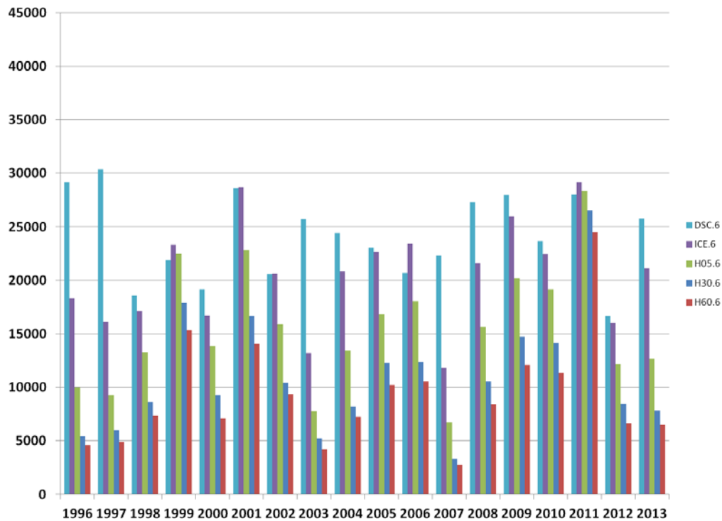
Figure 38. The aqueduct with 6 in. of outside insulation: the total maximum ice volume (ft 3 ) formed over each winter season.
