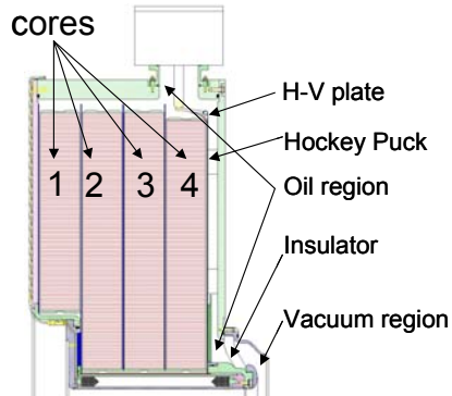
Figure 1. Cross-section of the original DARHT II induction cell design.
