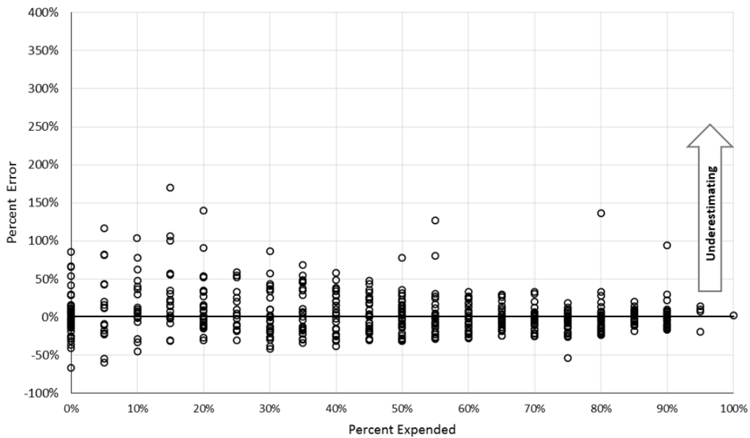
Figure 8. Predictive Model-Corrected Estimate Error by Percent Expended
