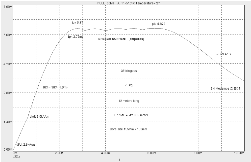
Figure 5. 63 MJ Muzzle Energy - Current Vs Time
