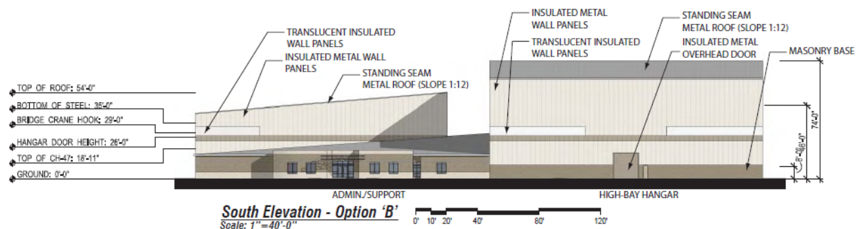
Figure 4-3. Building Features and South Elevation of the Proposed FAF (Facing Mat 3)
