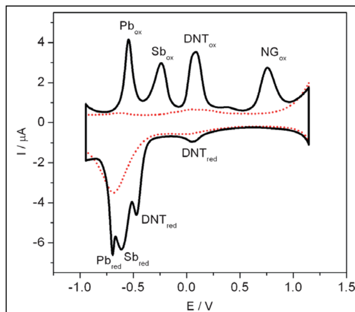
Fig. 1. Cyclic square-wave voltammogram at the bare GCE for a mixture of trace metals and explosives constituents of GSR: 3 ppm Pb, 10 ppm Sb, 50 ppm NG, and 10 ppm DNT. Square wave parameters: Estep, 4 mV; amplitude, 25 mV; frequency, 8 Hz; and teq, 5 s; (reduction) Estart, 1.15 V; and Estop, 0.95 V; (oxidation) Estart,accum, 0.95 V; Estop, 1.15 V; and taccum, 120 s. Electrolyte, acetate buffer (pH ¼ 4.5).
