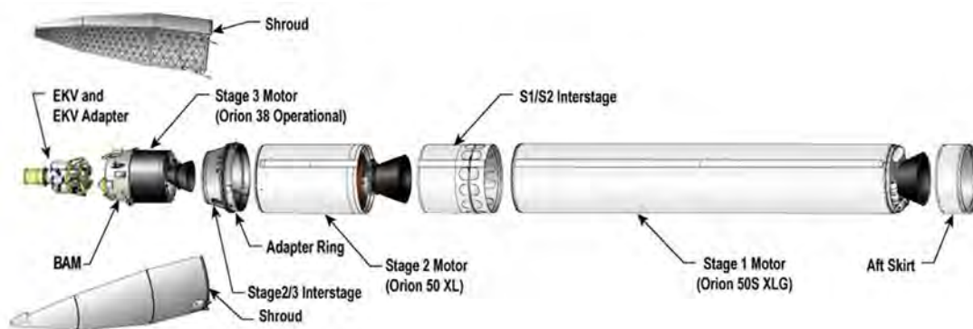
Figure 2. Ground-Based Interceptor
