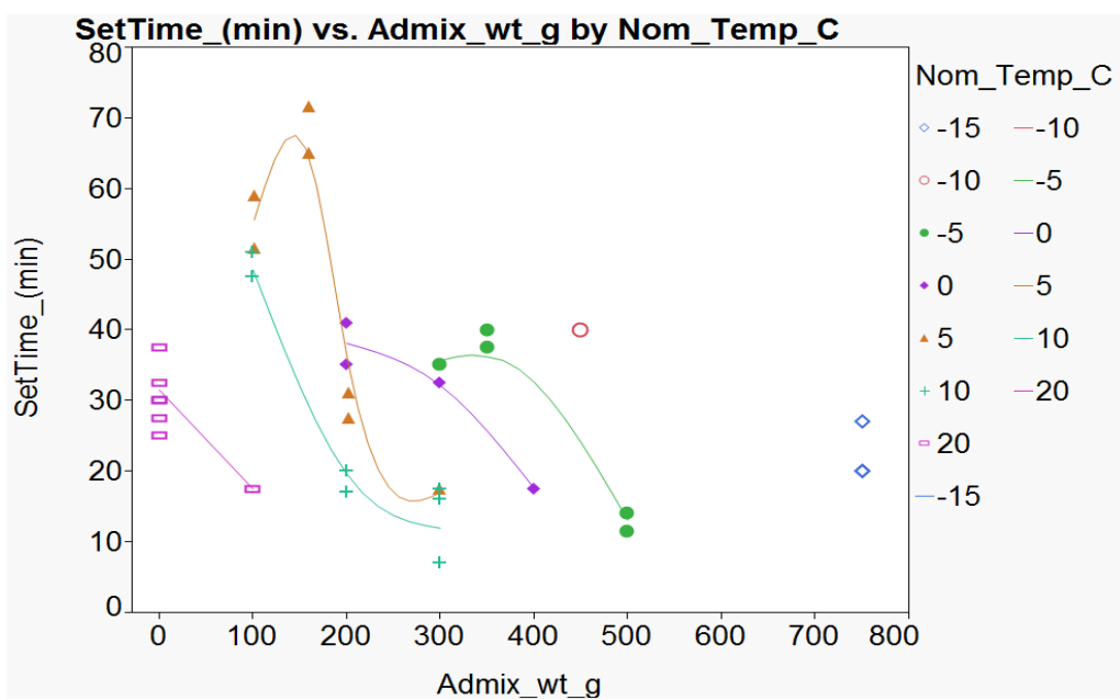
Figure B2. Task 3 (aluminum sulfate) testing: set time (time to reach 500 psi, in min) vs. the amount of aluminum sulfate used (g), filtered by testing temperature (°C). Tests shown only where 2 hr UCS is greater than 2500 psi.
