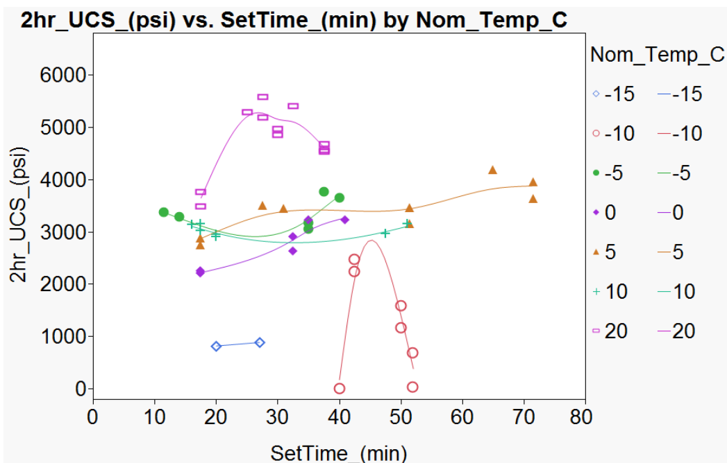
Figure B6. Task 3 (aluminum sulfate) testing: 2 hr UCS vs. set time (time to reach 500 psi, in min), filtered by testing temperature ( ^{\circ}\text{C} ). All completed tests in task 3 are shown.
