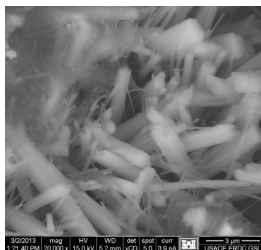
(b) 20K× SEM micrograph
