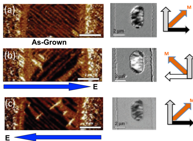
FIG. 13. In-plane PFM of the BiFeO 3 domain structure (left) and XMCD of a Co 0.90 Fe 0.10 feature (middle) in a device architecture where an in-plane electric field can be applied (blue arrows). BiFeO 3 and the coupled Co 0.90 Fe 0.10 feature are as-grown (a), 1st switch (b) and 2nd switch (c) states. (b) Schematics illustrating the correlation of XMCD contrast to moment direction and the direction of the total moment (orange arrow). Reprinted with permission from Chu et al. , Nature Mater. 7 , 478 (2008). Copyright 2008 Chu et al.
