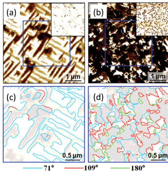
FIG. 2. (a) and (b) IP PFM (and out-of-plane PFM: insets) images of two BiFeO 3 films deposited on SrTiO 3 substrates at different deposition rates. (c) and (d) Line traces of the domain walls present in the two films highlighting that the domain structure and the composition of the domain walls can be tuned with deposition rate. The domain structure in (a) is primarily 71° domain walls while that in (b) is largely 109° domain walls. Reprinted with permission from Martin et al. , Nano Lett. 8 , 2050 (2008). Copyright 2008 American Chemical Society.
