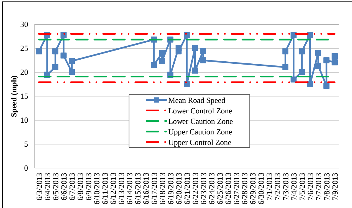
Figure B-2. Mean road speed and caution and control bounds.
