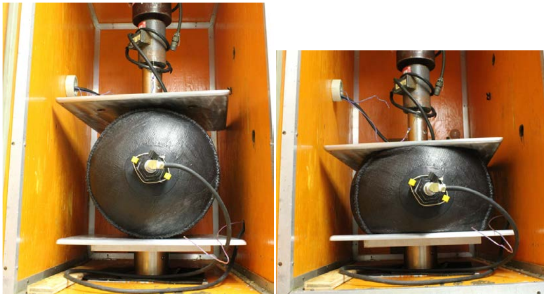
Figure 10. Low-temperature compression tests on a sample ARCS pontoon built by FFF using materials designated Samples 14 and 16 here (Weale et al. 2011). The photo on the right in Figure 4 shows the liner-shell construction of this pontoon sample.
