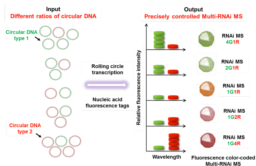
Figure 4. Design of multiple component RNAi microsponges with ratio control approach that allows tuning of the relative amounts of each siRNA sequence.
