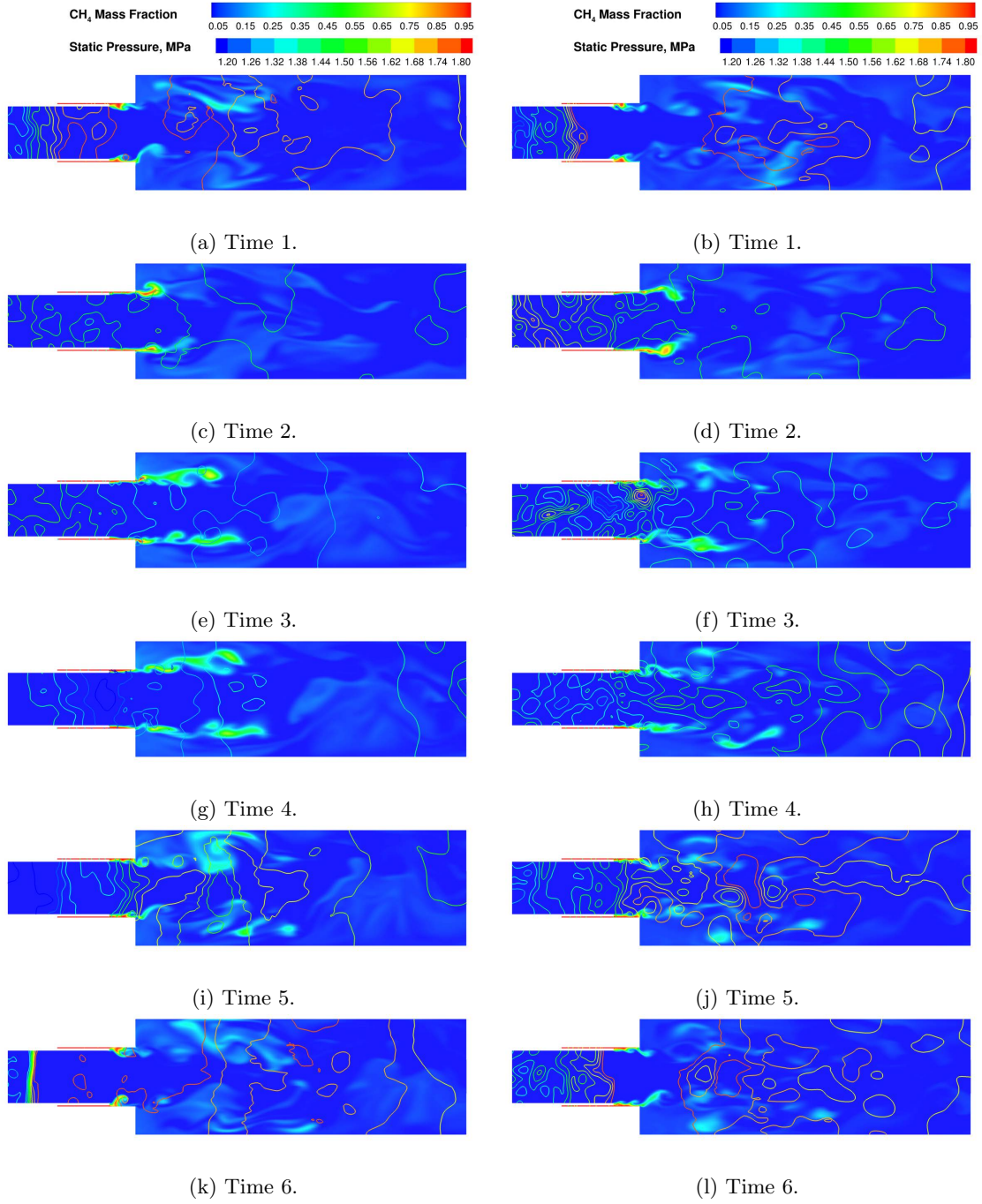
Figure 7: Time evolution of \text{CH}_4 mass fraction for a single cycle. Right images show the baseline case without swirl and the images on the left show the case with 9^\circ of swirl. Contours are \text{CH}_4 mass fraction; lines are colored with static pressure.
