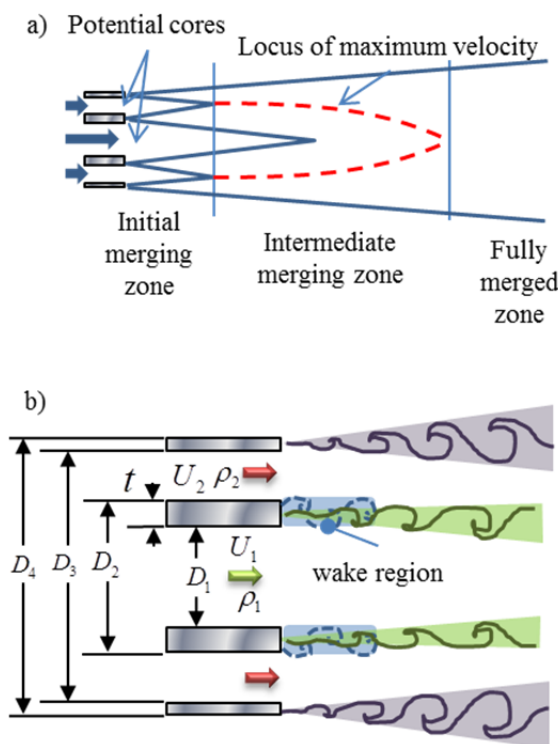
Figure 1. The a) global and b) near-field features of the coaxial jet.
