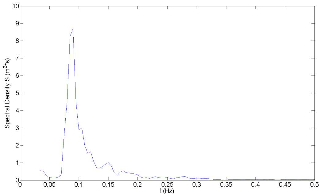
Figure 92: Wave Spectra, 9/22/2013 1020-1040
