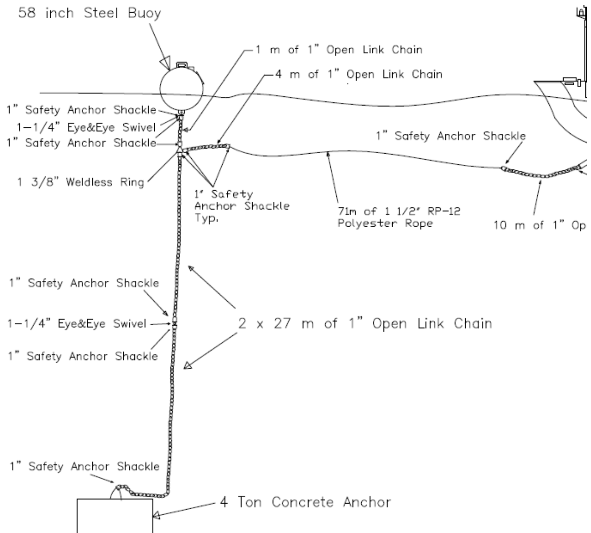
Figure 26: Bow mooring leg connection details, 2012 configuration (AXYS 2012-c)
