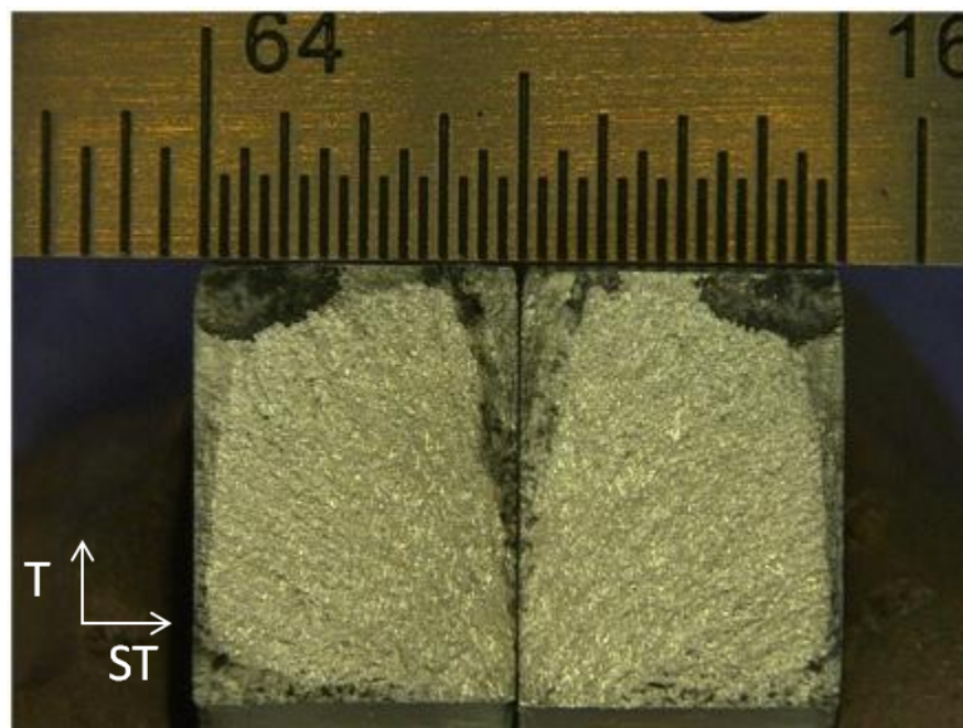
Fig. 126 Fracture surfaces for constant amplitude non-cold-expanded specimen (19X magnification); OFF-NCX2024-1, Constant-amplitude R=0.1 , \sigma_{\max} = 25 ksi, 20 Hz, Lab Air
