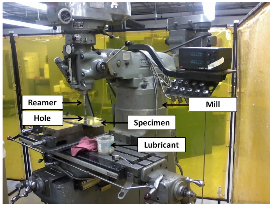
Fig. 18 Photo of mill at the University of Utah used to ream final diameter for cold-expanded specimens
