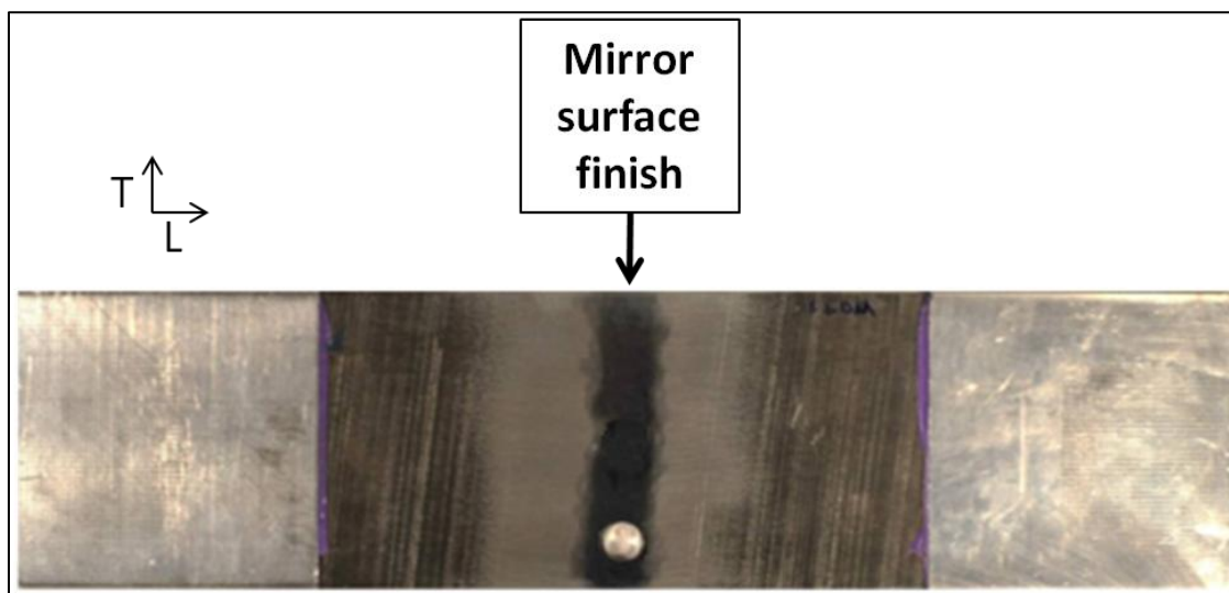
Fig. 19 Typical cold-expanded specimen after final sanding and polishing; view looking down at the EDM face, L and T orientations indicated
