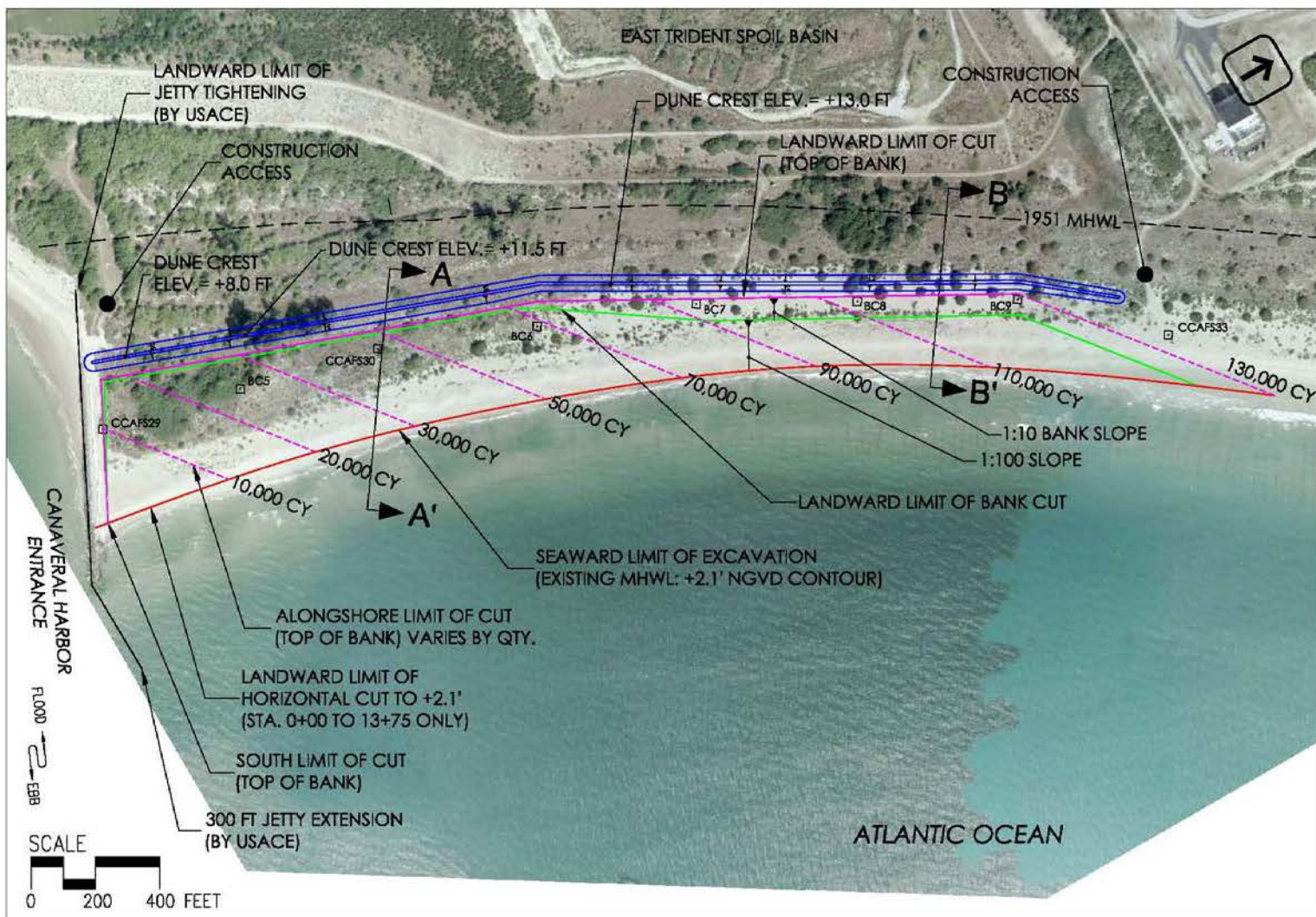
Figure 3: Plan View of Project Borrow Area North of Canaveral Harbor Entrance
