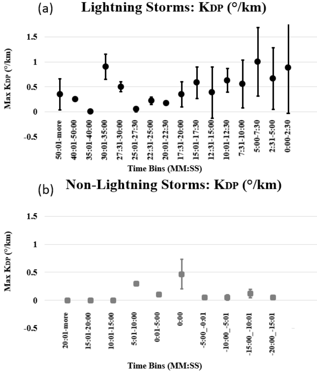
Figure 14: Specific differential phase -10^{\circ}\text{C} thermal level time bins. Plot of radar volume scans at -10^{\circ}\text{C} height of 21 lightning producing single-cell thunderstorms leading up to lightning initiation at 0:00 min, organized into specific differential phase time bins (a) and 13 non-lightning storms with maximum K_{DP} values organized into time bins (b). The marker (black dot for lightning storms (a) and grey square for non-lightning storms (b)) on each plot represents the average K_{DP} value for the time bin specified and the error bars represent the standard deviation.
