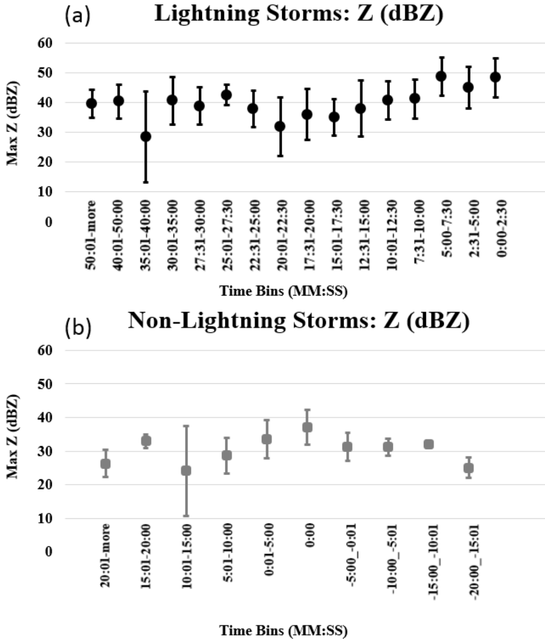
Figure 12: Reflectivity -10°C thermal level time bins. Plot of radar volume scans at -10°C height of 21 lightning producing single-cell thunderstorms leading up to lightning initiation at 0:00 min, organized into reflectivity time bins (a) and 13 non-lightning storms with maximum Z value occurring at 0:00 min organized into time bins (b). The marker (black dot for lightning storms (a) and grey square for non-lightning storms (b)) on each plot represents the average Z value for the time bin specified and the error bars represent the standard deviation.
