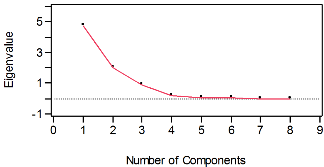
Figure 4-14. Plot showing the relationship between the primary PCs and how they account for the 2010 comparison dataset variability in the PCA evaluation shown in Table 4-10.
