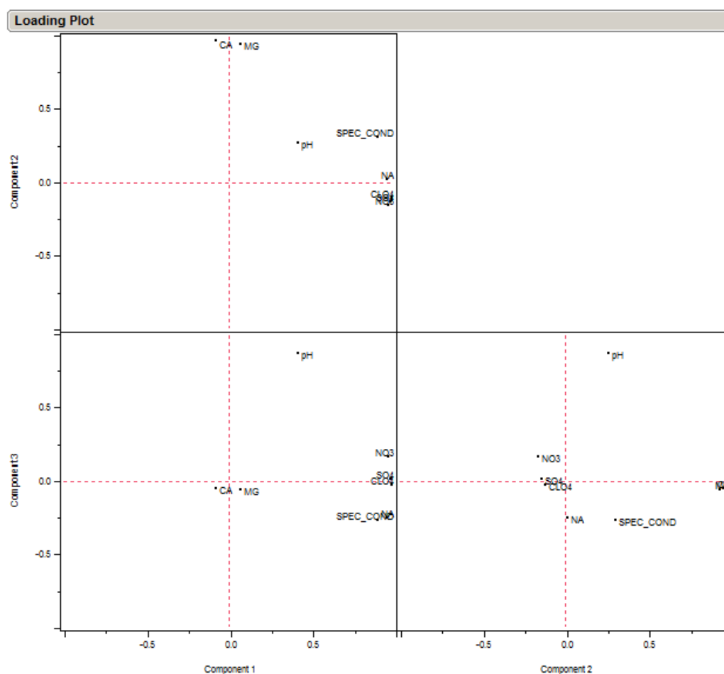
Figure 4-15. Loading plots showing the relationship between the primary principal components PCs (accounting for > 90% of the dataset variability) and analysis variables for the 2010 comparison dataset PCA evaluation shown in Table 4-10.
