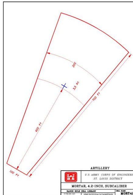
Mortar, 4.2", Subcaliber
