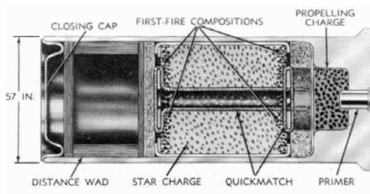
Signal, Illumination, Aircraft. AN-M43 Series
