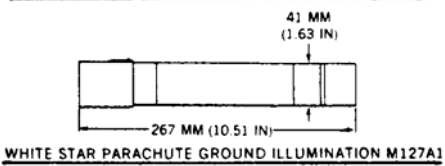
Signal, Illumination, Ground. RED STAR M126A1, WHITE STAR M127A1, M158; M195; M207, M159
