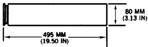
Bomb, 6-lb, Incendiary, Cluster, AN-M69, AN-M69X
