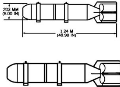
Bomb, 100-lb, Incendiary, AN-M47
