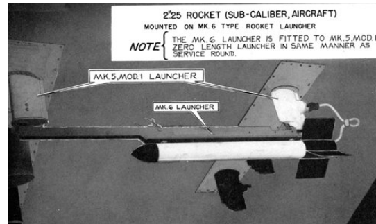
Rocket, 2.25-inch SCAR, Practice, Mk1
