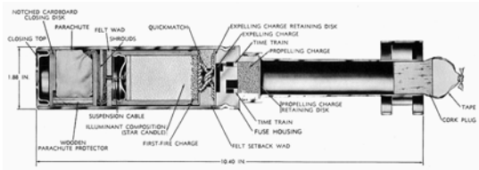
Signal, Illumination, Parachute, Rifle. M17 Series (M17A1)
