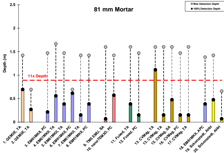
Figure 2-6. Performance of Selected Detection Systems at the APG Open-Field Standard Test Site (100% Detection Depth and Max Detection Depth)
