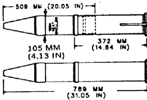
Projectile, 105 mm, HEAT & TP. M67
