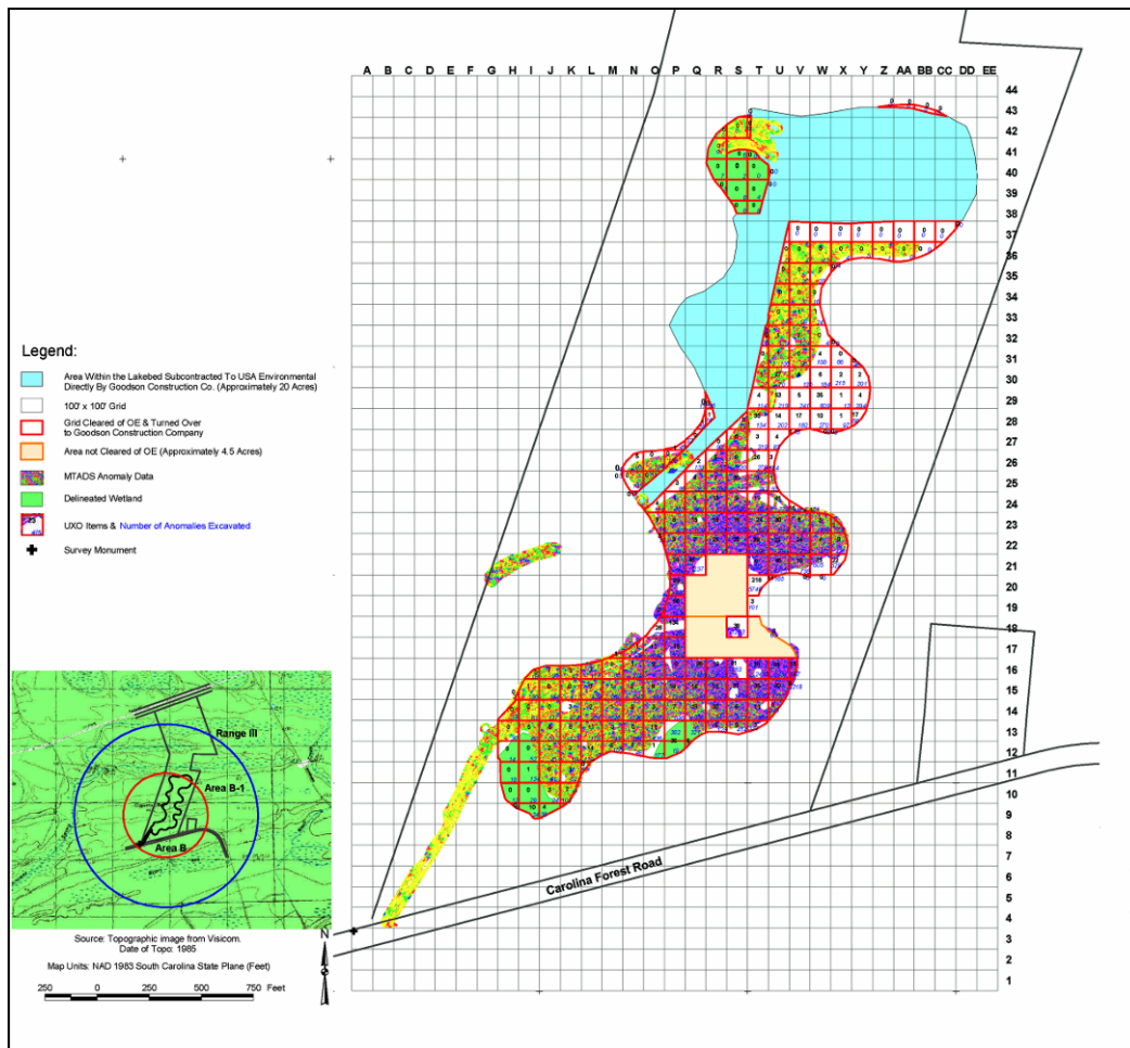
Figure CBGR-5. Detail of Portion of Impact Area Showing the MTADS Anomaly Data Generated during the TCRA, Range III, Conway BGR
