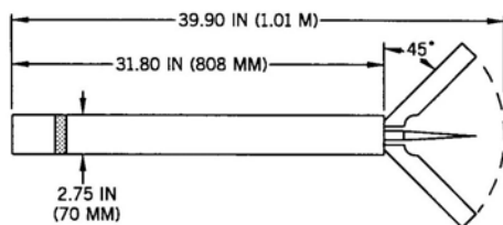
Rocket, 2.75-inch FFAR, Motor, MK1, 2, 3, & 4; SR105-AJ-1; LSFFAR, MK 40
