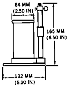
Signal, Illumination, Parachute, Rifle. M17 Series (M17A1)
