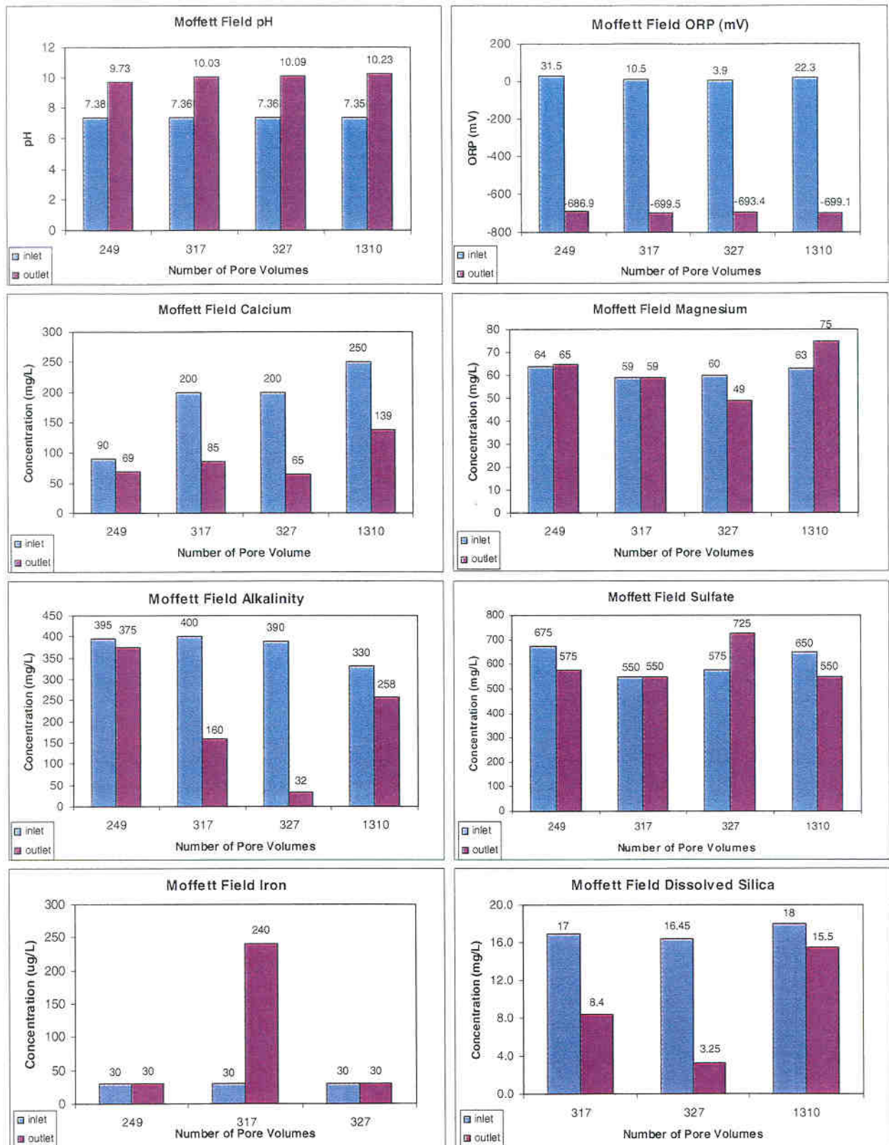
Figure 5-15. Bar graphs for former NAS Moffett Field column showing input and output concentrations of inorganic analytes (filtered).
