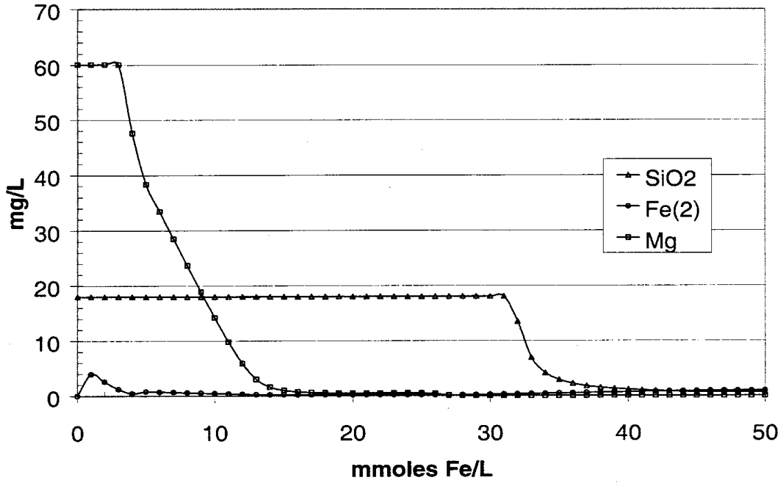
Figure 5-23. Profiles of silica, Fe(II), and Mg based on Case 1.
