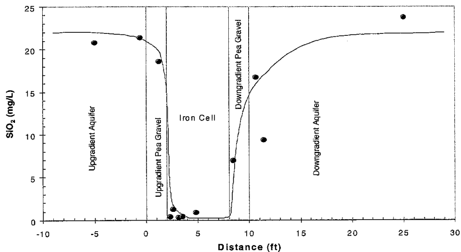
Figure 5-1. Plot showing the distribution of dissolved silica in the former NAS Moffett Field PRB in October 1998.
