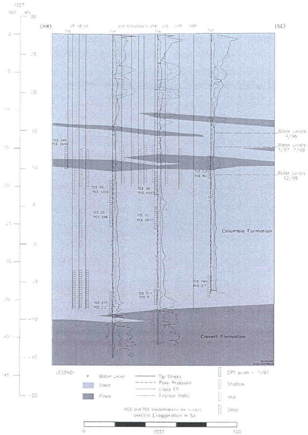
Figure 3-5. Lithology at the Dover AFB PRB.
