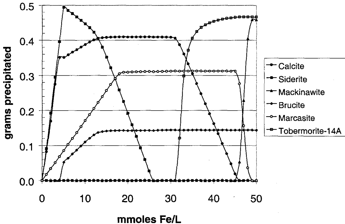
Figure 5-25. Masses of minor precipitates based on Case 1.
