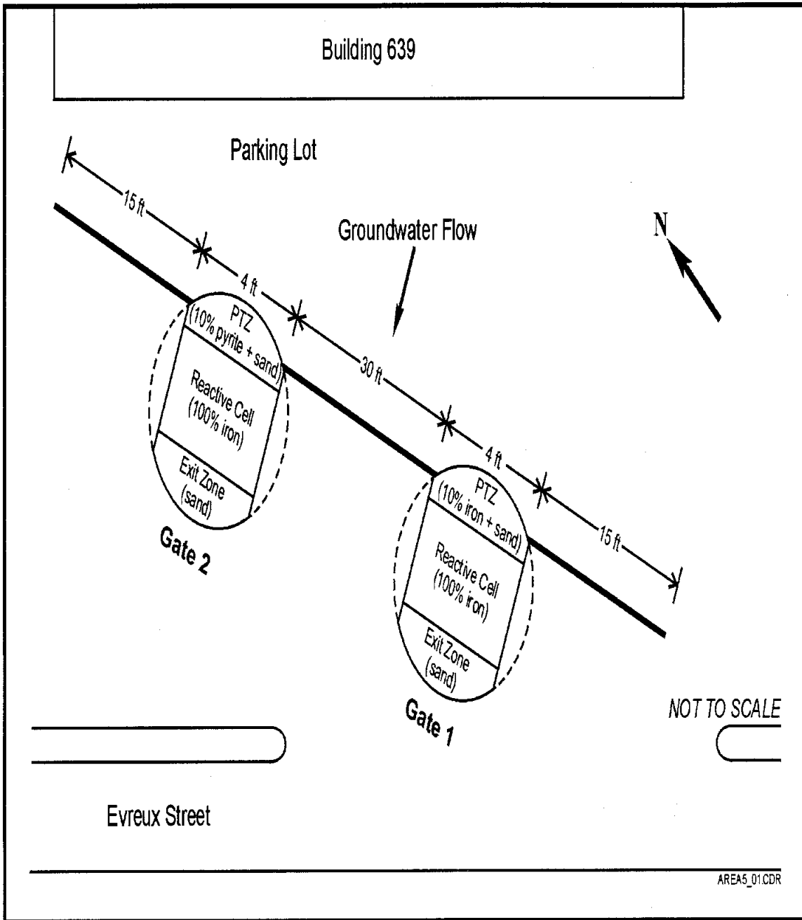
Figure 3-6. Plan view of PRB at Dover AFB.
