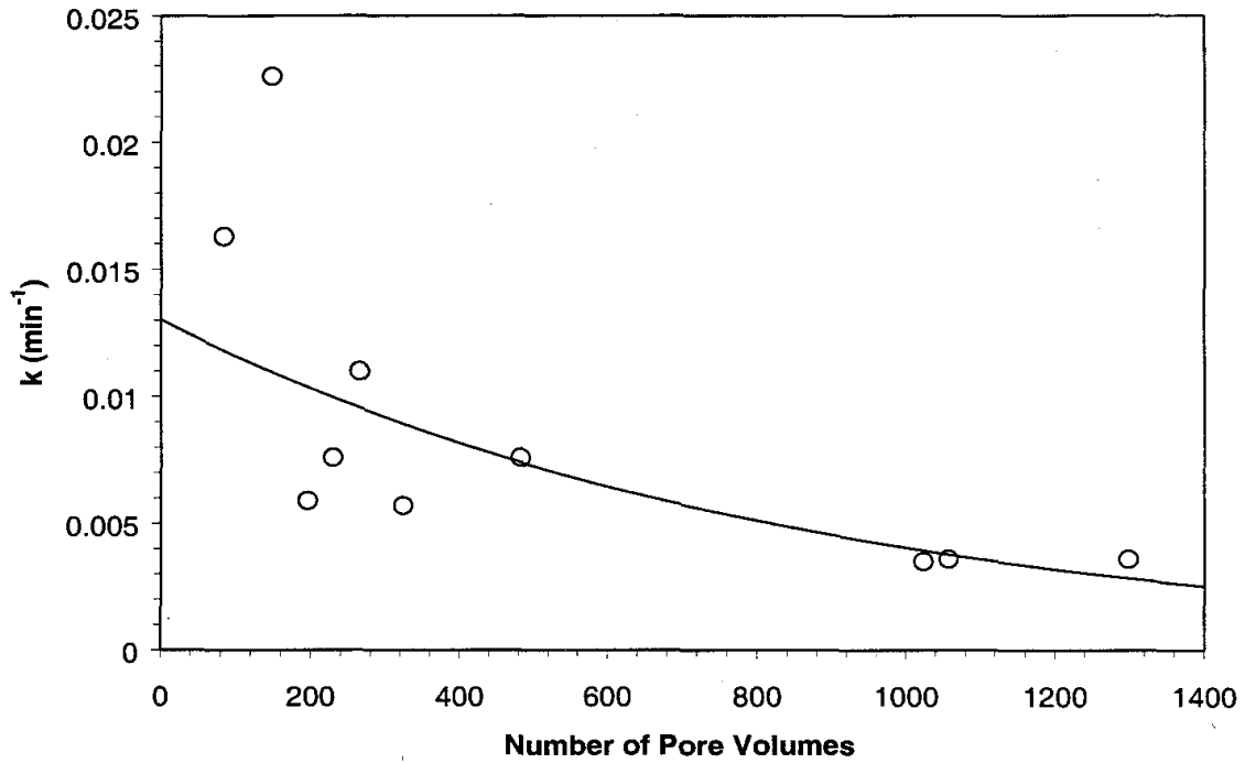
Figure 5-18. Plot of TCE degradation rates for Lowry column at different cumulative pore volumes.
