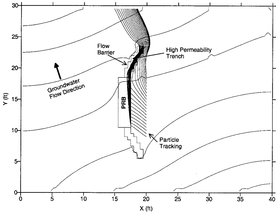
Figure 6-22. Base case model and groundwater flow at an angle to the PRB.
