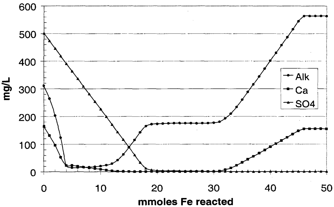
Figure 5-22. Profiles of alkalinity, Ca, and sulfate based on Case 1.
