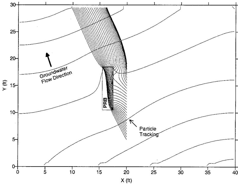
Figure 6-23. Model with trench and groundwater flow at an angle to the PRB.
