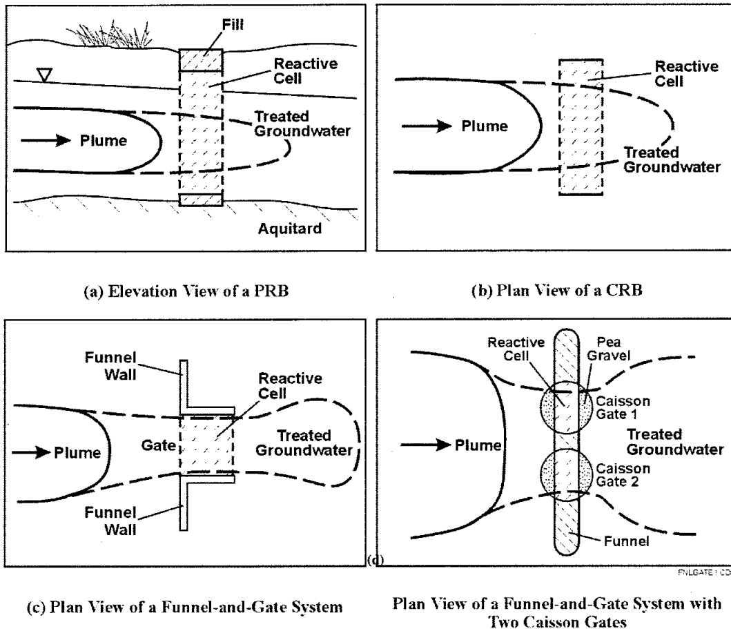
Figure 2-1. Schematic illustrations of some PRB configurations.
