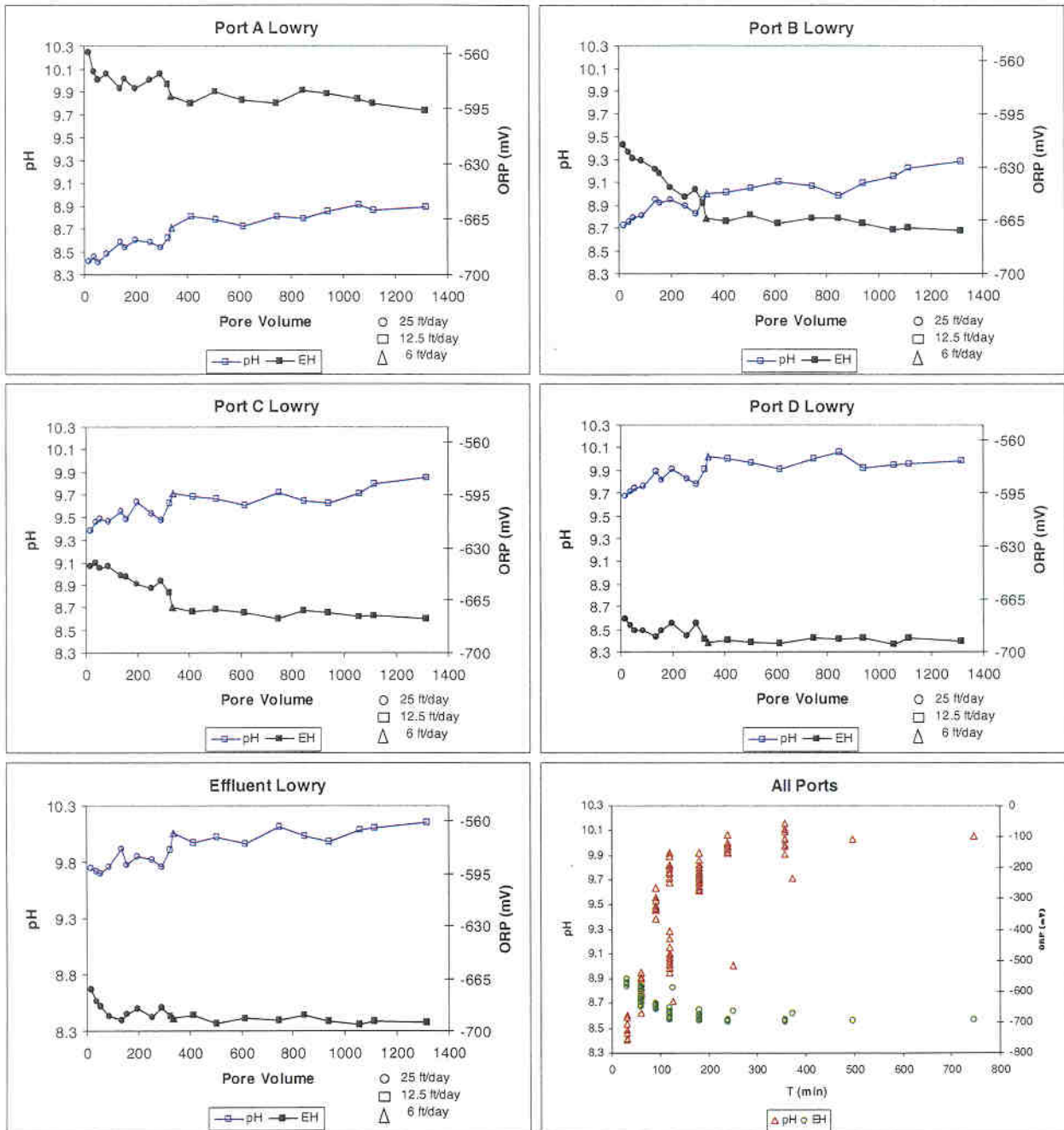
Figure 5-17. pH and ORP values in the Lowry column at different pore volumes ages.
