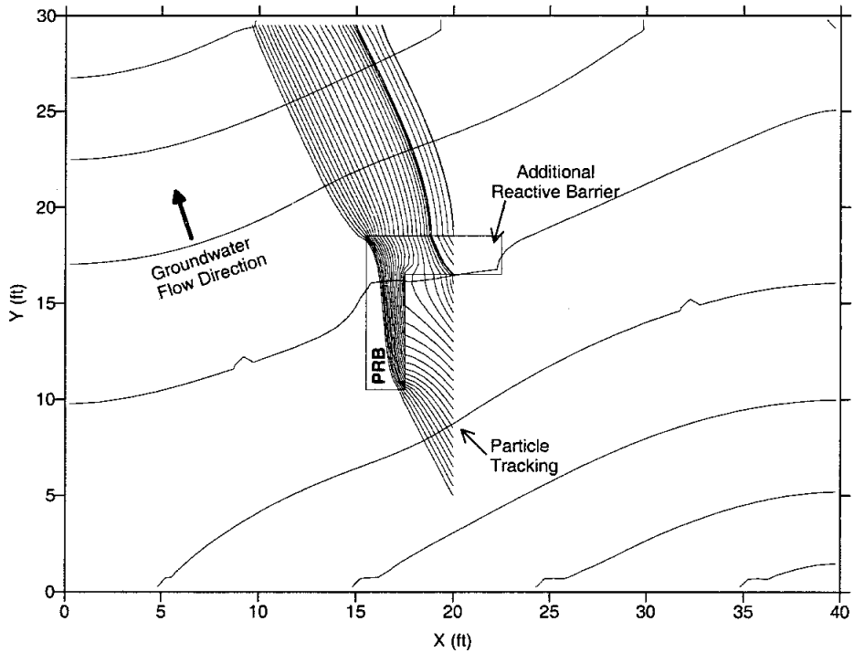
Figure 6-27. Model with additional reactive barrier and groundwater flow at an angle to the PRB.
