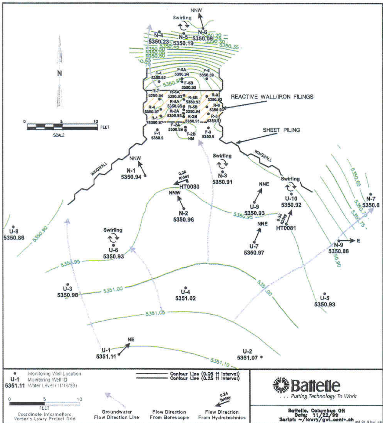
Figure 6-4. November 1999 water levels and other hydraulic measurements at former Lowry AFB PRB.
