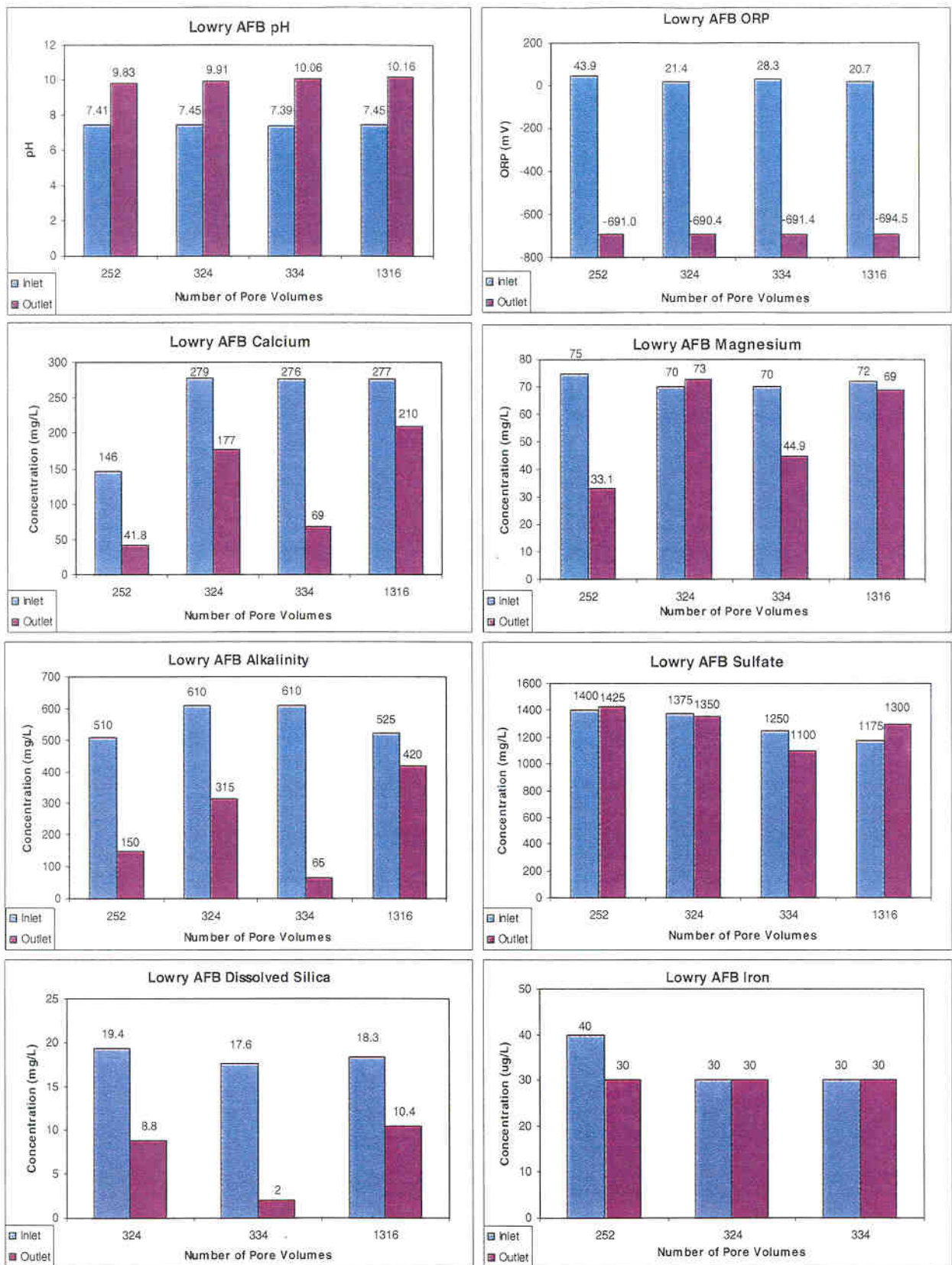
Figure 5-20. Bar graphs showing input and output concentrations of inorganic analytes (filtered).
