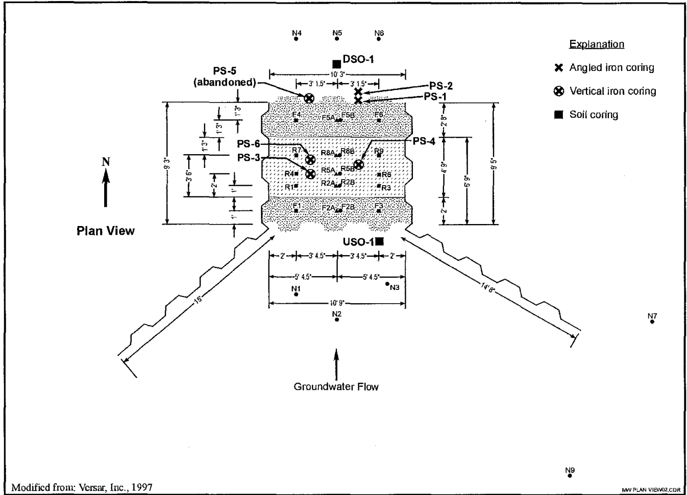
Figure 5-9. Sampling well locations in the PRB and vicinity at former Lowry AFB.
