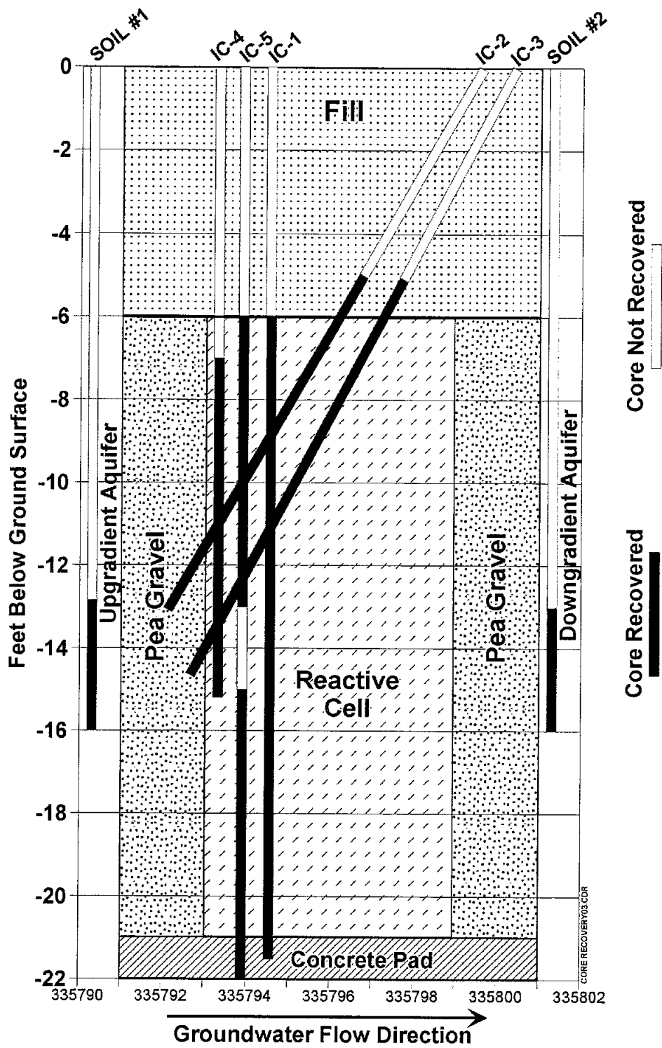
Figure 4-2. Coring locations in former NAS Moffett Field permeable reactive barrier (vertical profile).
