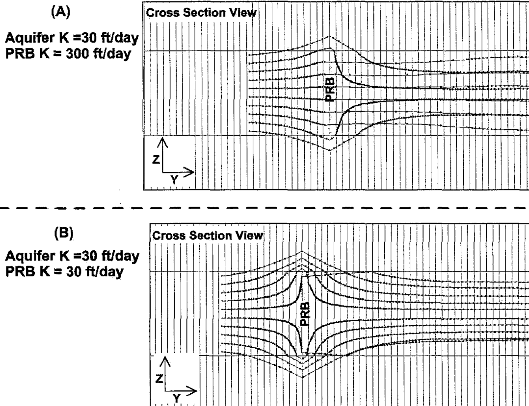
Figure 6-18. Particle tracking through a hanging wall PRB configuration. With PRB K set at 300 ft/day (A) only a small portion of groundwater flows under/over the wall, but with PRB K set at 30 ft/day (B) a large proportion of groundwater flows under/over the wall.
