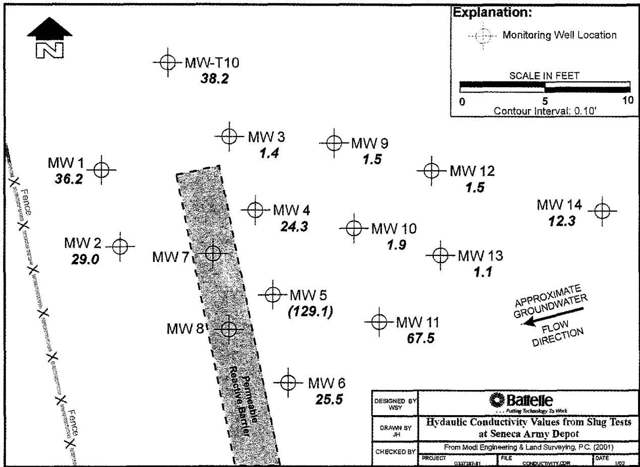
Figure 3-4. Hydraulic conductivity values (ft/d) from slug tests at the Seneca Army Depot PRB showing variations in hydraulic conductivity at the site.
