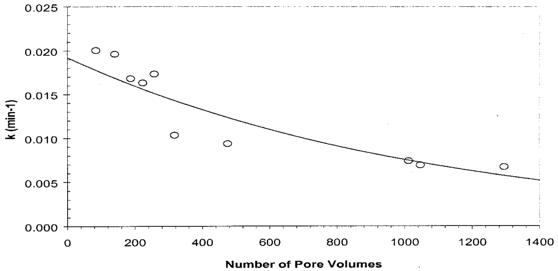
Figure 5-13. Plot of TCE degradation rates for former NAS Moffett Field column at different cumulative pore volumes.
