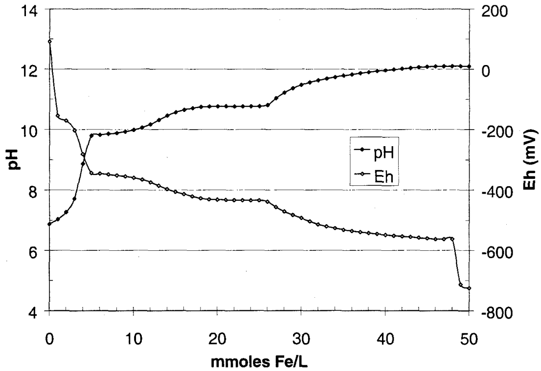
Figure 5-21. pH and Eh profile based on Case 1.
