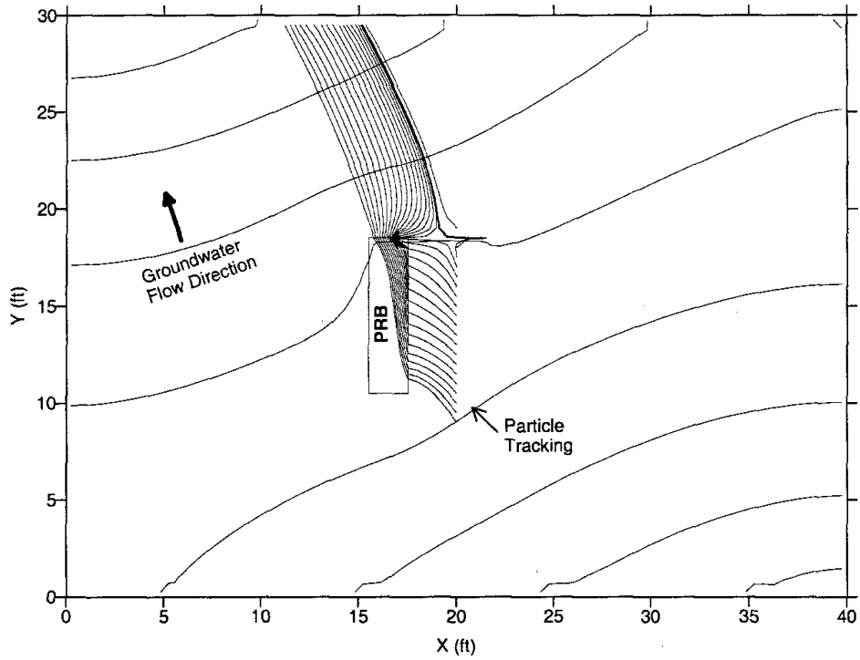
Figure 6-24. Model with downgradient drain and groundwater flow at an angle to the PRB.
