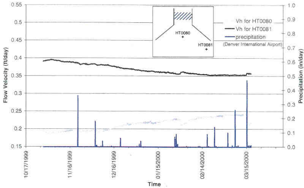
HydroTechnics Sensor Groundwater Direction Data at Lowry AFB
