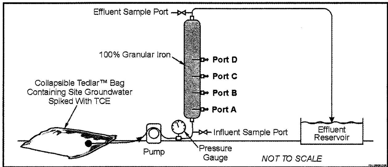
Figure 4-13. Schematic of accelerated column test setup
