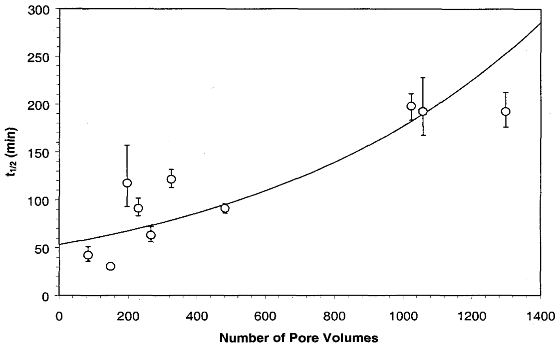
Figure 5-19. Plot of TCE half-lives for Lowry column at different cumulative pore volumes.
