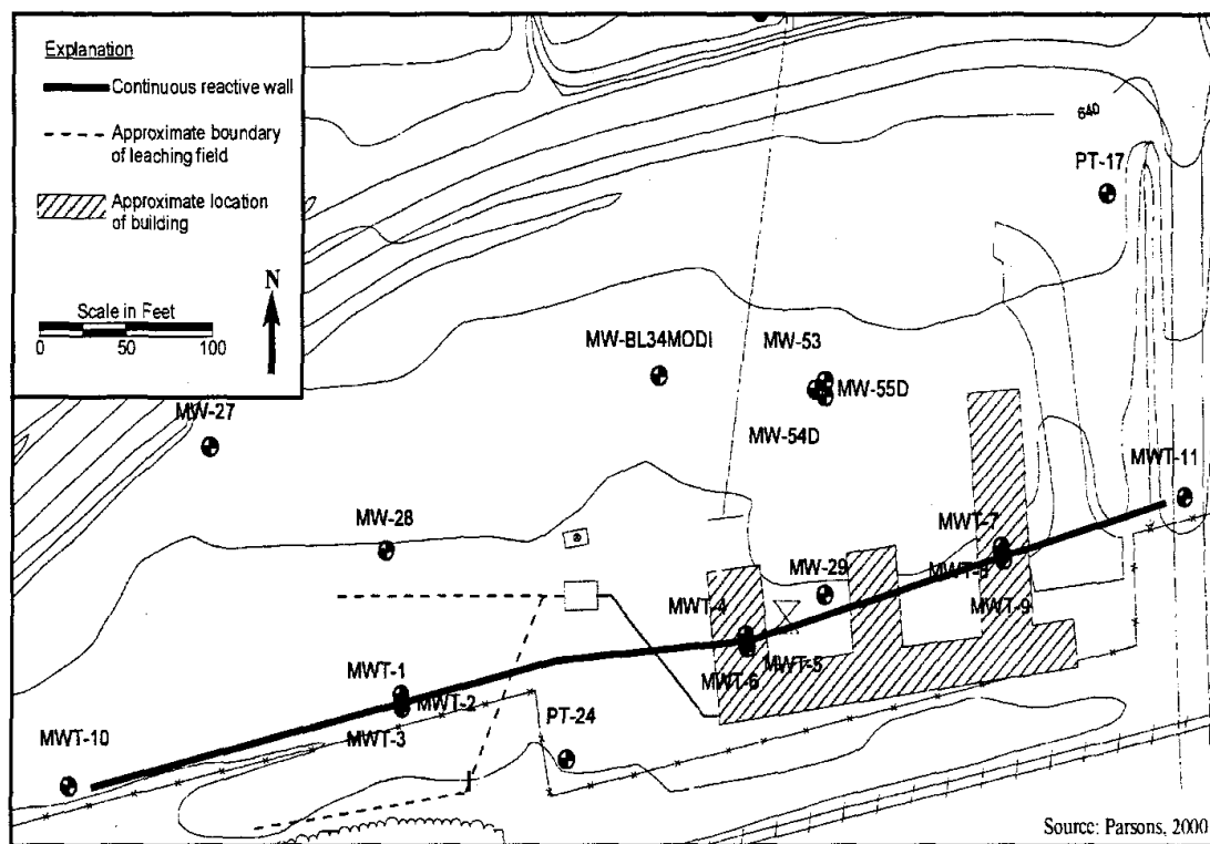
Figure 3-3. Plan view of PRB at Seneca Army Depot.
