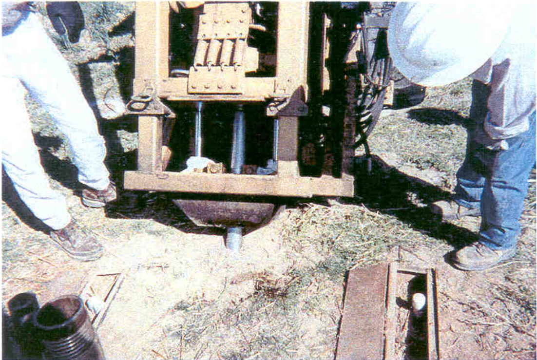
Figure 4-8. Close-up view of coring equipment.
