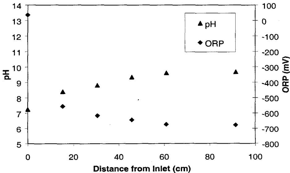
Figure 5-11. Plot showing stability of pH and ORP after 15 pore volumes of groundwater.
