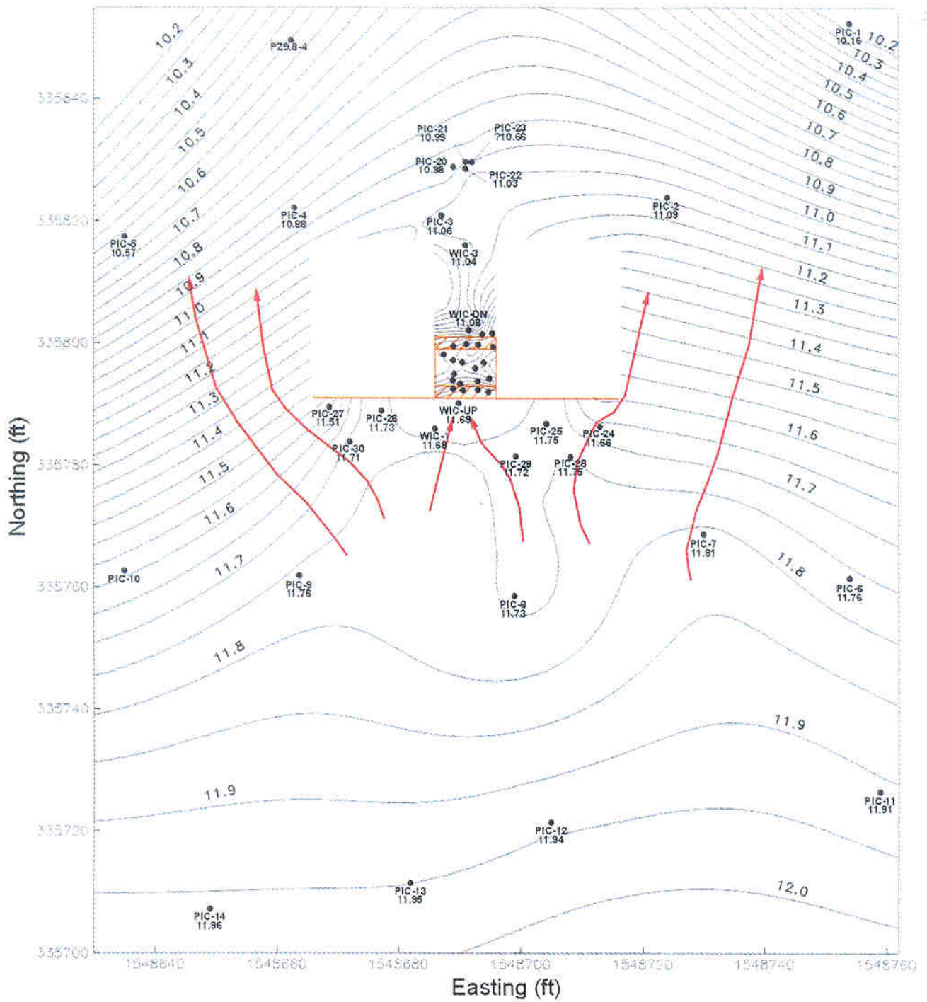
Figure 6-1. May 2001 water levels and flow patterns in the vicinity of former NAS Moffett Field PRB.
