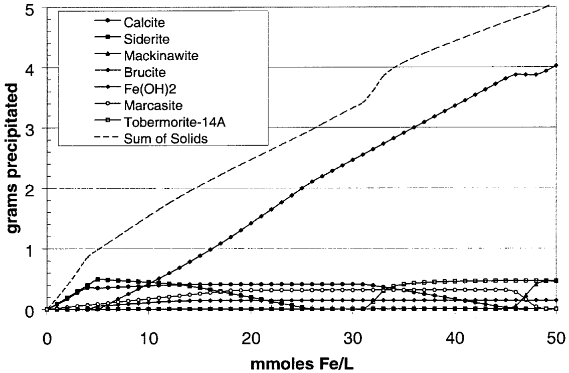
Figure 5-24. Masses of precipitates based on Case 1.
