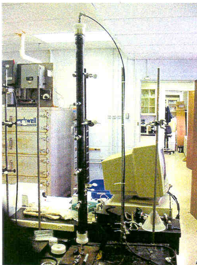
Figure 4-14. Picture of accelerated column tests.
