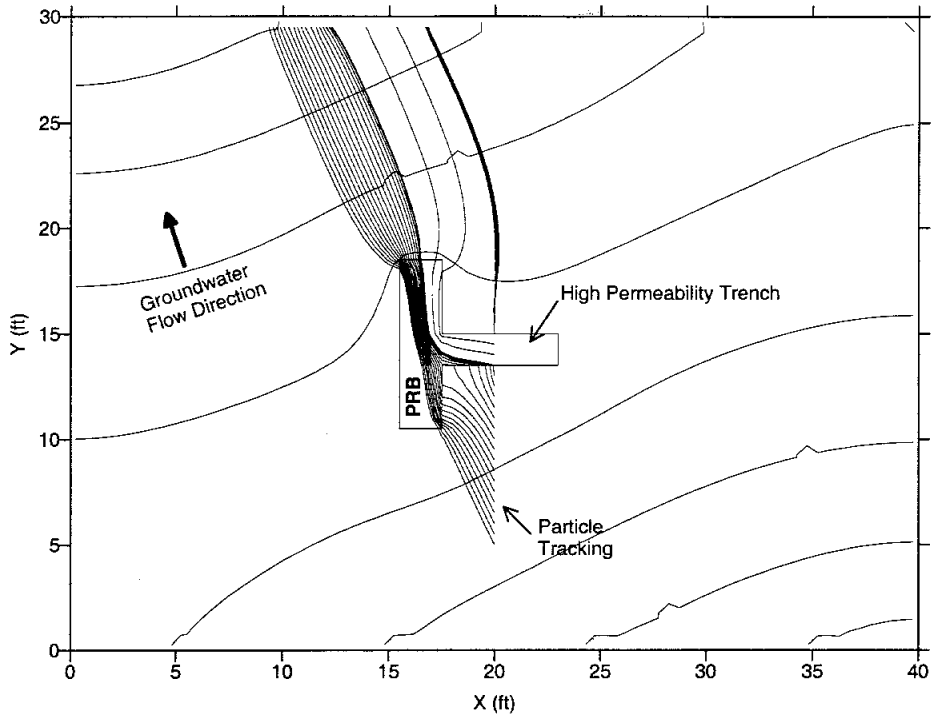
Figure 6-26. Model with upgradient trench and groundwater flow at angle to the PRB.
