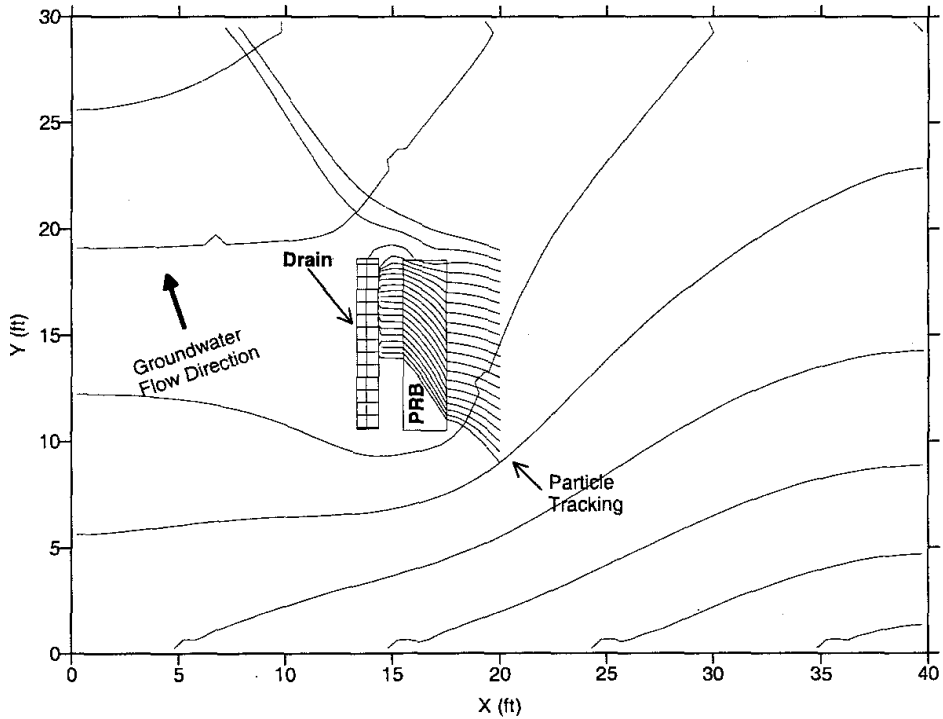
Figure 6-25. Model with downgradient barrier and groundwater flow at an angle to the PRB.
