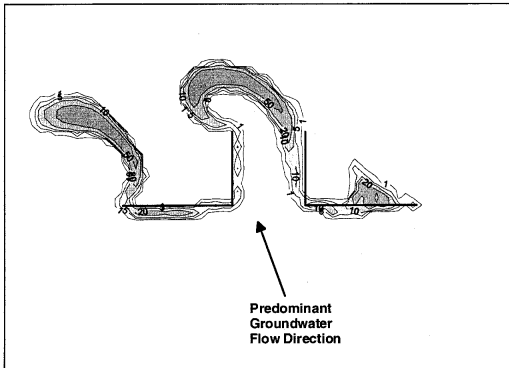
Figure 6-20. Transport modeling of plume migration for a PRB oriented at 70 degrees to the predominant direction of groundwater flow illustrating how contamination is diverted around portions of the PRB.
