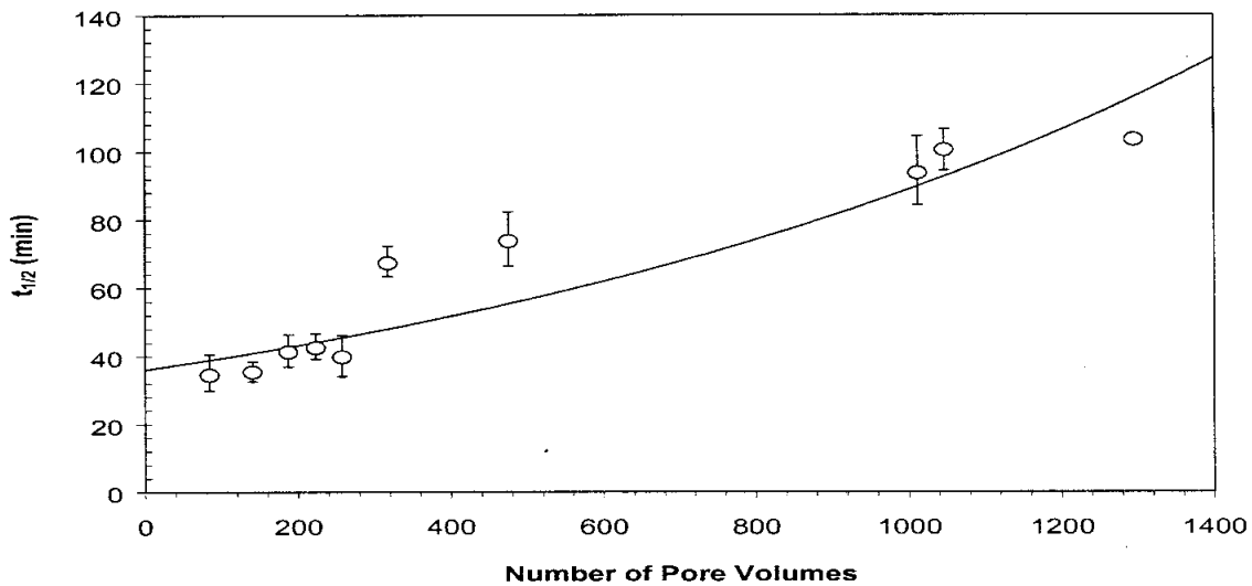
Figure 5-14. Plot of TCE half-lives for former NAS Moffett Field column at different cumulative pore volumes.
