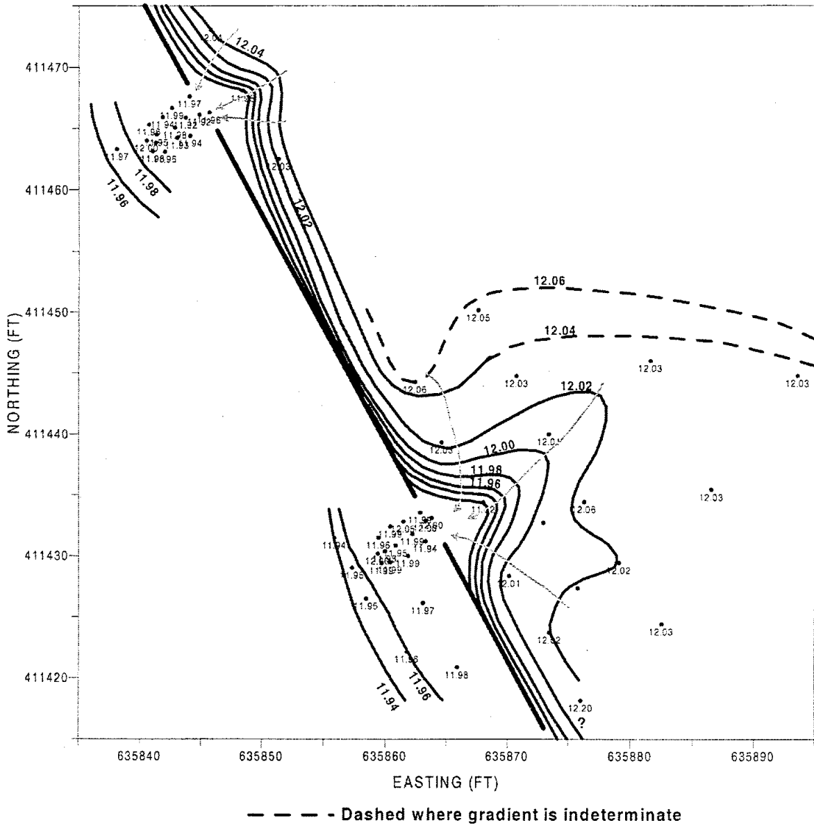
Water Levels (shallow) Feb 03, 1998 - Area 5 Funnel and Gate, Dover AFB
