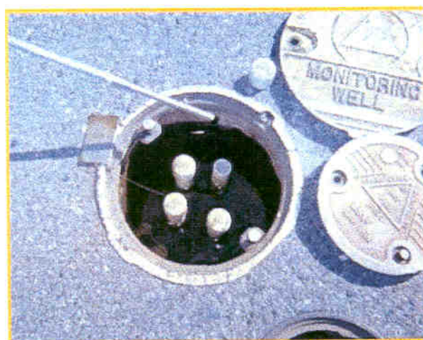
Figure 4-12. Silt sampler ready to be lowered into a monitoring well at former NAS Moffett Field.
