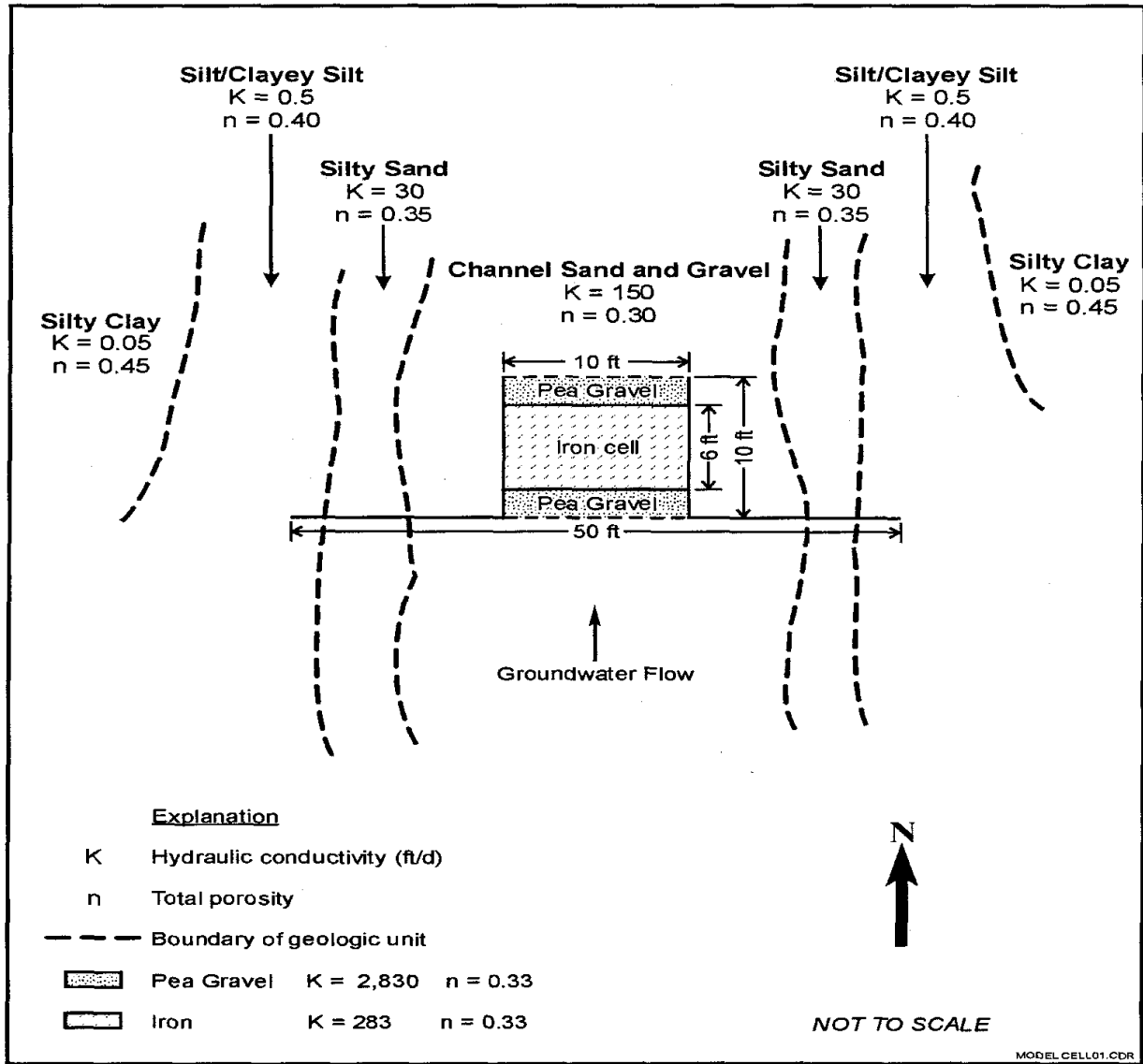
Figure 3-1. PRB at former NAS Moffett Field relative to lithologic variations in the surrounding aquifer.
