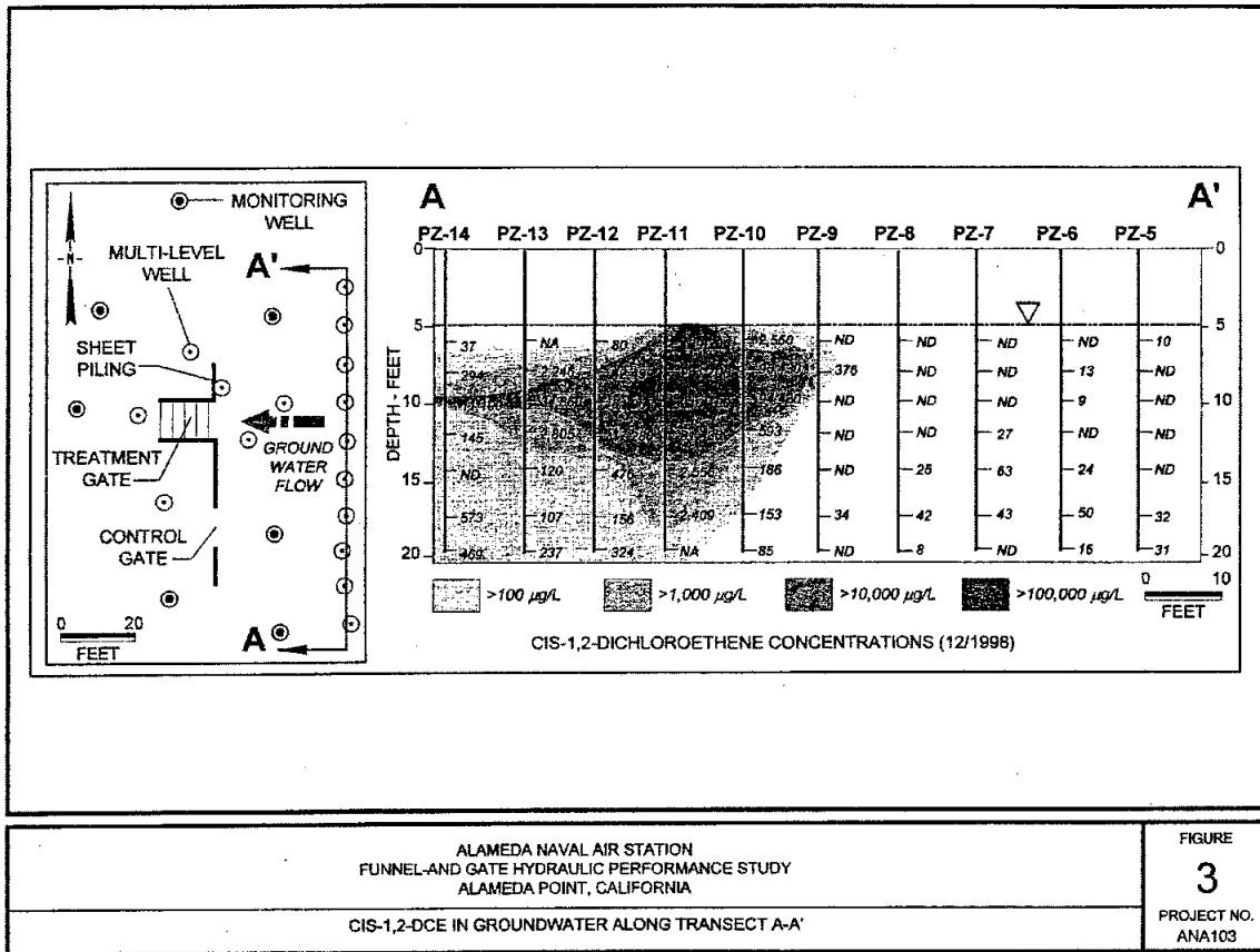
Figure 3-7. Schematic view of PRB and upgradient contamination profile at former NAS Alameda site (Einarson et al., 2000).
