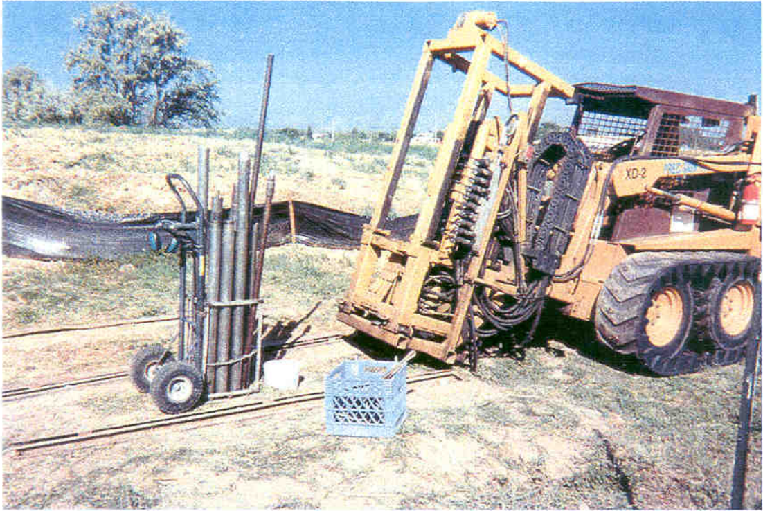
Figure 4-7. Coring rig.
