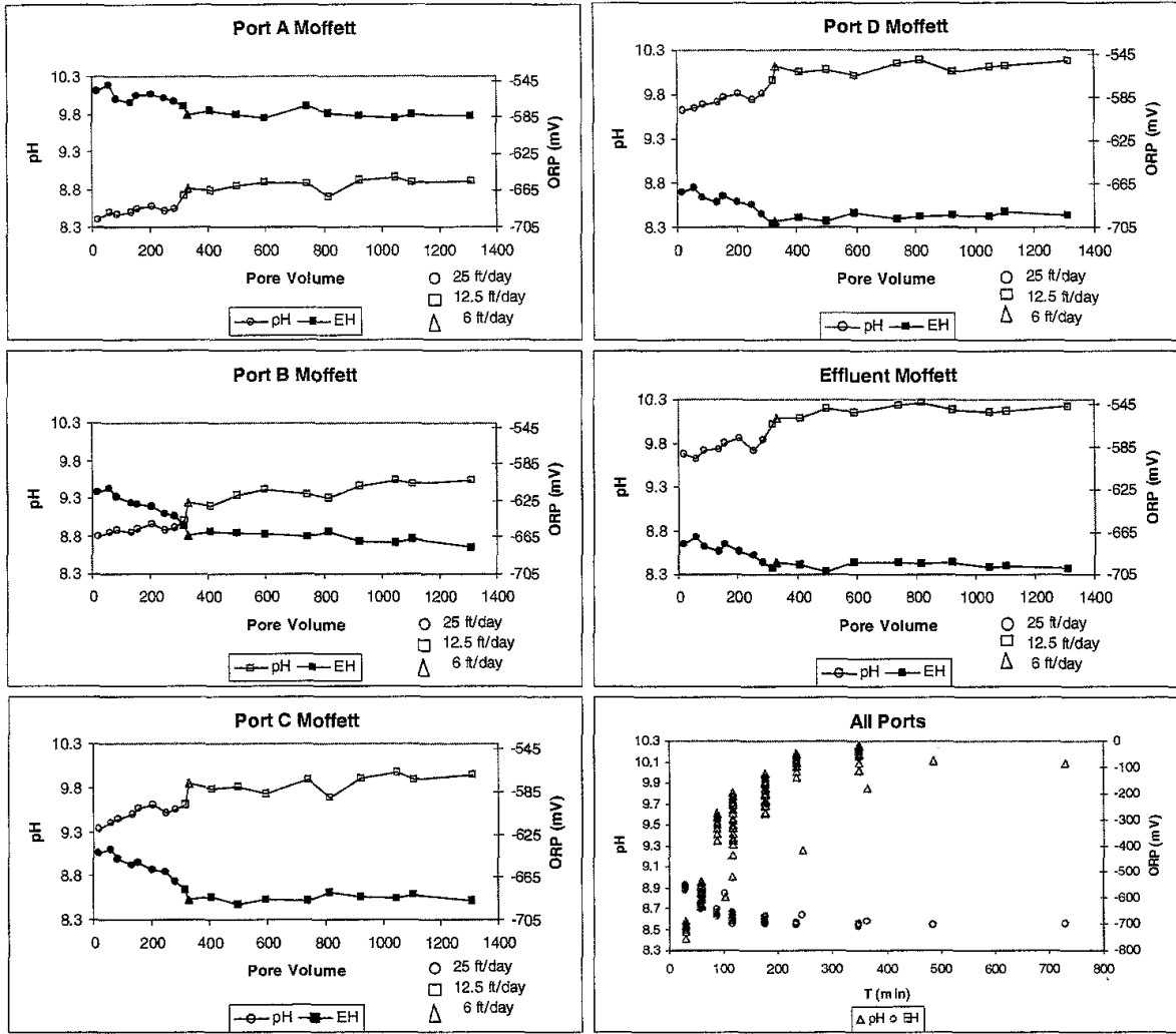
Figure 5-12. pH and ORP values in the former NAS Moffett Field column at different pore volumes (ages of iron).
