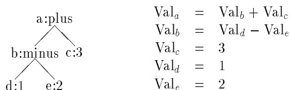
Figure 4.1: Tree and corresponding set of attribute equations for calculator example
