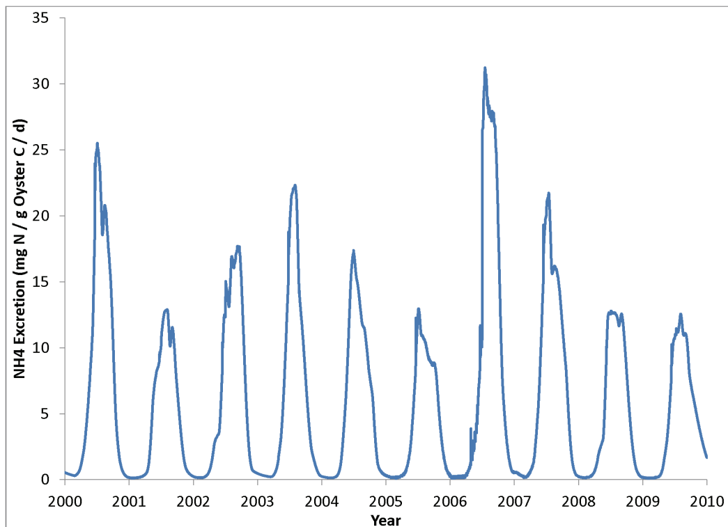
Figure 32. Computed specific ammonium excretion rate, averaged over all individuals.
