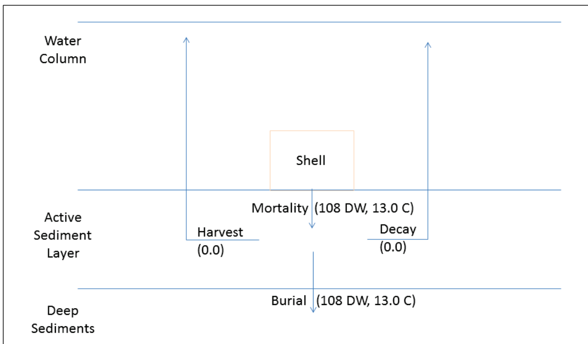
Figure 41. Computed shell benefits (dry weight shell and associated carbon) in the Great Wicomico. All values are annual averages in metric tons.
