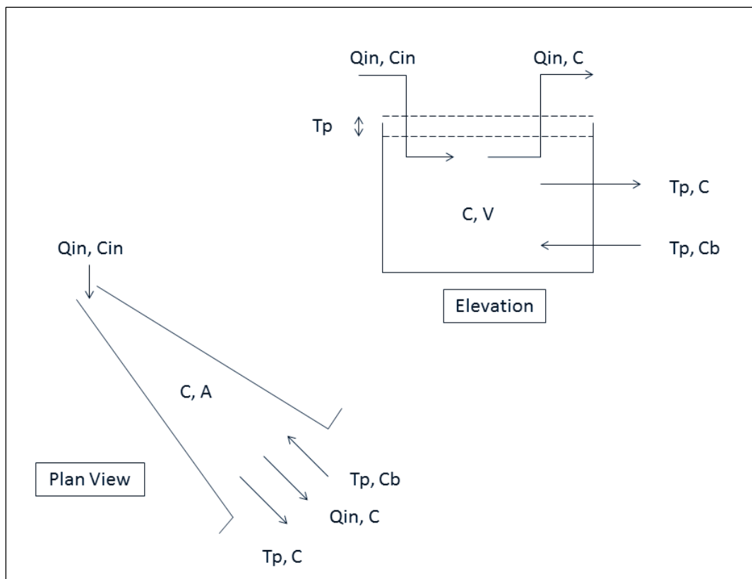
Figure 6. Tidal Prism Model Schematic. The system has volume V , surface area A , and concentration C . The tidal prism, T_p , is the product of the tide range and surface area. Runoff, Q_{in} , enters from the watershed carrying concentration C_{in} . Concentration C_b prevails outside the mouth.
