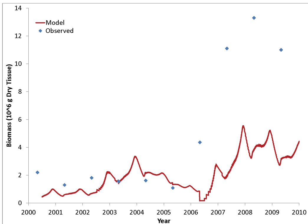
Figure 24. Computed and observed (Southworth et al. 2010) total biomass of oyster dry tissue.
