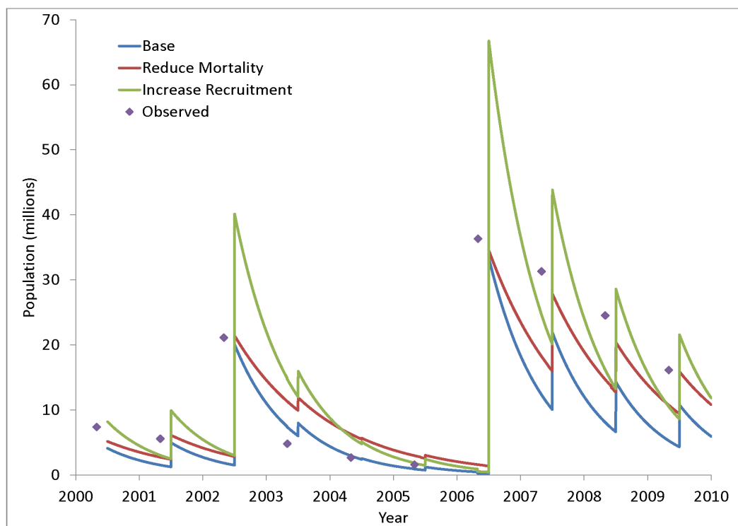
Figure 25. Sensitivity of computed and observed population to recruitment and mortality rates. Computations based on reduced mortality and increased recruitment are compared to the base computation and to observations.
