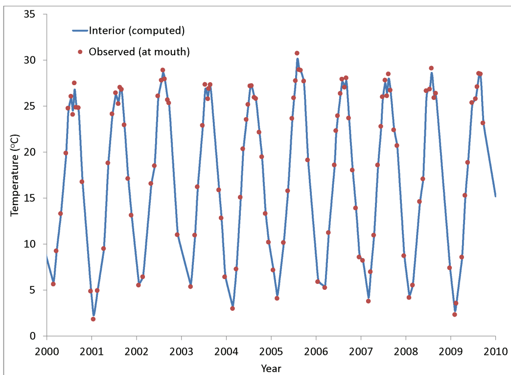
Figure 13. Temperature observed at the mouth of the Great Wicomico and computed in the interior.
