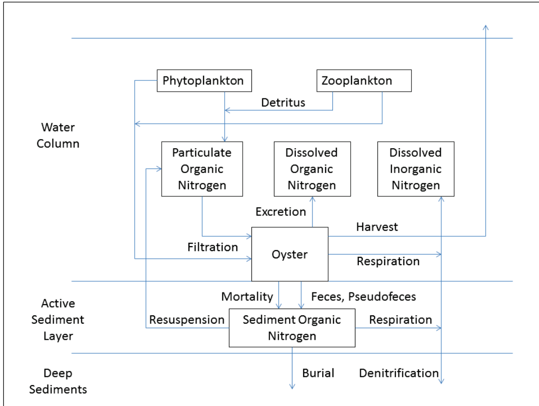
Figure 8. The model nitrogen cycle including oysters. The quantifiable benefits include nitrogen removal via fisheries harvest, nitrogen removal through burial to deep, inactive sediments, and nitrogen removal via denitrification.
