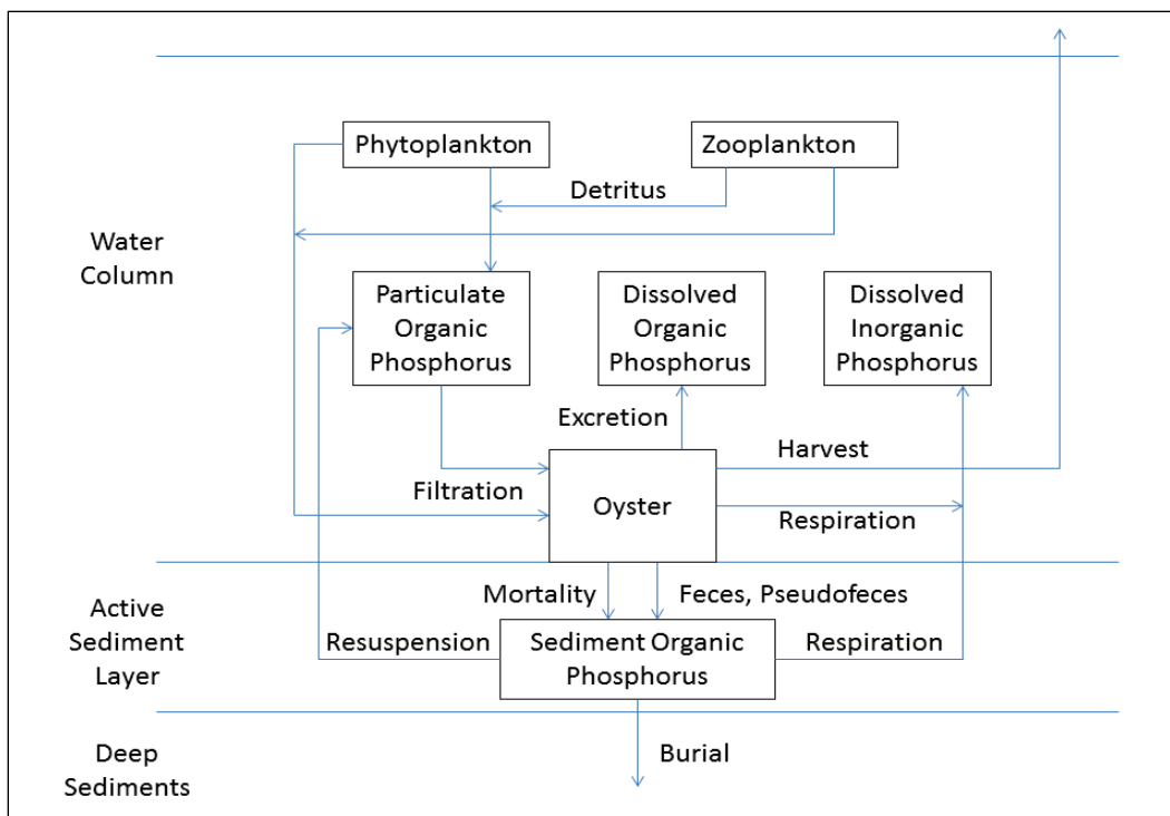
Figure 9. The model phosphorus cycle including oysters. The primary benefits include phosphorus removal via fisheries harvest and phosphorus removal via burial to deep, inactive sediments.
