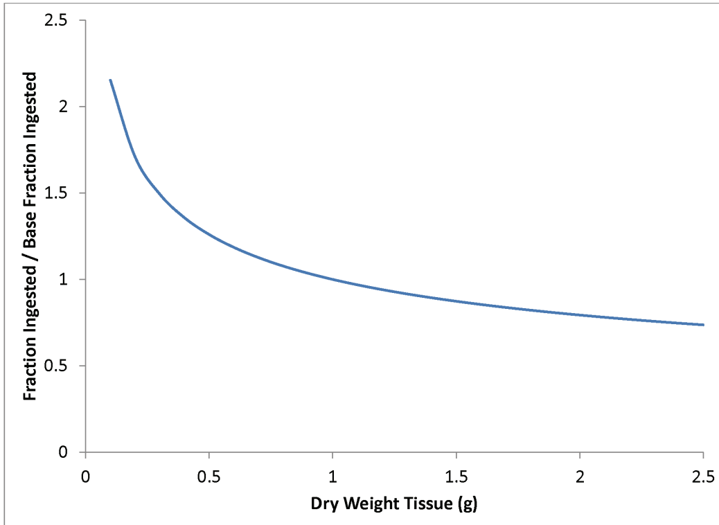
Figure 4. The effect of individual size on ingested fraction. The effect is shown as a ratio applied to a base rate calculated for an individual of 1 gm dry weight tissue with ing\_exp = -0.333 . As an individual increases in size, the ingested fraction diminishes.
