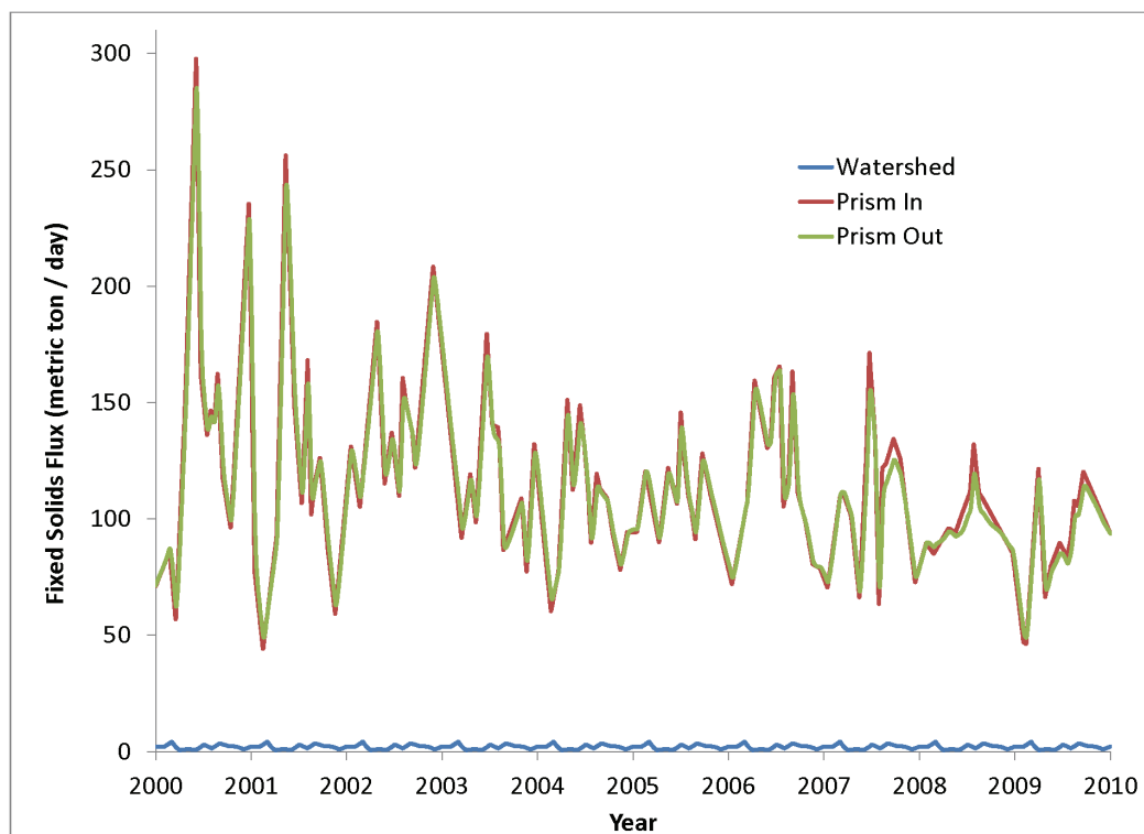
Figure 36. Computed fixed (inorganic) solids fluxes through the Great Wicomico.
