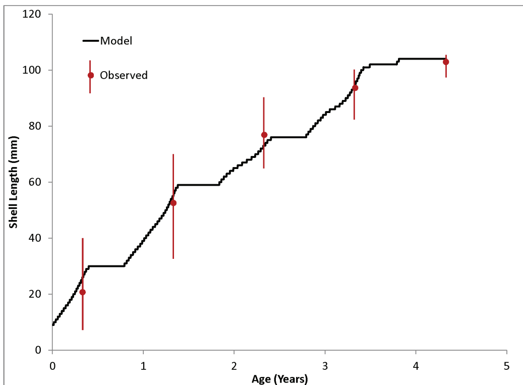
Figure 18. Computed and observed (Southworth et al. 2010) “age at length” relationships.
