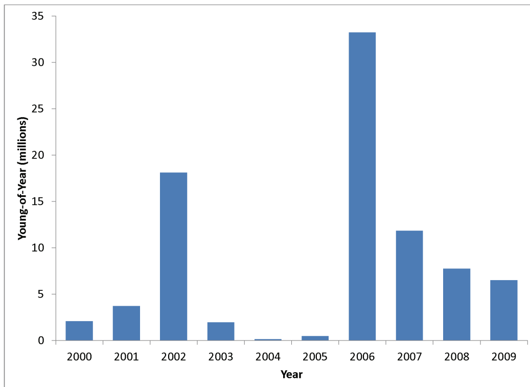
Figure 22. Observed (Southworth et al. 2010) “young-of-year.”
