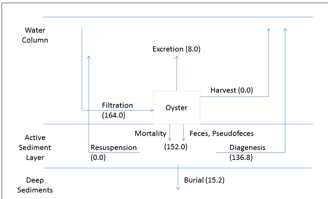
Figure 37. Computed carbon fluxes and benefits in the Great Wicomico. All values are annual averages in metric tons.
