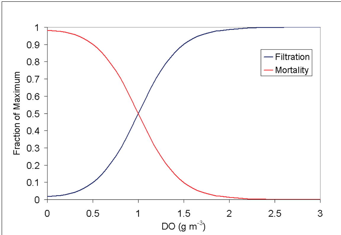
Figure 2. Modeled effect of dissolved oxygen on filtration and suffocation (mortality) rates.
