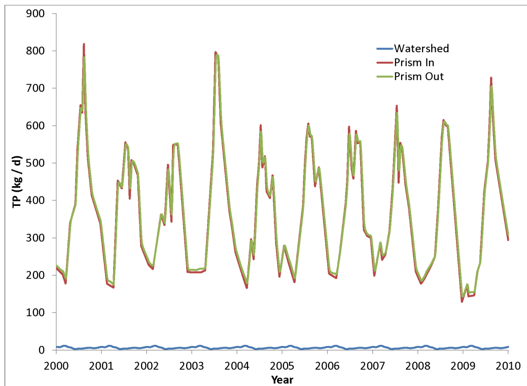
Figure 35. Computed total phosphorus fluxes through the Great Wicomico.
