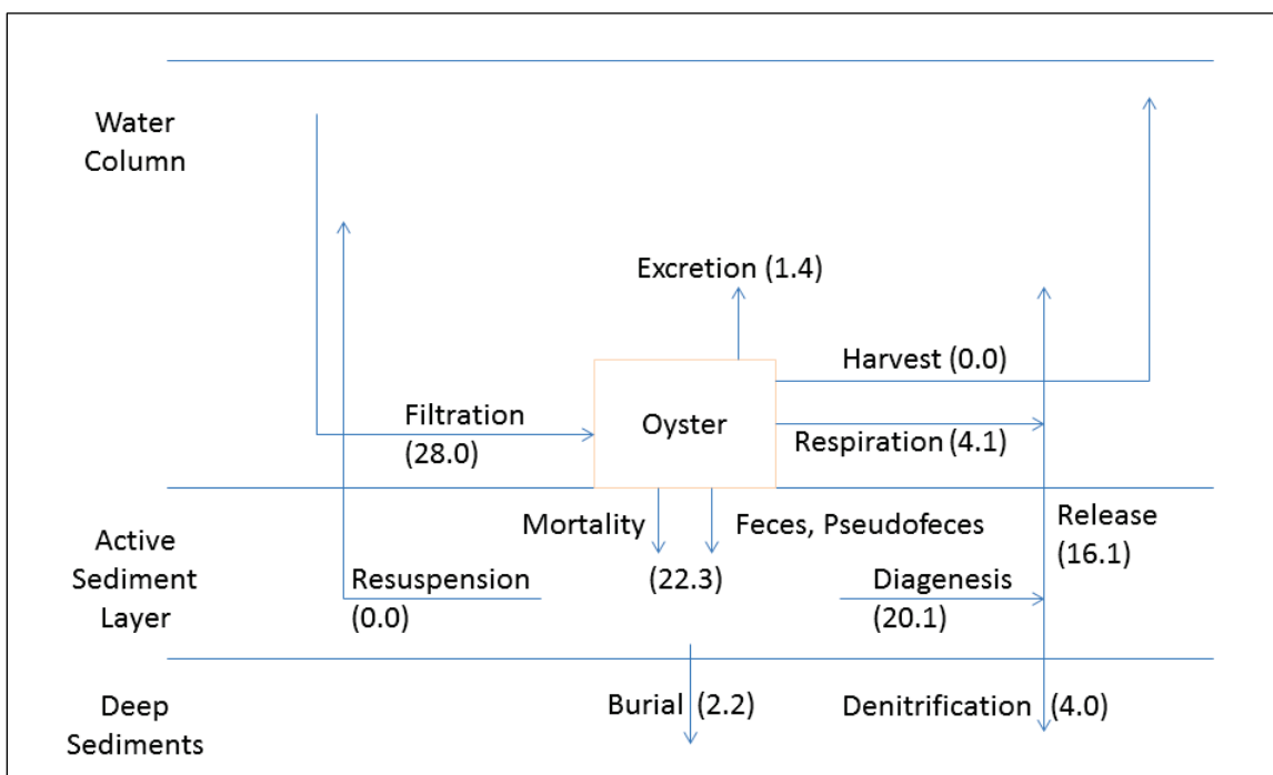
Figure 38. Computed nitrogen fluxes and benefits in the Great Wicomico. All values are annual averages in metric tons.
