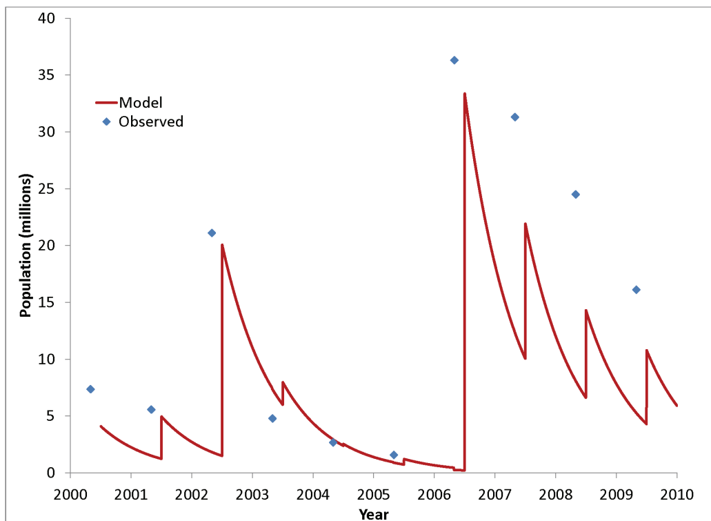
Figure 20. Computed and observed (Southworth et al. 2010) oyster population.
