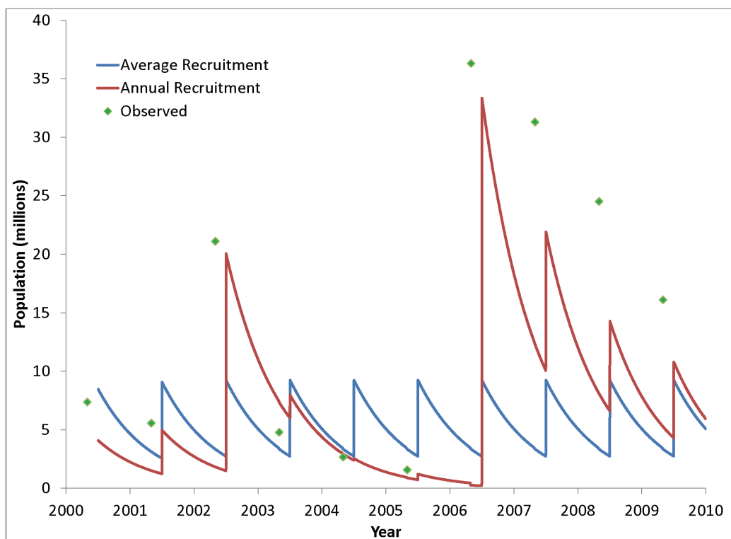
Figure 23. Sensitivity of computed population as compared to recruitment rate. Two computations are shown: one based on observed recruitment in individual years, the other based on recruitment rate averaged over all years.
