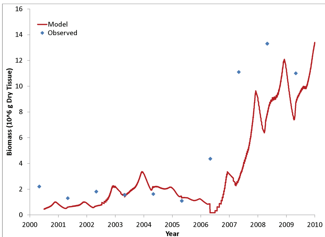
Figure 28. Total biomass computed on the basis of two mortality rates; 1.2 yr -1 for 2000 – 2005 and 0.77 yr -1 for 2006 – 2010.
