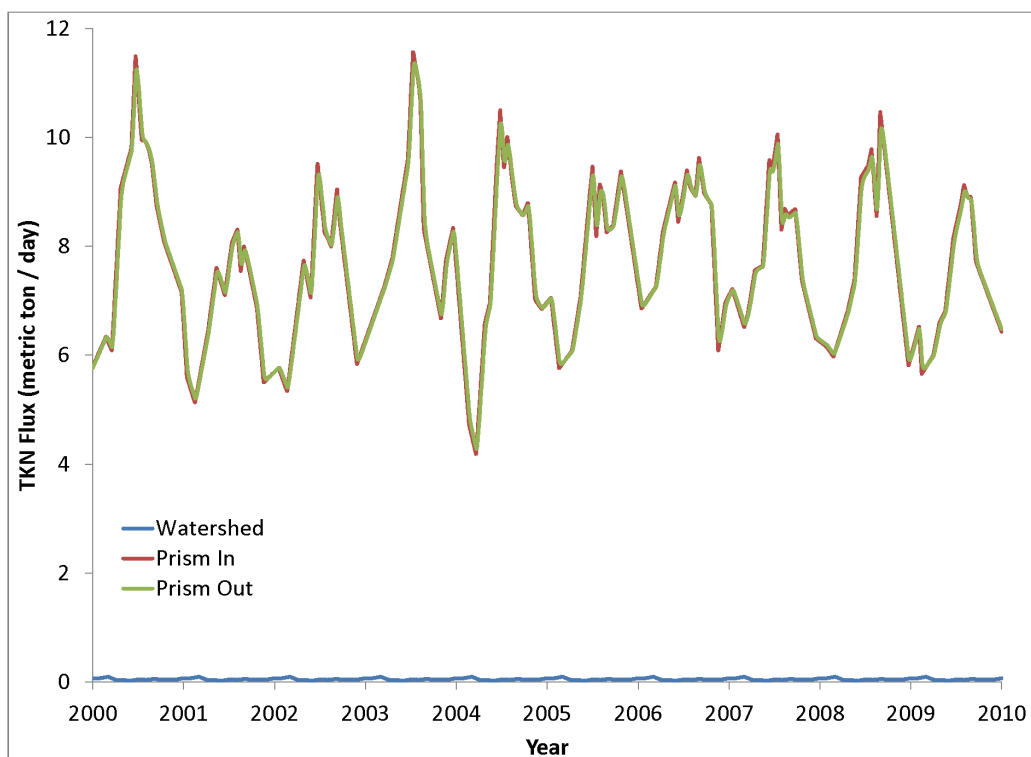
Figure 34. Computed TKN fluxes through the Great Wicomico.
