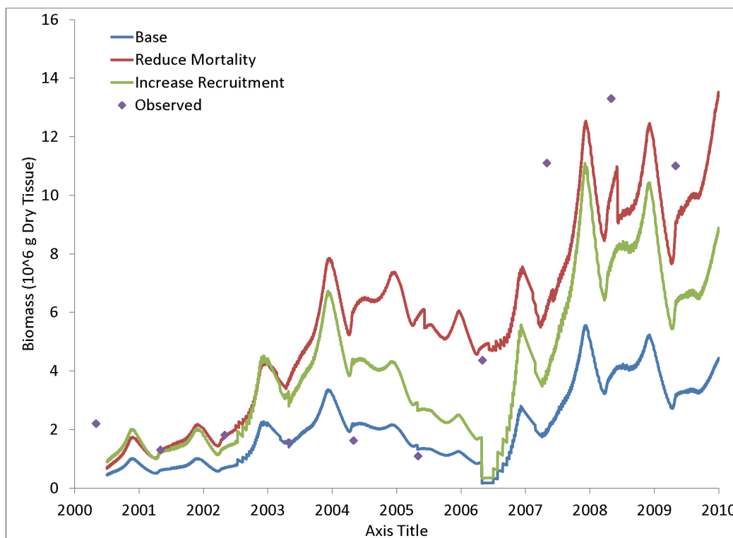
Figure 26 Sensitivity of computed total biomass to recruitment and mortality rates. Computations based on reduced mortality and increased recruitment are compared to the base computation and to observations.
