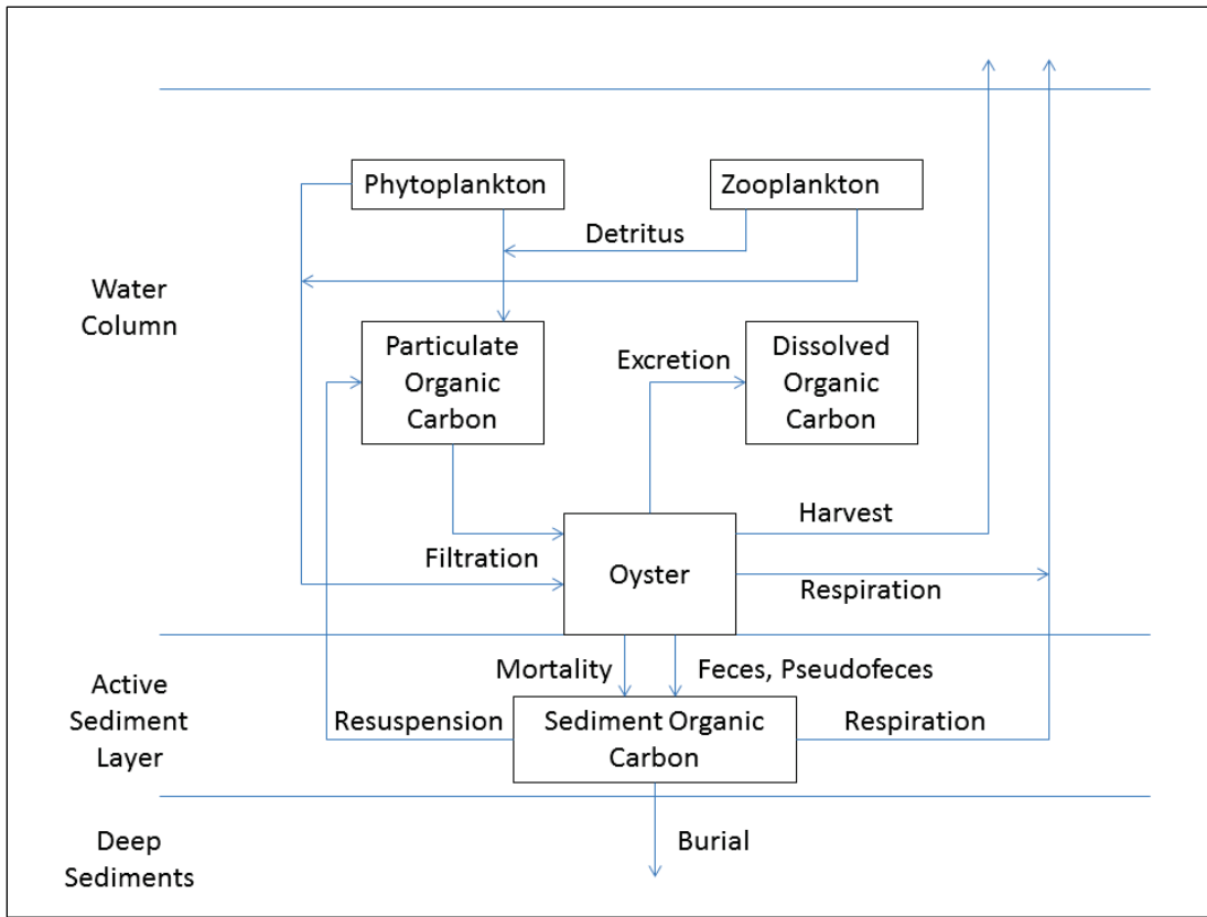
Figure 7. The model carbon cycle including oysters. The quantifiable benefits include carbon removal via fisheries harvest and carbon removal via burial to deep, inactive sediments.
