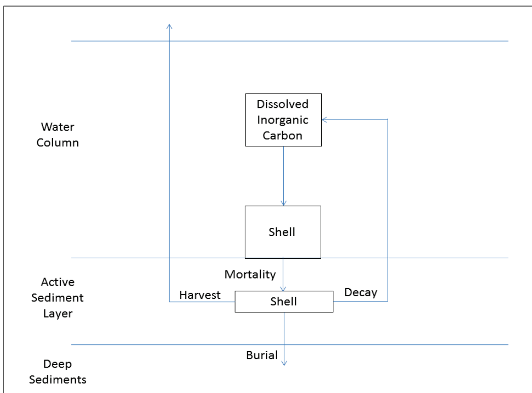
Figure 10. A simplified representation of processes affecting oyster shell in the water column and bottom sediments. Quantifiable benefits include shell accumulation in situ and shell collected as a by-product of fisheries harvest.
