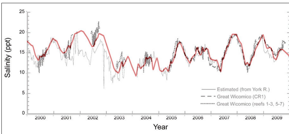
Figure 17. Computed salinity in the Great Wicomico (red) superimposed on values reported by Southworth et al. (2010).
