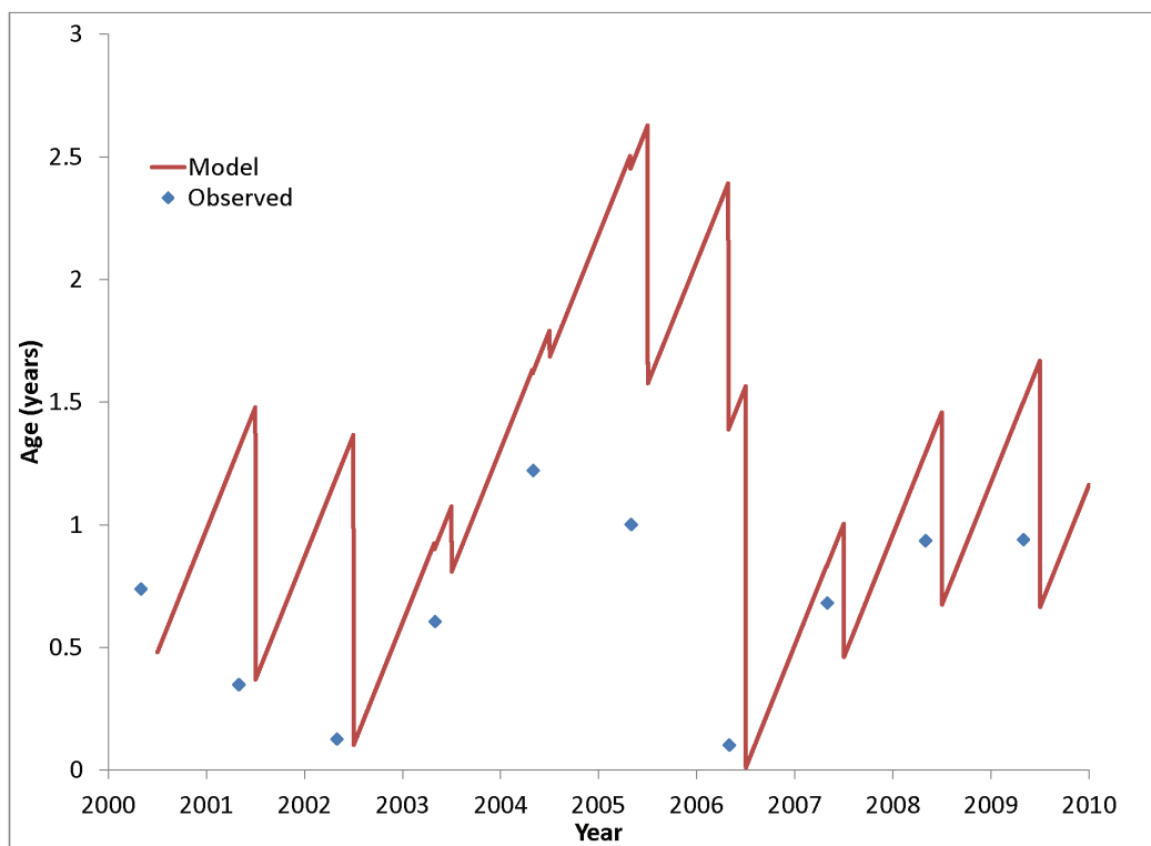
Figure 21. Computed and observed (Southworth et al. 2010) average age of oyster population.
