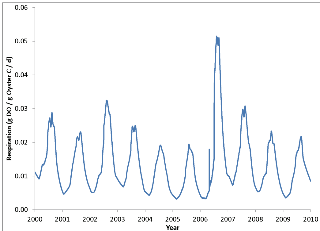
Figure 31. Computed specific respiration rate, averaged over all individuals.
