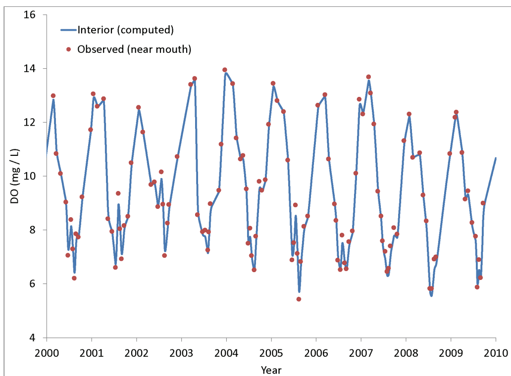
Figure 15. Dissolved oxygen observed at the mouth of the Great Wicomico and computed in the interior.
