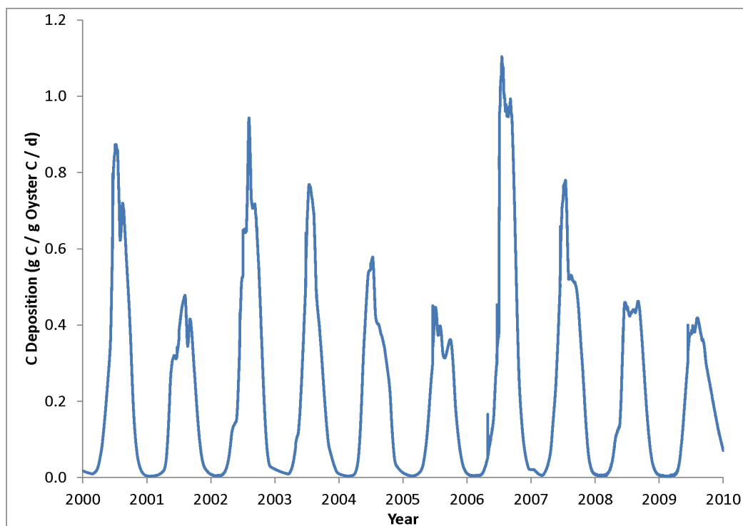
Figure 33. Computed specific carbon deposition rate, averaged over all individuals.
