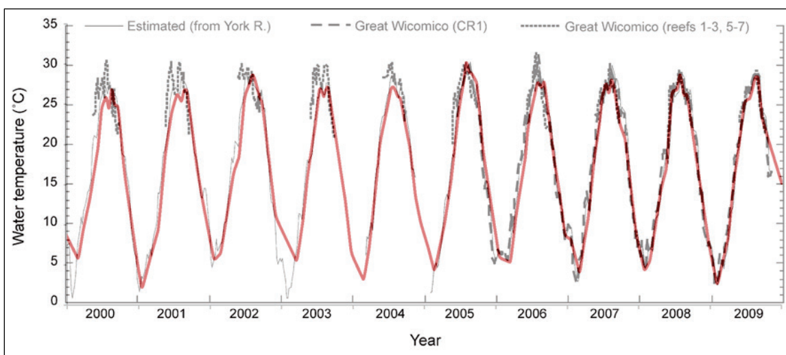
Figure 16. Computed temperature in the Great Wicomico (red) superimposed on values reported by Southworth et al. (2010).
