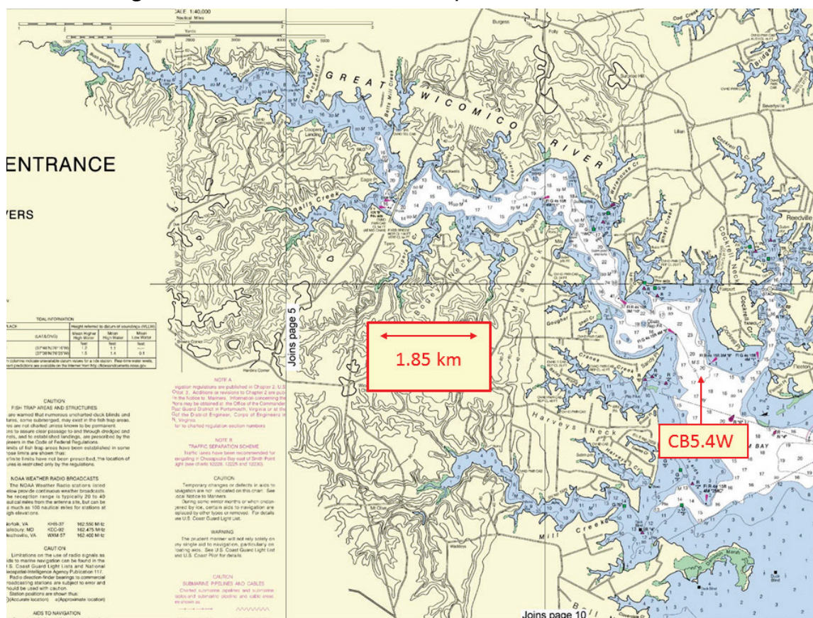
Figure 12. The Great Wicomico River. Sample station CB5.4W is indicated.
