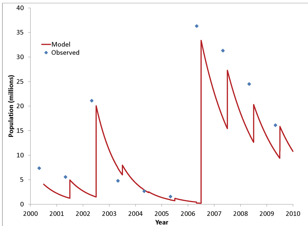
Figure 27. Population computed on the basis of two mortality rates, 1.2 yr -1 for 2000 – 2005 and 0.77 yr -1 for 2006 – 2010.
