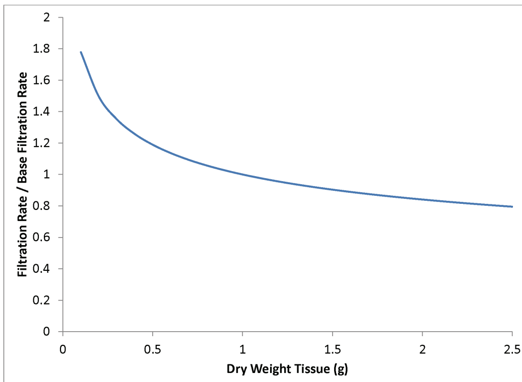
Figure 3. The effect of individual size on specific filtration rate. The effect is shown as a ratio applied to a base rate calculated for an individual of 1 gm dry weight tissue with \text{FRexp} = -0.25 . As an individual increases in size, the filtration rate diminishes. The same relationship applies to the effect of individual size on specific metabolic rate.
