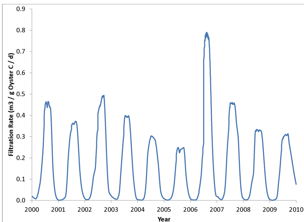
Figure 30. Computed specific filtration rate, averaged over all individuals.
