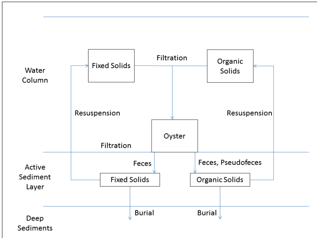
Figure 11. The modeled influence of oysters on fixed and volatile suspended solids. The primary benefits are burial of both forms to deep, inactive sediments.
