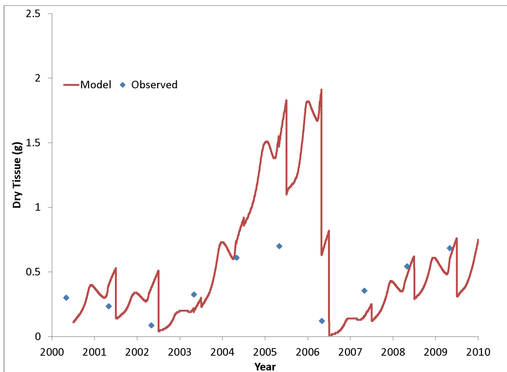
Figure 19. Computed and observed (Southworth et al. 2010) population-average individual dry tissue weight.
