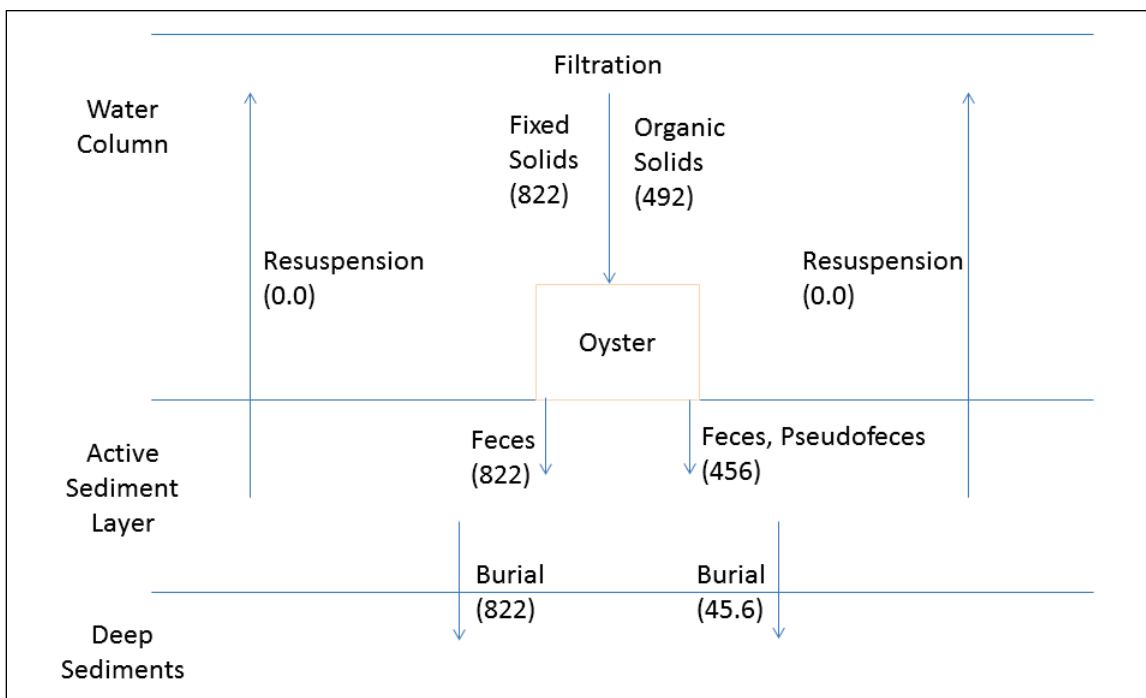
Figure 40. Computed solids fluxes and benefits in the Great Wicomico. All values are annual averages in metric tons.
