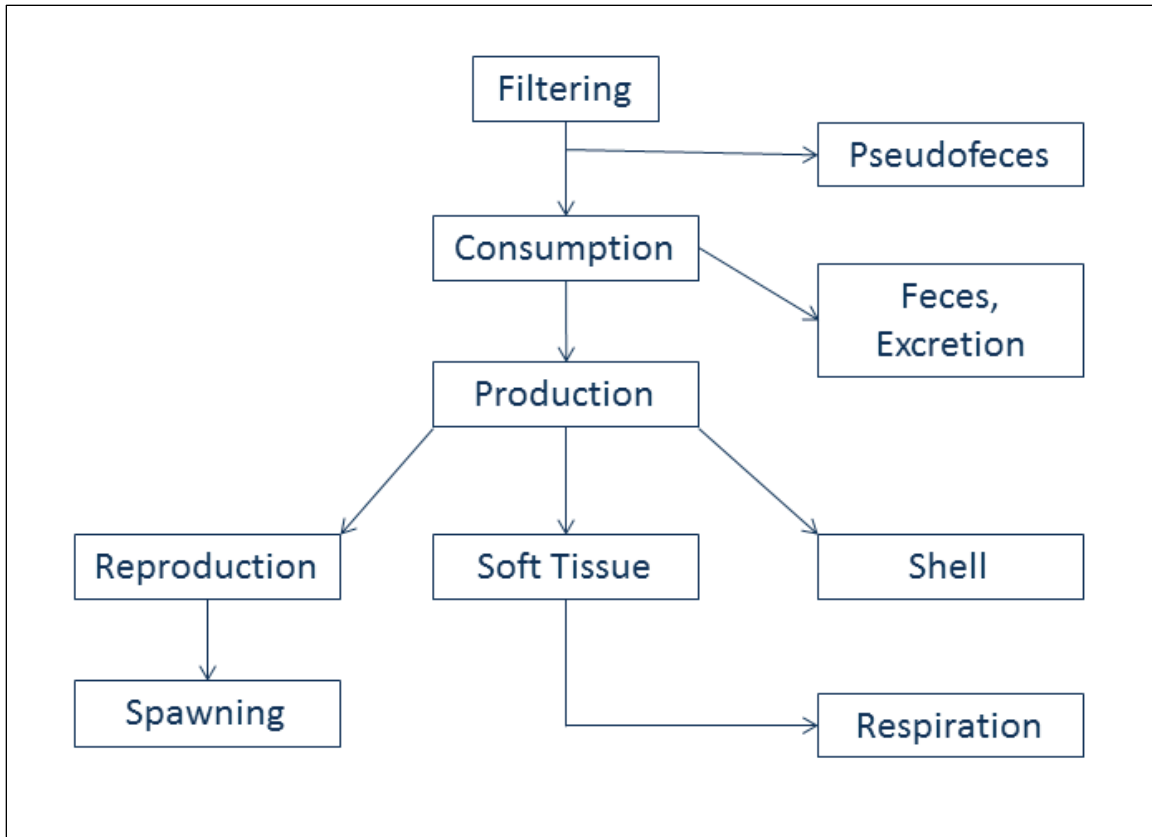
Figure 1. Energy flows in the bivalve energetics model.
