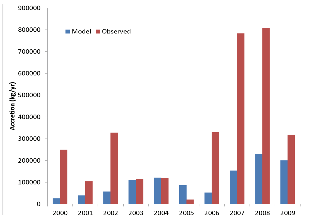
Figure 29. Computed and observed (Southworth et al. 2010) shell accretion rates.
