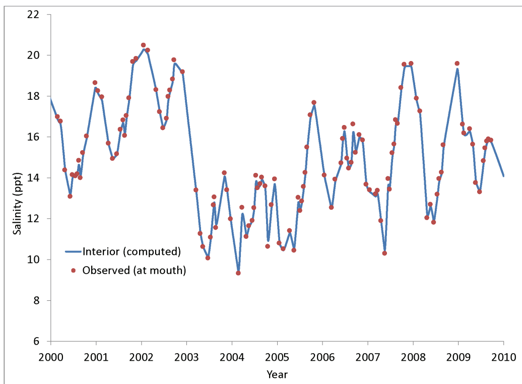
Figure 14. Salinity observed at the mouth of the Great Wicomico and computed in the interior.
