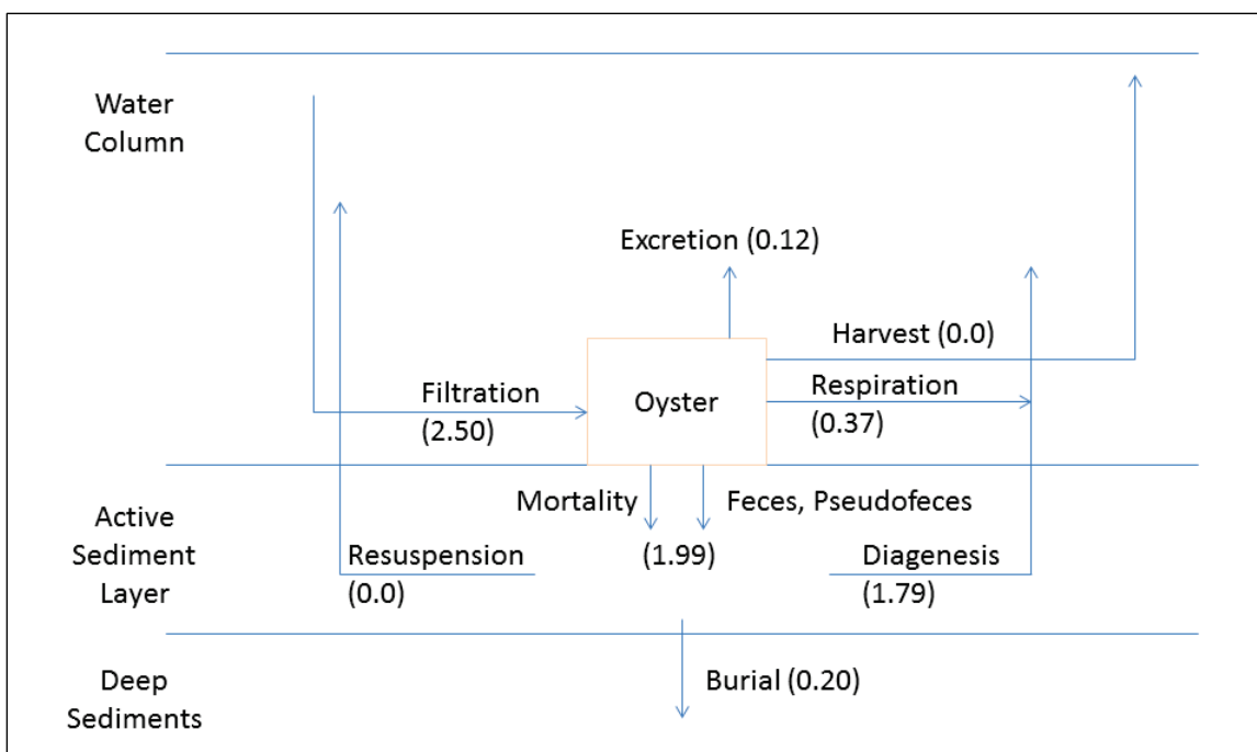
Figure 39. Computed phosphorus fluxes and benefits in the Great Wicomico. All values are annual averages in metric tons.
